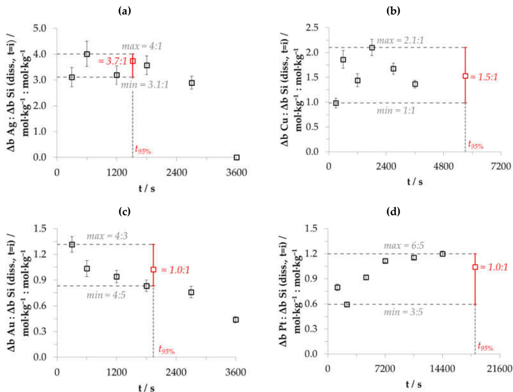
Figure 5. Stoichiometric ratios between the metal deposition \Delta b \text{ Me} ((a) Ag, (b) Cu, (c) Au and (d) Pt) and silicon dissolution \Delta b \text{ Si} as a function of time t ( \Delta b \text{ Me}:\Delta b \text{ Si} (\text{diss.}, t = i) ) based on the experiments of Figure 1 with an indication of the t_{95\%} -weighted stoichiometric ratios (red dots) and the corresponding minima and maxima (bars) denoted as ( \Delta b \text{ Me}:\Delta b \text{ Si} (\text{diss.}, t_{95\%}) ).
