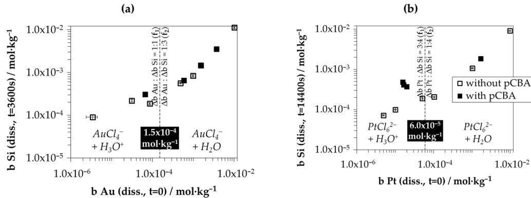
Figure 8. Molality of dissolved silicon in (a) gold deposition after t = 3600 \text{ s} ( b \text{ Si (diss., } t = 3600 \text{ s)} ) and (b) platinum deposition after t = 14,400 \text{ s} ( b \text{ Si (diss., } t = 14,400 \text{ s)} ) in relation to the initial metal ion molality ( b \text{ Au (diss., } t = 0) and b \text{ Pt (diss., } t = 0) ), respectively with and without the presence of para-chlorobenzoic acid (pCBA).
