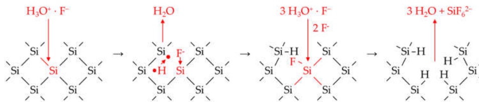
Figure 9. Proposed scheme of the reaction of the ion pair \text{H}_3\text{O}^+ \cdot \text{F}^- with silicon.
