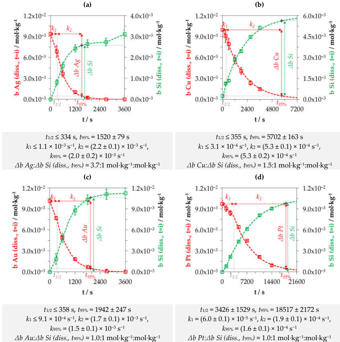
Figure 1. Dissolved (a) Ag, (b) Cu, (c) Au and (d) Pt species b \text{ Me (diss., } t = i) and (a–d) Si species b \text{ Si (diss., } t = i) at t = i ; the period of the metal deposition phases 1 ( t = 0 until t_{1/2} ) and 2 ( t_{1/2} until t_{95\%} ); the metal deposition rates k_1 and k_2 ; the t_{95\%} -weighted deposition rate k_{95\%} ; and the stoichiometric ratio of the change in molality of the dissolved metal ion \Delta b \text{ Me} in relation to the change in molality of the dissolved silicon species \Delta b \text{ Si} in the period of t = 0 until t_{95\%} ( \Delta b \text{ Me} : \Delta b \text{ Si (diss., } t_{95\%}) ).
