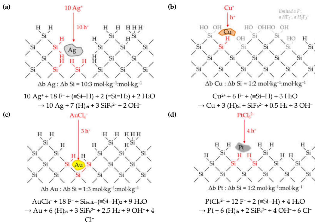
Figure 11. Reaction schemes of (a) silver, (b) copper, (c) gold and (d) platinum deposition on hydrogen-terminated silicon within section IV .
