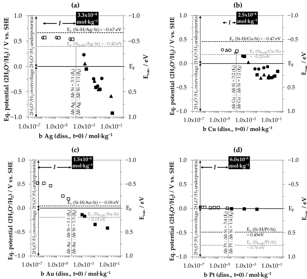
Figure 7. Equilibrium potentials of the 2\text{H}_3\text{O}^+/\text{H}_2 half-cells at the (a) Ag, (b) Cu, (c) Au or (d) Pt surfaces (bright metal state/colloidal metal solution [76]) in relation to the initial metal ion molalities ( b \text{ Me (diss., } t=0) ), the level of the Fermi energy E_F and levels of the valence bands of the bulk silicon ( E_v(\text{Si}_{\text{bulk}}/\text{Me-Si}) ) and that of the hydrogen-terminated silicon ( E_v(\text{Si-H}/\text{Me-Si}) ) at the metal–silicon contact. (Hollow symbols = oxonium ion reduction to molecular hydrogen possible, full symbols = no reaction).
