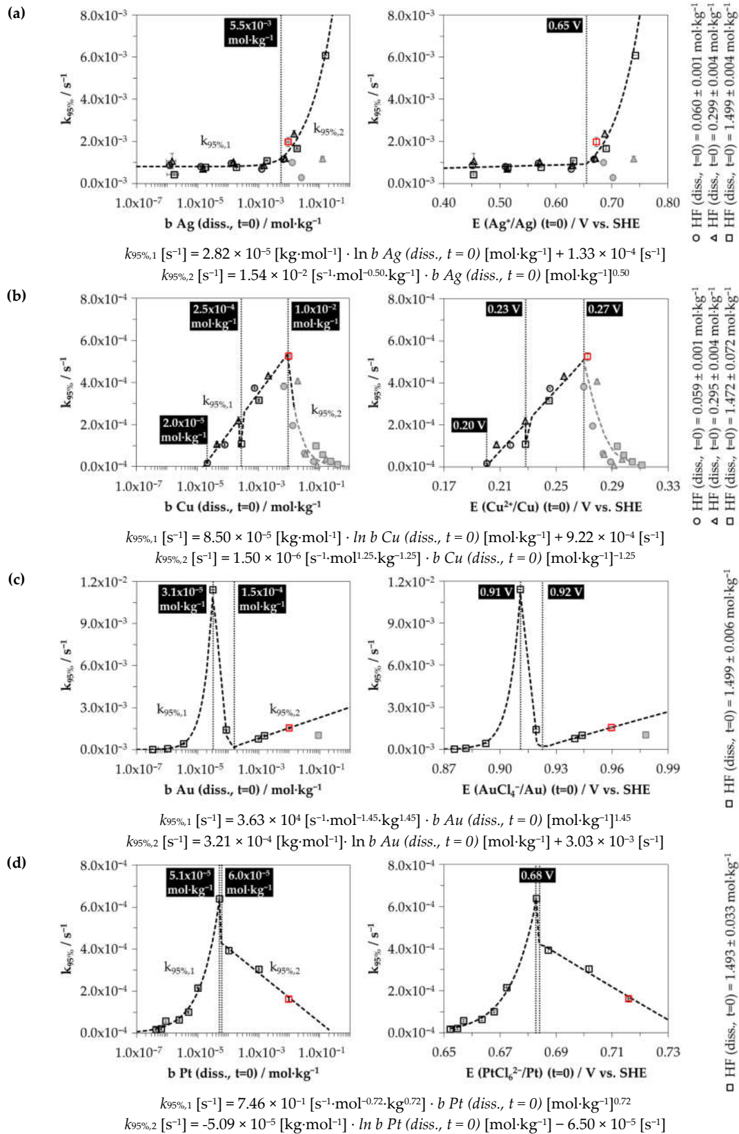
Figure 2. Metal deposition rates k_{95\%} ( k_{95\%,1} and k_{95\%,2} ) of the (a) Ag, (b) Cu, (c) Au and (d) Pt depositions in relation to the initial metal ion molality ( b \text{ Me (} t=0 \text{)} , \text{Me} = \text{Ag, Cu, Au, Pt} ) or to the redox potential of the \text{Me}^{2+}/\text{Me} half-cells E (\text{Me}^{2+}/\text{Me}) . Red dots = examples from Figure 1, grey dots = findings with delayed silicon dissolution.
