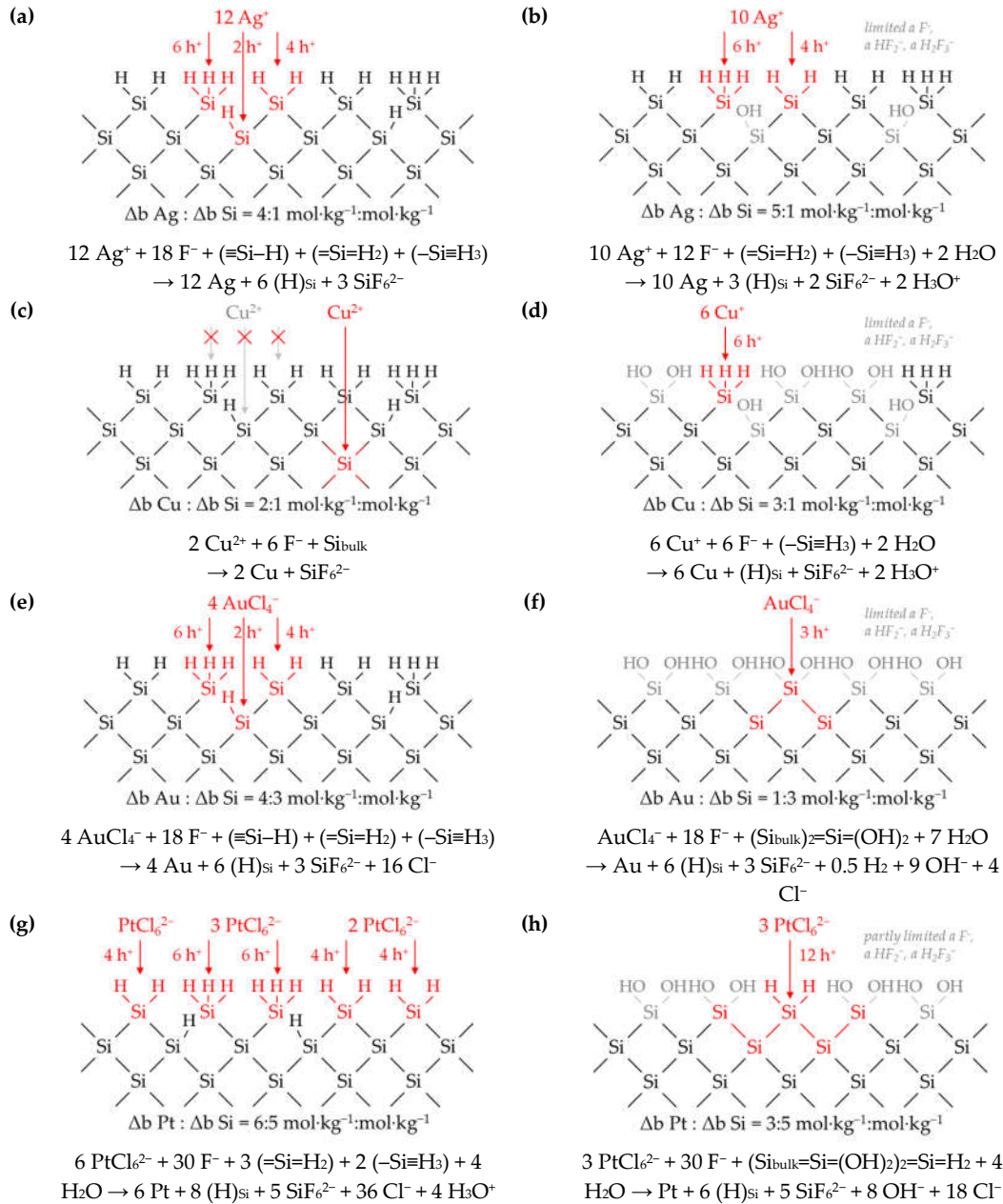
Figure 10. Reaction schemes of (a,b) silver, (c,d) copper, (e,f) gold and (g,h) platinum deposition on hydrogen-terminated silicon within section III.
