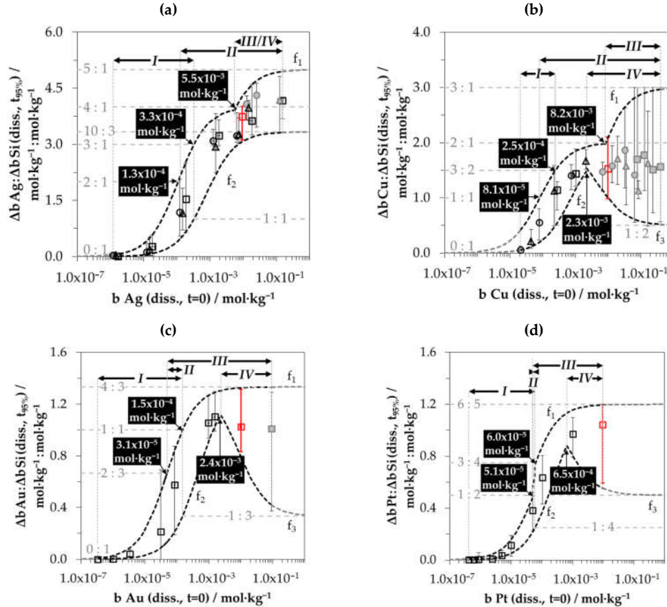
Figure 6. Stoichiometric ratios between the metal deposition \Delta b Me ((a) Ag, (b) Cu, (c) Au and (d) Pt) and silicon dissolution \Delta b Si until t_{95\%} ( \Delta b Me : \Delta b Si (diss., t_{95\%}) ), in relation to the initial metal ion molality ( b Me (diss., t = 0) ), are indicated as points for the t_{95\%} -weighted values and as bars for the corresponding minima and maxima with delimitation by sigmoid functions f_1 , f_2 and f_3 and classification of the underlying processes in sections I, II, III and IV (red dots = examples from Figure 1, grey dots = findings with limited silicon dissolution).
