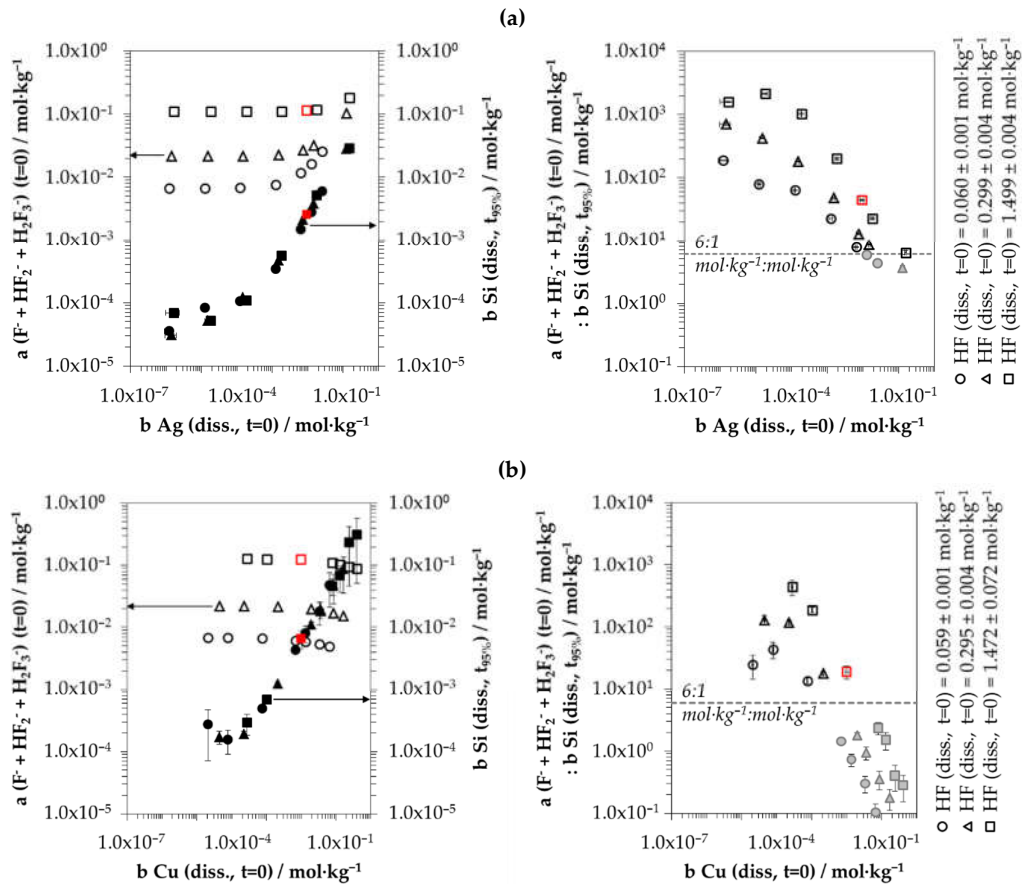
Figure 4. Left: Sum of the initial activities of the anionic HF dissociation products \text{F}^- , \text{HF}_2^- and \text{H}_2\text{F}_3^- ( a(\text{F}^- + \text{HF}_2^- + \text{H}_2\text{F}_3^-)(t=0) ) and molality of the dissolved silicon at t_{95\%} ( b \text{ Si (diss., } t_{95\%}) ) in relation to the initial metal ion molality: (a) b \text{ Ag (diss., } t=0) or (b) b \text{ Cu (diss., } t=0) . Right: Quotient of a(\text{F}^- + \text{HF}_2^- + \text{H}_2\text{F}_3^-)(t=0) and b \text{ Si (diss., } t_{95\%}) in relation to b \text{ Ag (diss., } t=0) or b \text{ Cu (diss., } t=0) . (Red dots = examples from Figure 1, grey dots = findings with delayed silicon dissolution).
