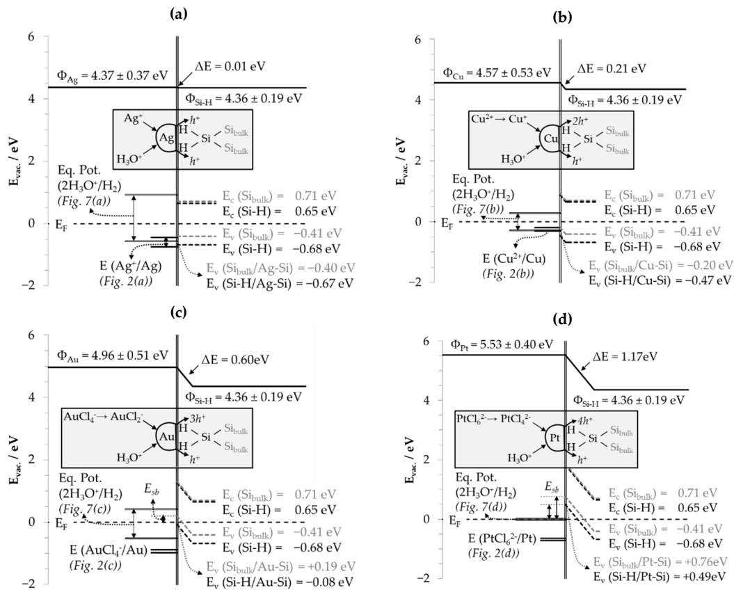
Figure 3. Work functions \Phi of the metals (a) Ag, (b) Cu, (c) Au and (d) Pt and that of hydrogen-terminated Si in vacuum [65–70]; the difference in work functions \Delta E ; the Fermi energy level E_F and that of the valence and conduction band of hydrogen-terminated silicon [71] ( E_v(\text{Si-H}) or E_c(\text{Si-H}) ) and of bulk silicon [72,73] ( E_v(\text{Si}_{\text{bulk}}) or E_c(\text{Si}_{\text{bulk}}) ); the energy levels of the valence bands at the metal–silicon contact ( E_v(\text{Si}_{\text{bulk}}/\text{Me-Si}) or E_v(\text{Si-H}/\text{Me-Si}) ); the Schottky barrier E_{\text{sb}} ; the redox levels of the \text{Me}^{z+}/\text{Me} half-cells E(\text{Me}^{z+}/\text{Me}) ; and the equilibrium potentials of the 2\text{H}_3\text{O}^+/\text{H}_2 half-cells at the metal surface Equation Pot. ( 2\text{H}_3\text{O}^+/\text{H}_2 ).
