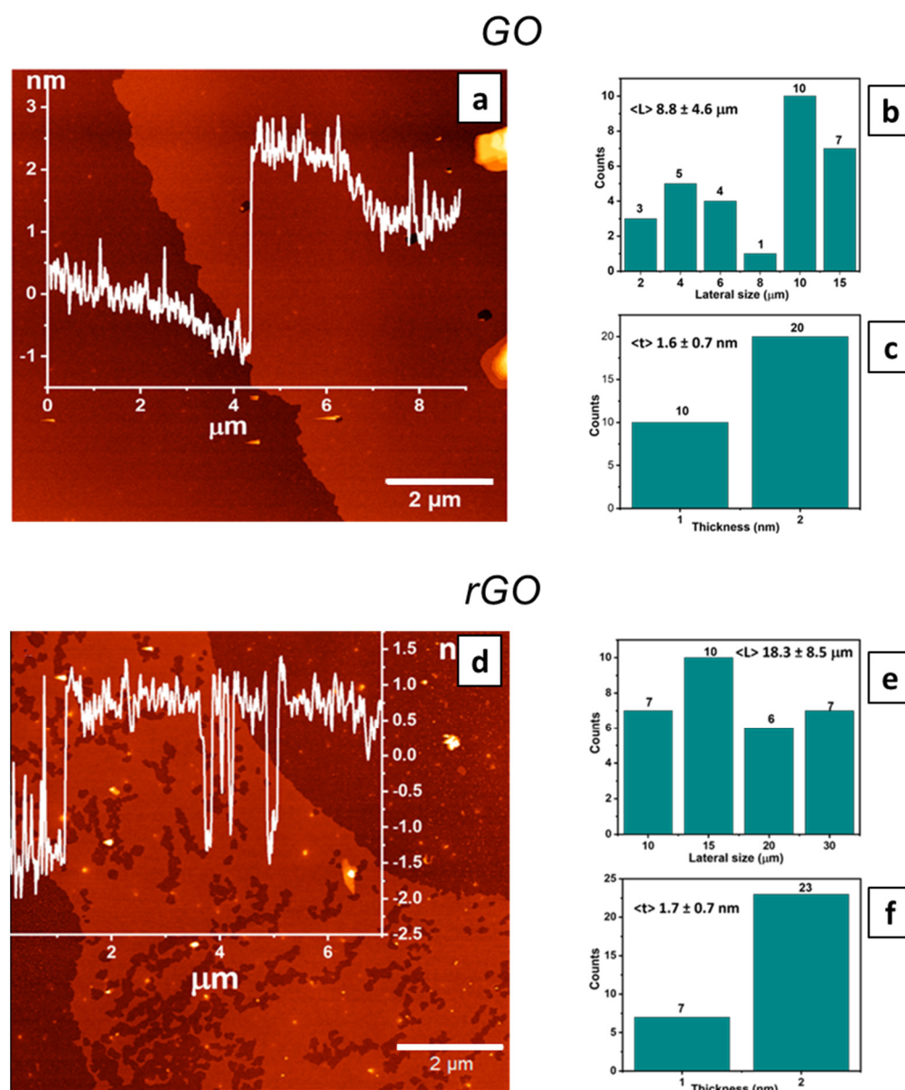
Figure 1. (a) Representative AFM image with a cross-sectional profile; average dimensional analyses of (b) the lateral size and (c) thickness distribution of GO flakes in ethanol dispersions. (d) Representative AFM image with a cross-sectional profile; average dimensional analyses of (e) the lateral size and (f) thickness distribution of rGO flakes in ethanol dispersions.
