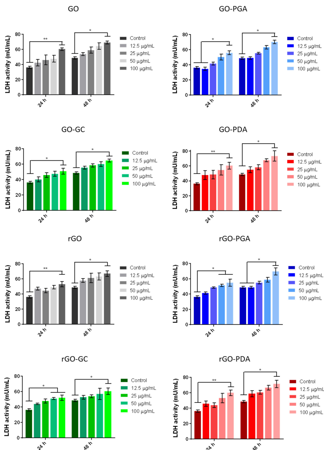
Figure 5. LDH assay of human chondrocytes of GO and rGO flakes with concentrations from 12.5 µg/mL to 100 µg/mL, compared with the use of different polymeric surfactants, namely propylene glycol alginate (GO-PGA and rGO-PGA), glycol chitosan (GO-GC and rGO-GC), and polydopamine (GO-PDA and rGO-PDA). Statistical significance was determined using the Kruskal–Wallis test with Dunn’s post hoc test to validate statistical significance, with * ( p -value < 0.05) and ** ( p -value < 0.01).
