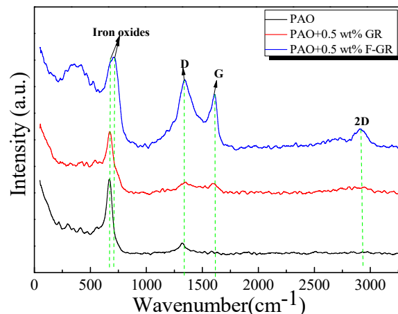
Figure 9. Raman analysis of worn traces of disks lubricated with PAO including 0.5 wt% GR and 0.5 wt% F-GR.
