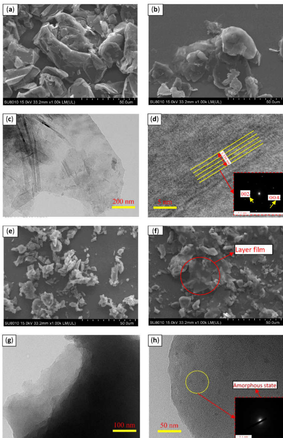
Figure 2. SEM and HRTEM images of different carbon materials. (a) SEM image of graphite, (b) SEM image of graphene, (c,d) HRTEM image of graphene and selected diffraction pattern, (e) SEM image of fluorinated graphite, (f) SEM image of fluorinated graphene (g,h) HRTEM image of fluorinated graphene and selected diffraction pattern.
