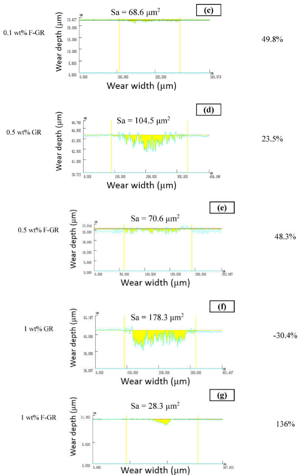
Figure 7. Crossing areas of wear traces of disks lubricated with different oil samples at 50 N and 10 mm/s for 60 min. (a) PAO6, (b) 0.1 wt% GR, (c) 0.1 wt% F-GR, (d) 0.5 wt% GR, (e) 0.5 wt% F-GR, (f) 1 wt% GR, (g) 1 wt% F-GR.
