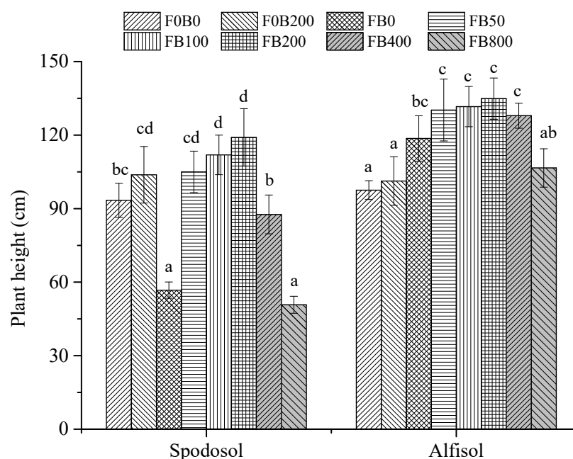
Figure 1. Effects of CNPs on the plant height of corn grown in Spodosol and Alfisol soils on the 49th day after transplanting. F0B0, control (without fertilizers and CNPs); F0B200, without fertilizers and with CNPs at 200 mg kg -1 soil; and FB0, FB50, FB100, FB200, FB400 and FB800 represent those with fertilizers and CNPs at application rates of 0, 50, 100, 200, 400 and 800 mg kg -1 soil, respectively. Error bars represent the standard error of the mean (n = 5). The letters a, b, c, and d indicate statistically significant difference at p < 0.05 within each group comparison between the treatments. Bars with no common letters are significantly different ( p < 0.05 ).
