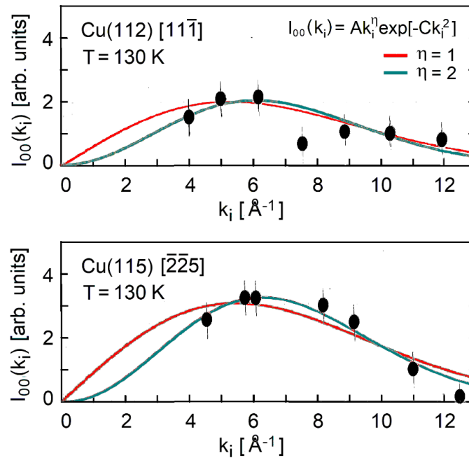
Figure 3. Specular HAS intensity as a function of the incident wave vector for the copper vicinal surfaces Cu(112) and Cu(115), measured at a surface temperature of 130 K along the directions normal to the steps [11\bar{1}] and [2\bar{2}5] , respectively, ( \bullet , from Miret-Artés et al. [46]). Solid lines show the fits of the HAS data with Equation (6) (reproduced in the upper panel) with two different values of the exponent \eta .
