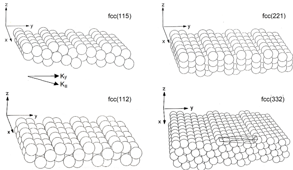
Figure 1. Ball models showing the structure of the (115) and (112) ( left ) and of the (221) and (332) ( right ) vicinal surfaces of a monatomic face-centered cubic (fcc) crystal (adapted from [47]). The orthogonal coordinates in the diagram are those of the vicinal surface; the wave vector component normal to steps lying in the terrace plane is here denoted as K_{\parallel} .
