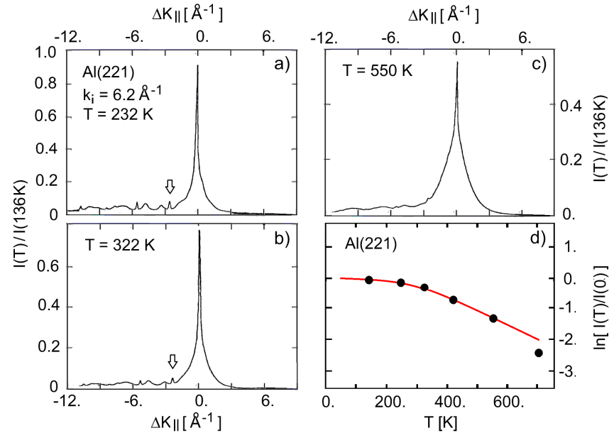
Figure 4. (a–c) HAS angular distributions from the Al(221) surface around the specular peak at three different surface temperatures and the same incident wave vector k_i = 6.2\text{ \AA}^{-1} as functions of the parallel wave vector change in the direction [\bar{1}\bar{1}4] normal to the steps [54]. Intensities are shown in units of the specular intensity at T = 136\text{ K} . The arrows in panels (a,b) indicate the positions of possible features from down-hill terrace specular scattering. (d) Temperature dependence of the DW exponent. The linear part of the fit (red full line above 300 K) indicates \lambda_{\text{HAS}} = 0.71 , while the point at 712 K would be fitted by a slope in the 550–712 K range corresponding to \lambda_{\text{HAS}} = 1.33 .
