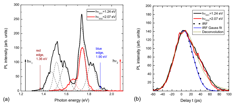
Figure 3. (a) PL spectra of quantum prism formed on SOI and excited with strong silicon absorption at h\nu_{\text{ex}2} = 2.1\text{ eV} (red curve), and weak silicon absorption h\nu_{\text{ex}1} = 1.2\text{ eV} (black curve). (b) The corresponding PL decays and system instrumental response function (dashed line with Gauss fit of 40 ps FWHM).
