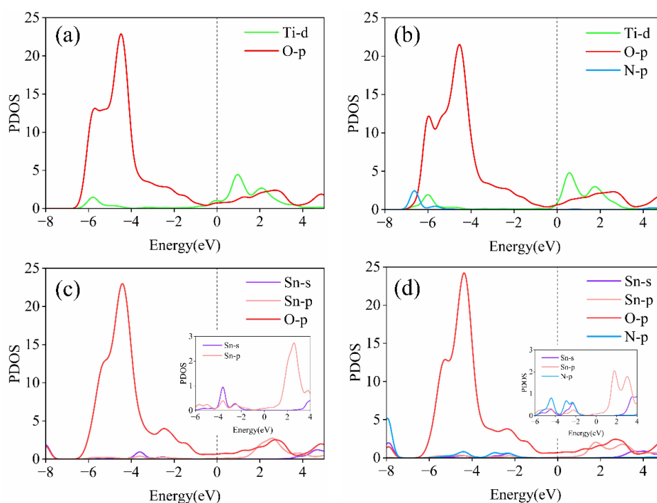
Figure 3. (a) PDOS of \text{Ti}/\text{Ti}_3\text{C}_2\text{O}_2 . (b) PDOS of \text{Ti}/\text{Ti}_3\text{C}_2\text{O}_2 + \text{NH}_3 . (c) PDOS of \text{Sn}/\text{Ti}_3\text{C}_2\text{O}_2 . (d) PDOS of \text{Sn}/\text{Ti}_3\text{C}_2\text{O}_2 + \text{NH}_3 .
