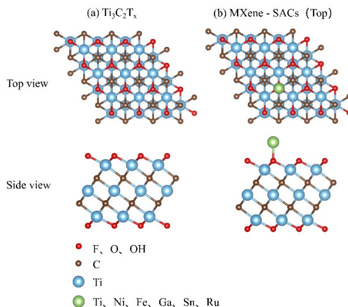
Figure 1. Schematic of \text{Ti}_3\text{C}_2 MXene pristine and doped monolayers.
