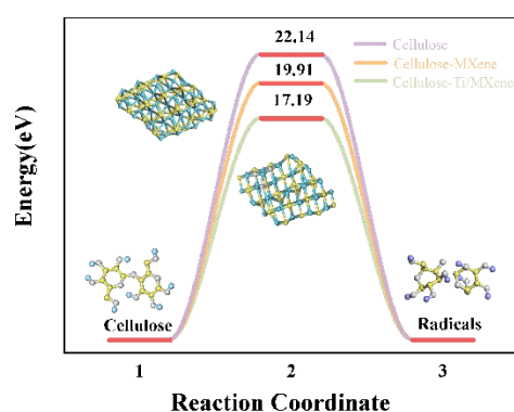
Figure 5. Proposed reaction pathways and relative energy profiles for cellulose-derived conversion in the uncatalyzed, \text{Ti}_3\text{C}_2\text{O}_2 , and \text{Ti}/\text{Ti}_3\text{C}_2\text{O}_2 systems.
