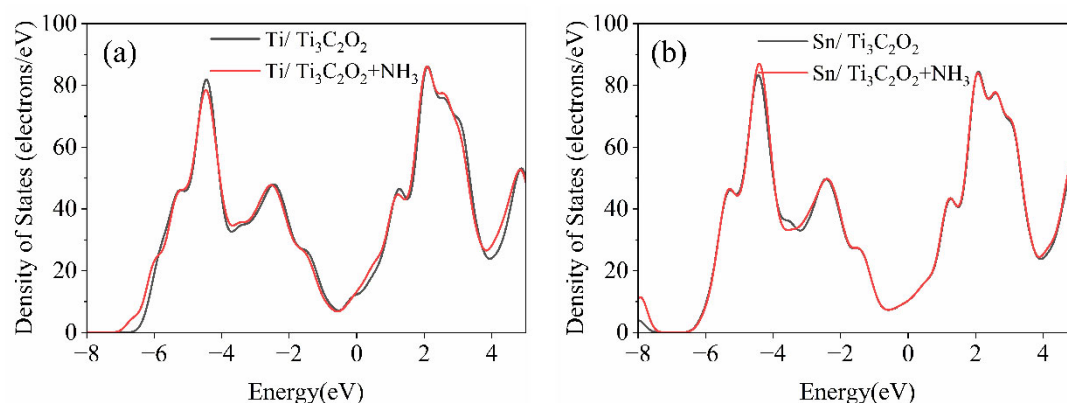
Figure 2. Density of states of representative MXene-supported single-atom systems before (a) and after \text{NH}_3 adsorption (b).
