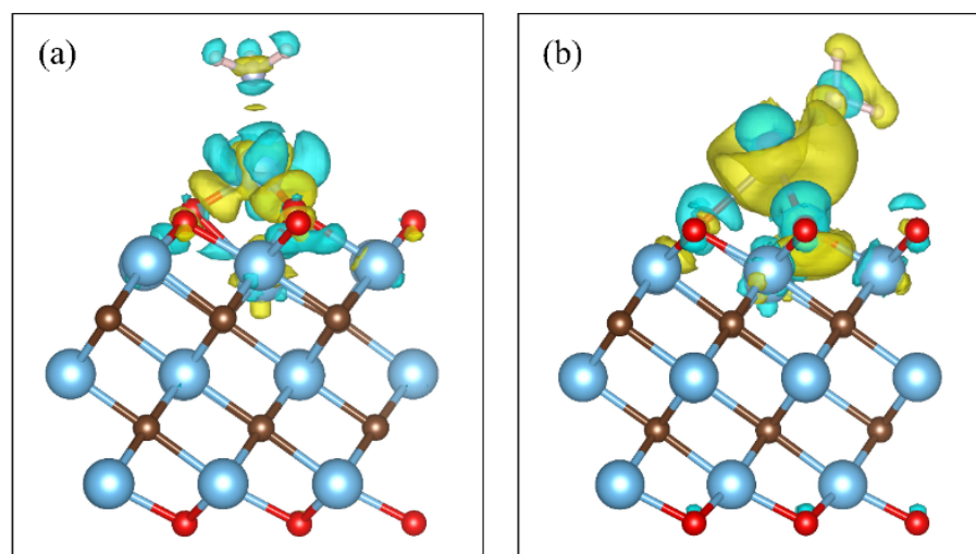
Figure 4. Charge density difference of \text{NH}_3 adsorption on representative MXene-supported single-atom sites: (a) \text{Ti}/\text{Ti}_3\text{C}_2\text{O}_2 + \text{NH}_3 . (b) \text{Sn}/\text{Ti}_3\text{C}_2\text{O}_2 + \text{NH}_3 . Note: yellow indicates an increase in charge density; blue indicates a decrease in charge density.
