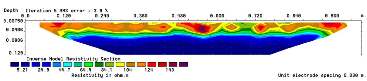
Figure 4. laB dataset: RES2DINV inverted section for Model C fully saturated, a = 30 mm, RMS = 3.9%, 5 iterations. Pervasive low \rho with smooth depth gradient and lateral uniformity.
