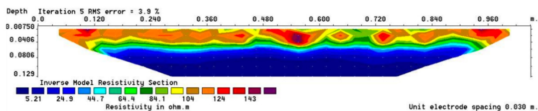
Figure 5. labmuftah dataset: RES2DINV inverted section for Model D corroded, a = 30 mm, RMS = 3.9%, 5 iterations. Heterogeneous near-surface layer above a sharp boundary at z \approx 40 mm with pervasive low \rho at rebar depth—the depth-preferential corrosion signature.
