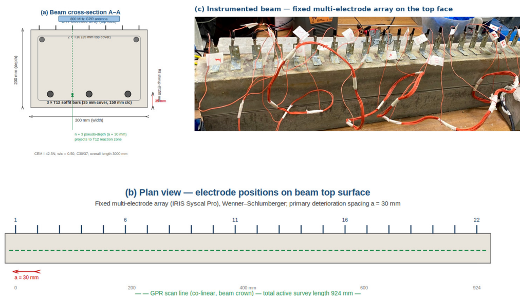
Figure 1. Beam cross-section and survey setup. (a) Cross-section A–A showing the reinforcement layout and 35 mm soffit cover, the ERT electrode array on the top (compression) face, and the 800 MHz GPR antenna scanning path; the n = 3 pseudo-depth at a = 30 mm projects to the T12 rebar reaction zone. (b) Plan view of the fixed multi-electrode array on the beam top surface (IRIS Syscal Pro; Wenner–Schlumberger, IRIS Instruments, Orléans, France), with the co-linear GPR scan line along the beam crown. (c) Photograph of the instrumented beam showing the fixed multi-electrode array, the numbered electrode leads, and the soffit chamfer.
