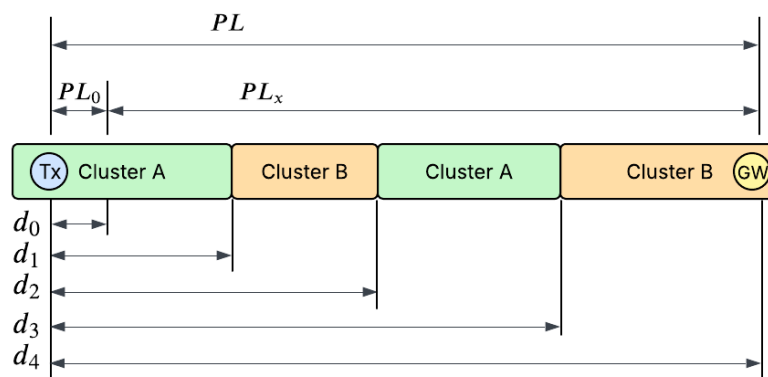
Figure 14. A more complicated case where subregions are traversed multiple times. Adapted from [34].
