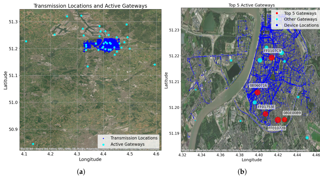
Figure 10. (a) Spatial distribution of the active gateways and transmissions. (b) Most active gateways.
