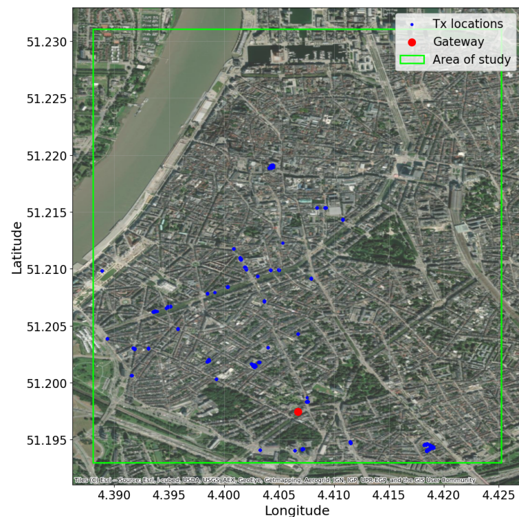
Figure 15. Transmission locations after performing filtering process.
