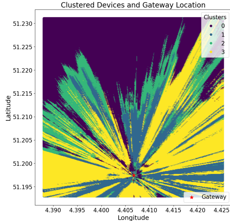
Figure 7. Visualization of the clusters at K = 4 .
