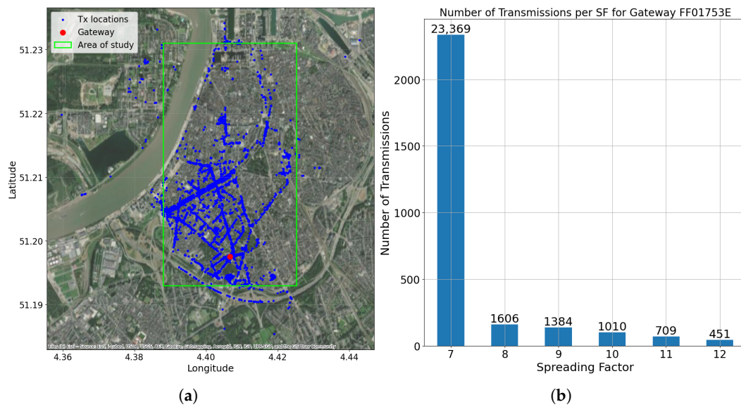
Figure 12. (a) Transmission locations and gateway located at coordinates 51.1974874° N and 4.406706° E. (b) Number of received transmissions per spreading factor for selected gateway FF01753E.
