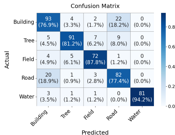
Figure 2. Land cover classification confusion matrix.
