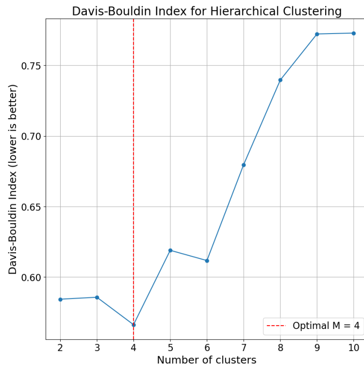
Figure 6. Davies–Bouldin indices at various number of clusters, showing K = 4 as optimal.
