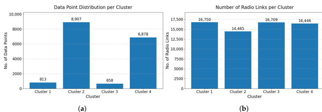
Figure 16. (a) Data point distribution per cluster and (b) number of radio links per cluster.
