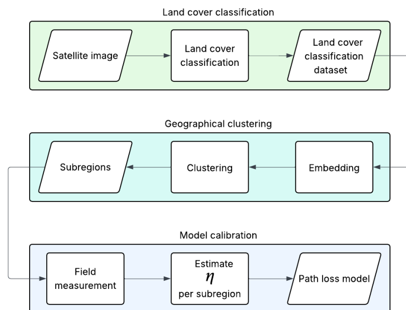
Figure 1. Path loss model development process using the proposed method.
