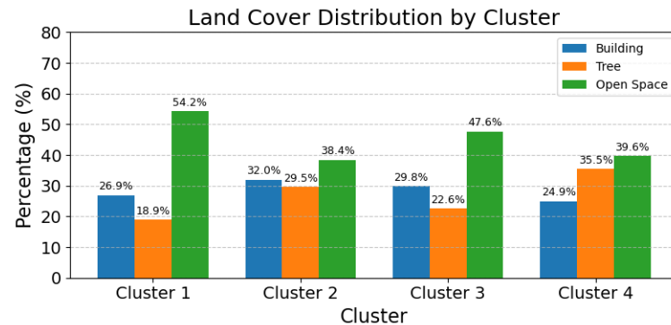
Figure 8. Land cover distribution (%) for each cluster.
