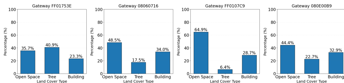
Figure 11. Land cover frequency distribution of each most active gateway.
