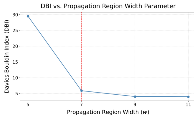
Figure 4. Davies–Bouldin indices at various propagation widths w , showing w = 7 having the largest marginal improvement.
