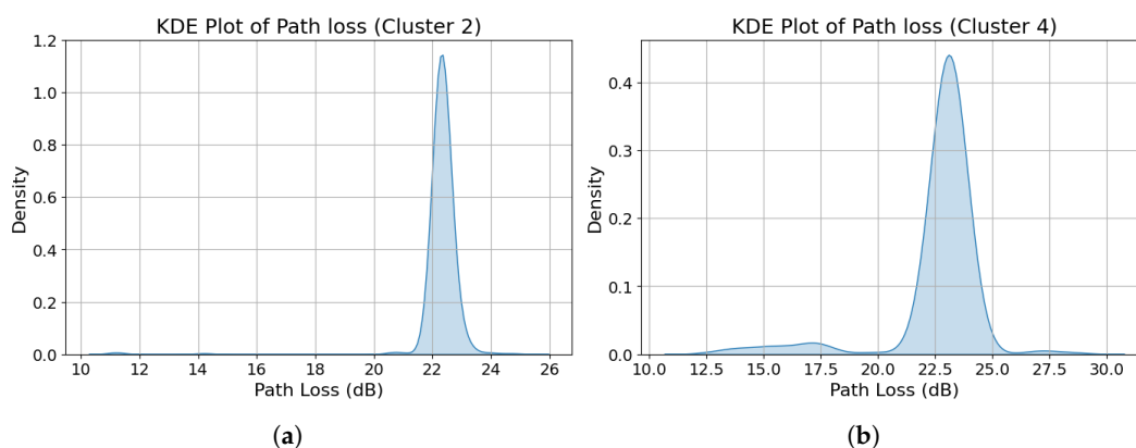
Figure 18. Kernel density estimate plots of path loss values for (a) Cluster 2 and (b) Cluster 4.
