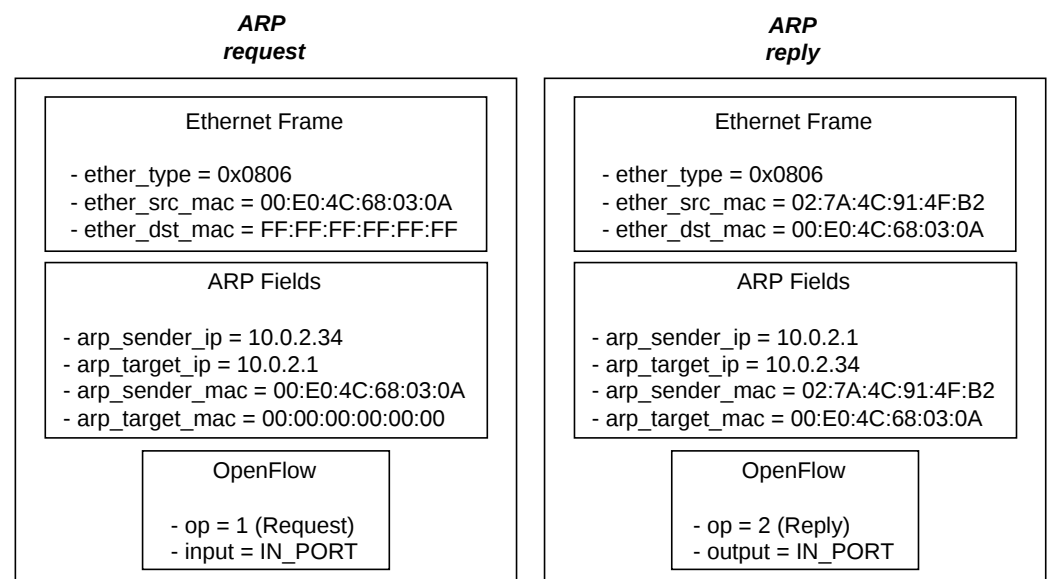
Figure 2. ARP packet handling SGAR strategy.
