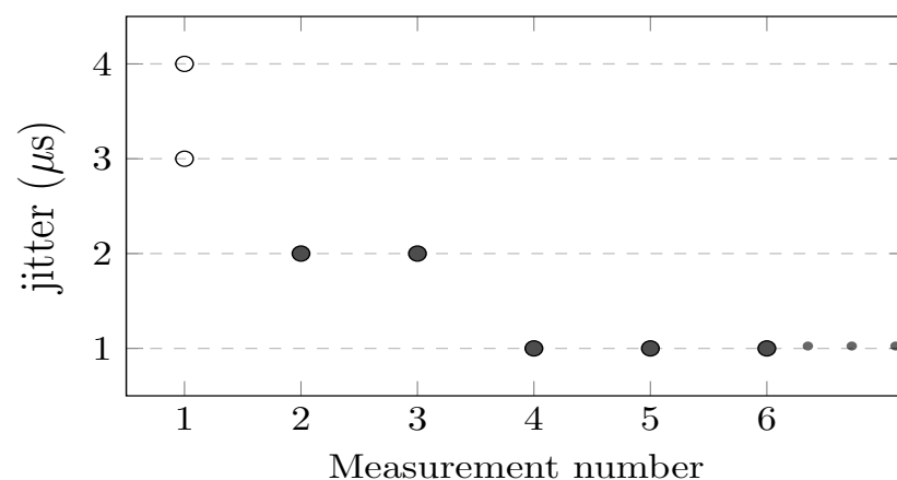
Figure 9. Jitter behavior for Mininet: (a) results for the first three strategies; (b) results for the SGAR strategy. The white dot indicates the point that may take two possible values.
