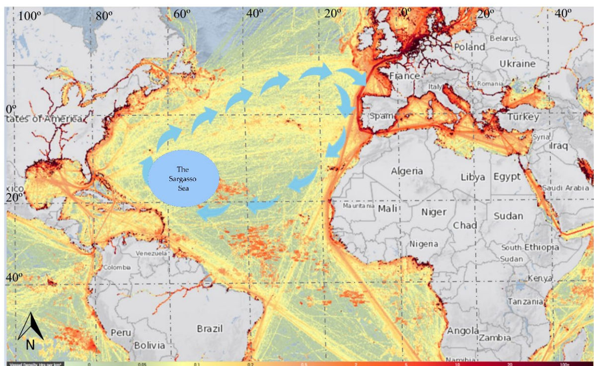
Figure 1. Map with the route followed by Anguilla anguilla that grows in Iberian rivers, showing the spawning site (Sargasso Sea), the maritime traffic occurring on 24 May 2024, and the migration route the species follows between Iberian rivers and the Sargasso Sea (blue arrows). This self-made map has been generated from the website https://globalmaritimetraffic.org/ [14] (accessed on 11 August 2024).
