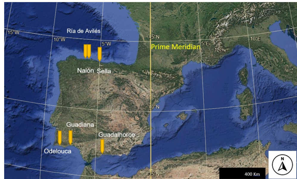
Figure 3. Map with the locations of the six estuaries analyzed: those of the Nalón and the Sella rivers and the estuary of Avilés, in the region of Asturias, Spain, and those of the Odelouca, in Portugal, Guadiana, on the Portugal–Spain border, and Guadalhorce rivers, in Málaga, Spain (Andalusia region). This self-made map has been generated from the website https://earth.google.es/ [38] (accessed on 23 January 2025).
