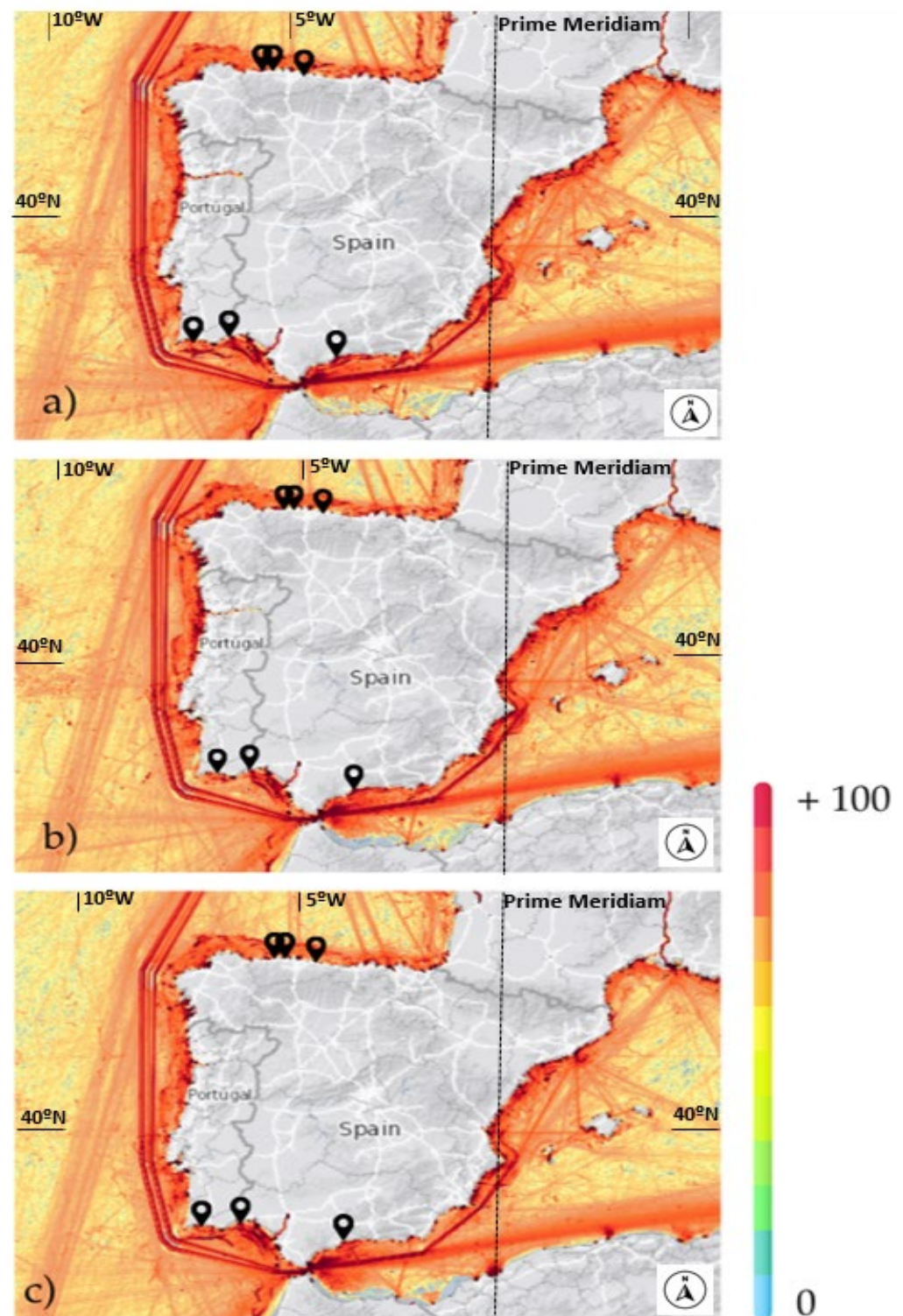
Figure 6. Cumulative pressure scores of the maritime traffic in the Iberian Peninsula during December (a), January (b), and February (c). The color scale ranges from blue (low pressure) to red (high pressure). The values range from 0 to 100+, representing relative cumulative pressure scores. This map has been generated from the website https://globalmaritimetraffic.org/ [14] (accessed on 11 August 2024).
