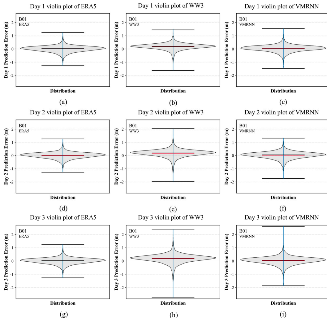
Figure 10. Violin plots comparing model results against in situ data at different prediction lead times: (a–c) violin plots of day 1 for ERA5, WW3, VMRNN; (d–f) violin plots of day 2 for ERA5, WW3, VMRNN; (g–i) violin plots of day 3 for ERA5, WW3, VMRNN. Day 1 (3–24 h); day 2 (27–48 h); day 3 (51–72 h).
