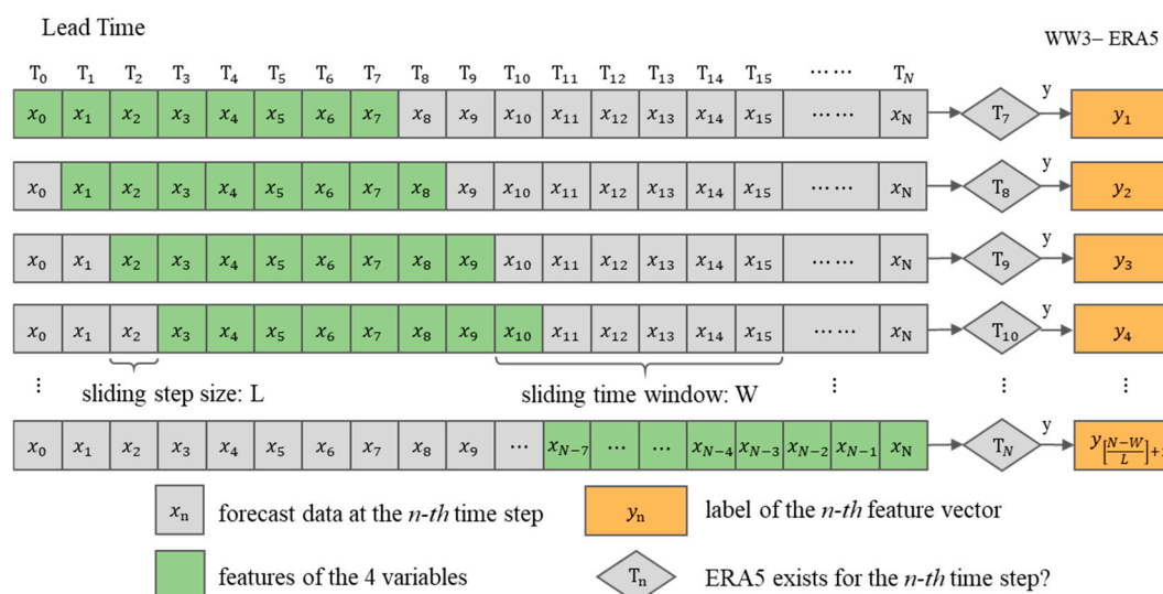
Figure 3. Sample dataset construction using the TSW method.
