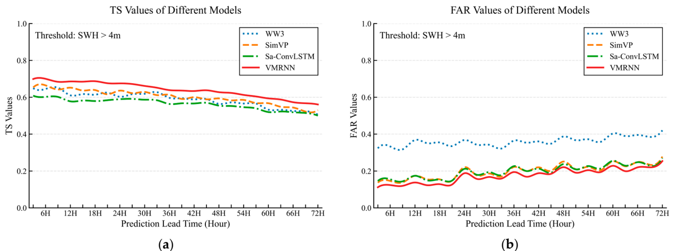
Figure 8. Time-series curves of TS and FAR for prediction of waves Above 4 m: (a) TS values of different models; (b) FAR values of different models.
