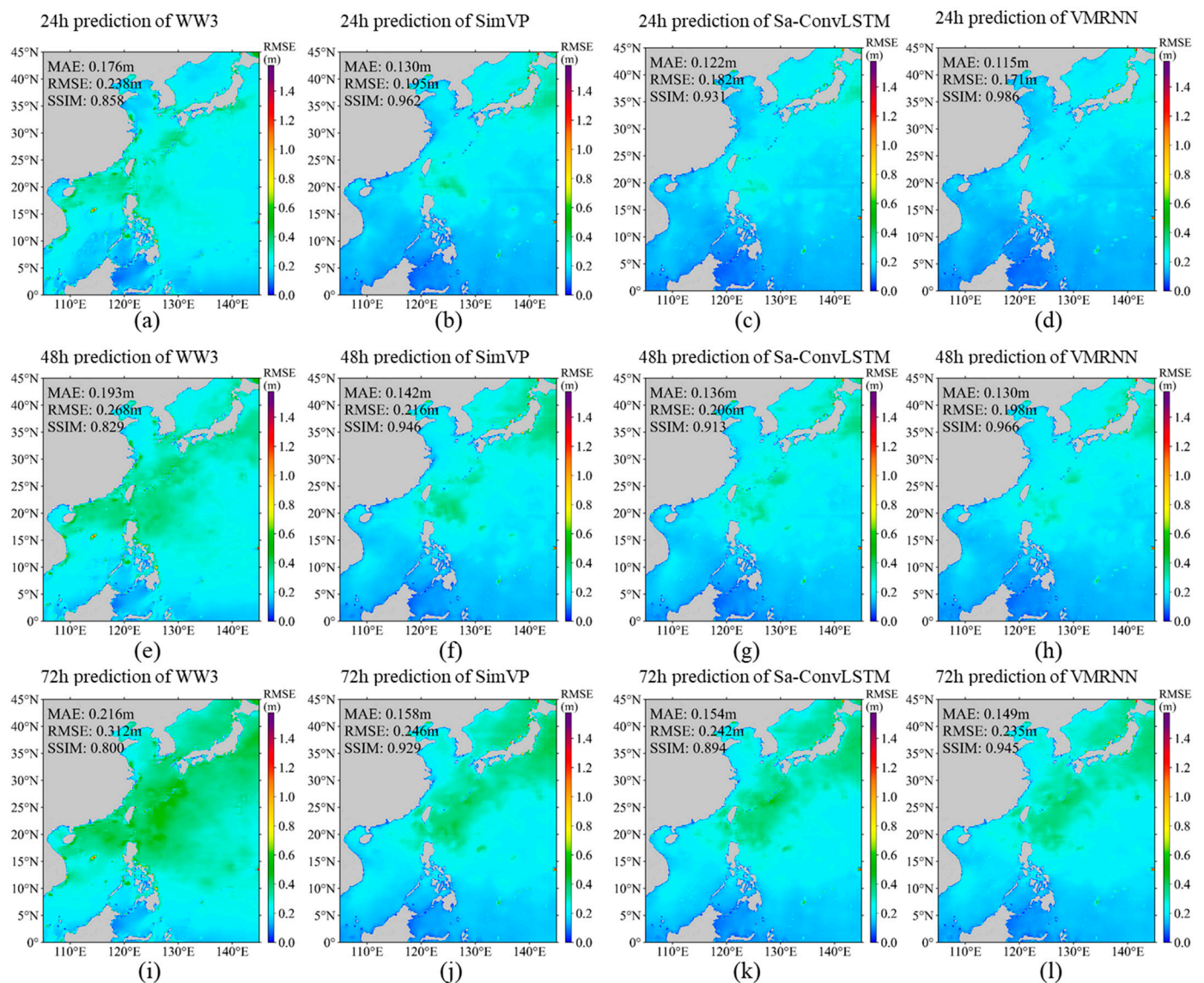
Figure 6. Spatial distribution of RMSE for SWH forecasts by different models at various lead times: (a–d) 24 h prediction of WW3, SimVP, Sa-ConvLSTM, VMRNN; (e–h) 48 h prediction of WW3, SimVP, Sa-ConvLSTM, VMRNN; (i–l) 72 h prediction of WW3, SimVP, Sa-ConvLSTM, VMRNN.
