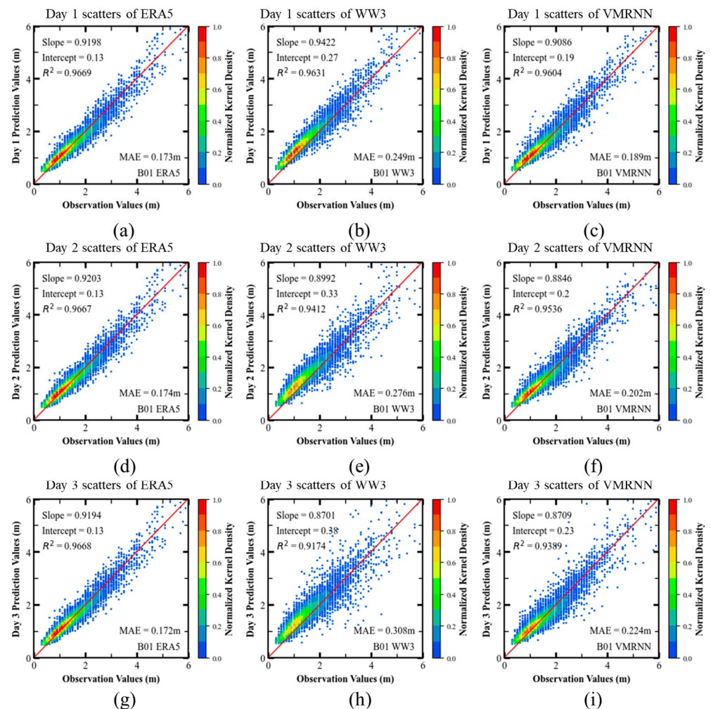
Figure 9. Scatter plot of model results versus in situ observations at different prediction lead times: (a–c) scatters of day 1 for ERA5, WW3, VMRNN; (d–f) scatters of day 2 for ERA5, WW3, VMRNN; (g–i) scatters of day 3 for ERA5, WW3, VMRNN. Day 1 (3–24 h); day 2 (27–48 h); day 3 (51–72 h).
