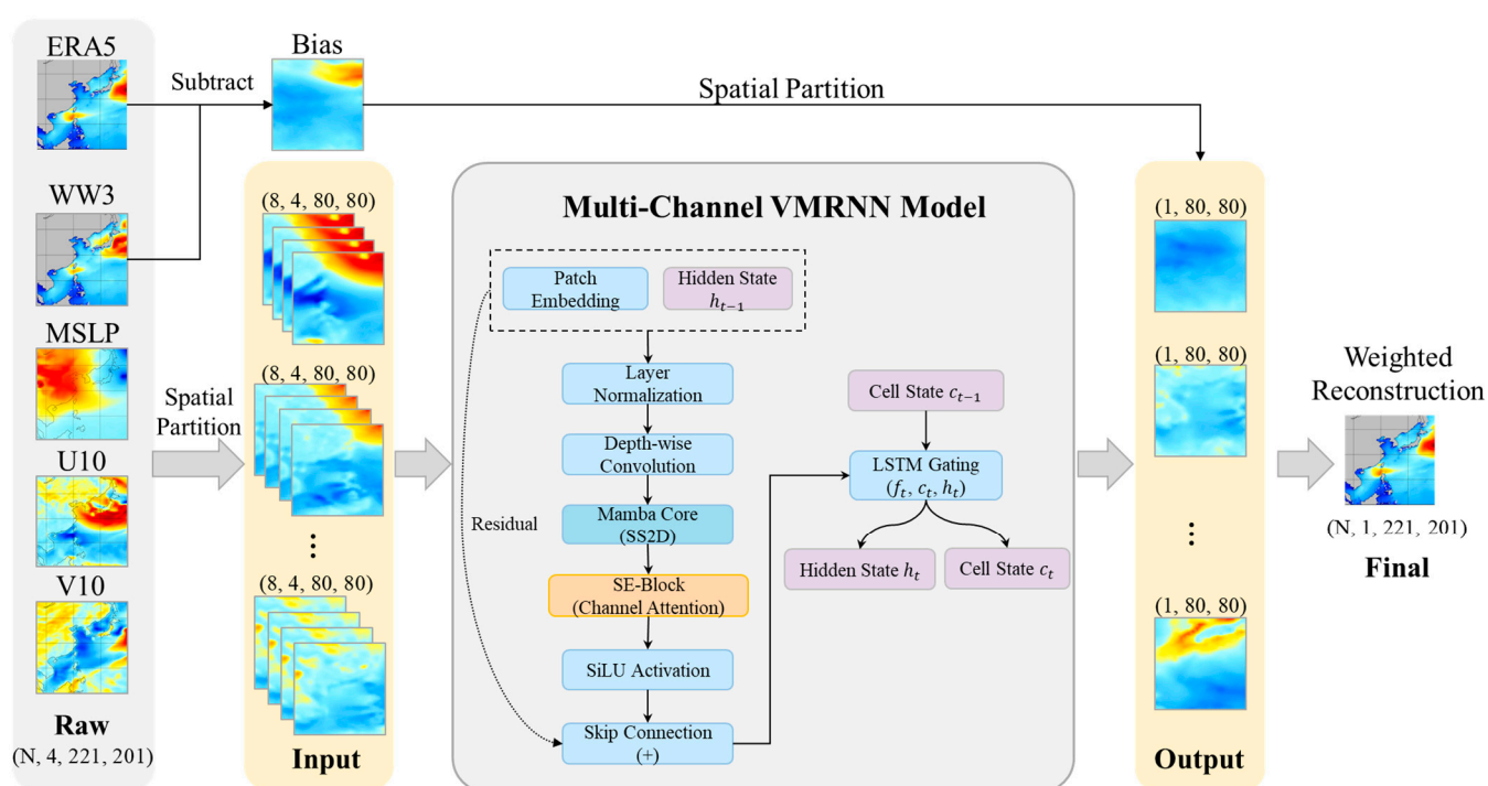
Figure 1. SWH prediction bias correction based on the multi-channel VMRNN: A technical flowchart.
