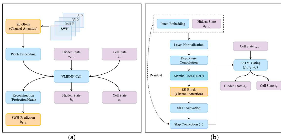
Figure 4. Structure of the VMRNN integrated with a channel attention mechanism: (a) Overall architecture; (b) VMRNN Cell detail.
