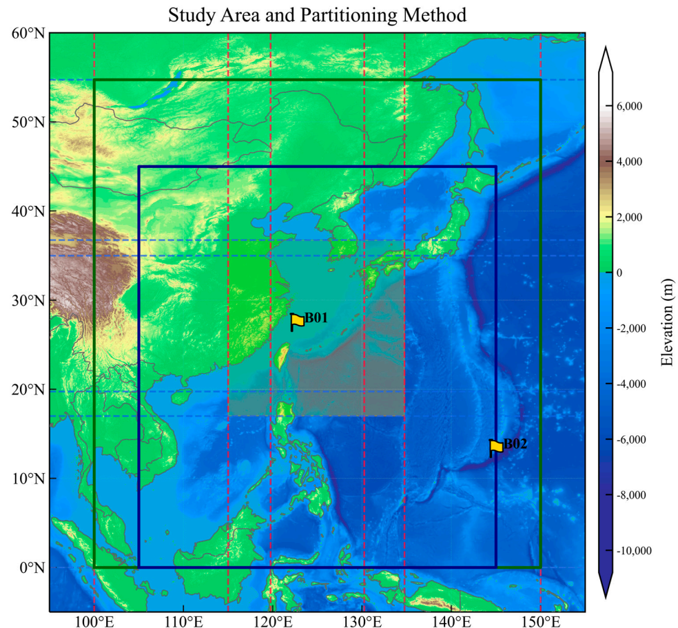
Figure 2. Study area and partitioning method. The meridional red dashed lines and zonal blue dashed lines divide the green box into a 3 \times 3 grid. Blue box is study area. Yellow flag symbols mark buoys B01 and B02, which are utilized for model validation.
