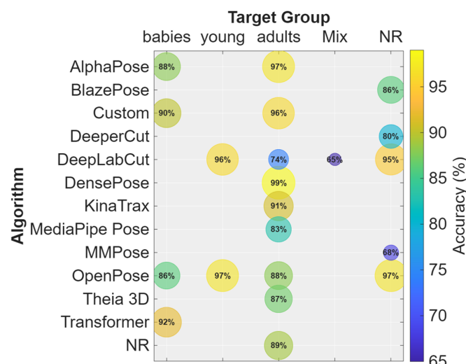
Figure 6. Accuracy distribution stratified by target age group. Note: Reported accuracy values should be interpreted with caution, as the underlying studies were not assessed for proper training methodology or healthy learning dynamics; thus, reported values may reflect overfitting or other methodological artifacts rather than true model generalizability.
