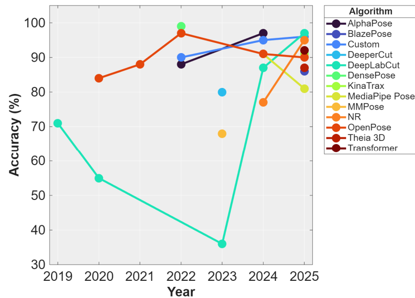
Figure 5. Evolution of algorithms accuracies. Note: Reported accuracy values should be interpreted with caution, as the underlying studies were not assessed for proper training methodology or healthy learning dynamics; thus, reported values may reflect overfitting or other methodological artifacts rather than true model generalizability.
