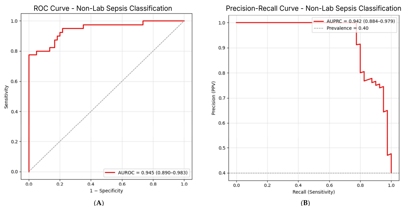
Figure 1. Receiver operating characteristic (ROC) curve (A) and precision – recall (PR) curve (B) for the logistic regression model classification of sepsis using the non-lab feature set. Curves were generated using aggregated out-of-fold predicted probabilities obtained from repeated stratified 5-fold cross-validation.
