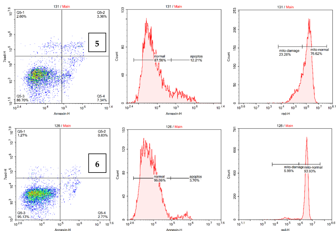
Figure 3. Detection of changes in mitochondrial membrane potential ( \Delta\Psi ) and apoptosis in Jurkat tumor cells treated with the studied compounds. The cells were treated with the tested compounds at their IC_{50} concentrations. Incubation time was 4 h. (1) LA, 6; (2) 8; (3) 11; (4) 15d; (5) 24d; (6) control. Staurosporine at a concentration of 0.8 \mu M. The cells were stained with the following dyes: MitoSense Red, annexin V—CF488A and 7-AAD.
