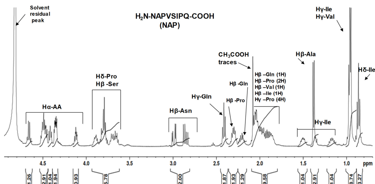
Figure 4. ^1\text{H} -NMR spectrum of NAP peptide dissolved in \text{D}_2\text{O} solvent.
