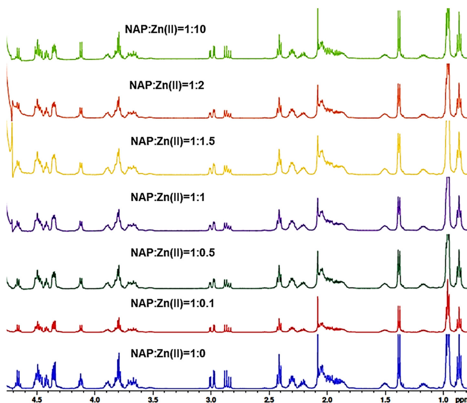
Figure 6. 1 H-NMR spectrum in the aliphatic region of NAP peptide titrated with increasing amounts of Zn 2+ at pH=5.
