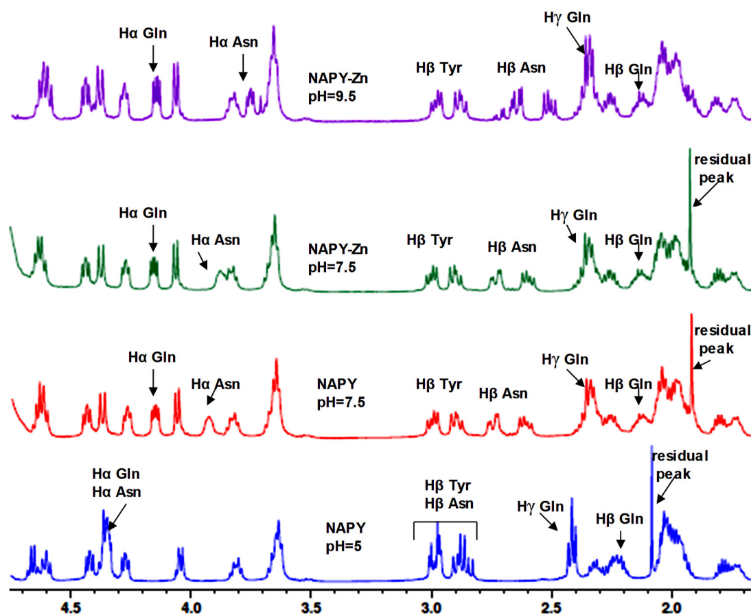
Figure 9. ^1\text{H} -NMR spectra of NAPI peptide titrated with \text{Zn}^{2+} ions at pH 7.5 and pH 9.5, at a 1:10 molar ratio.
