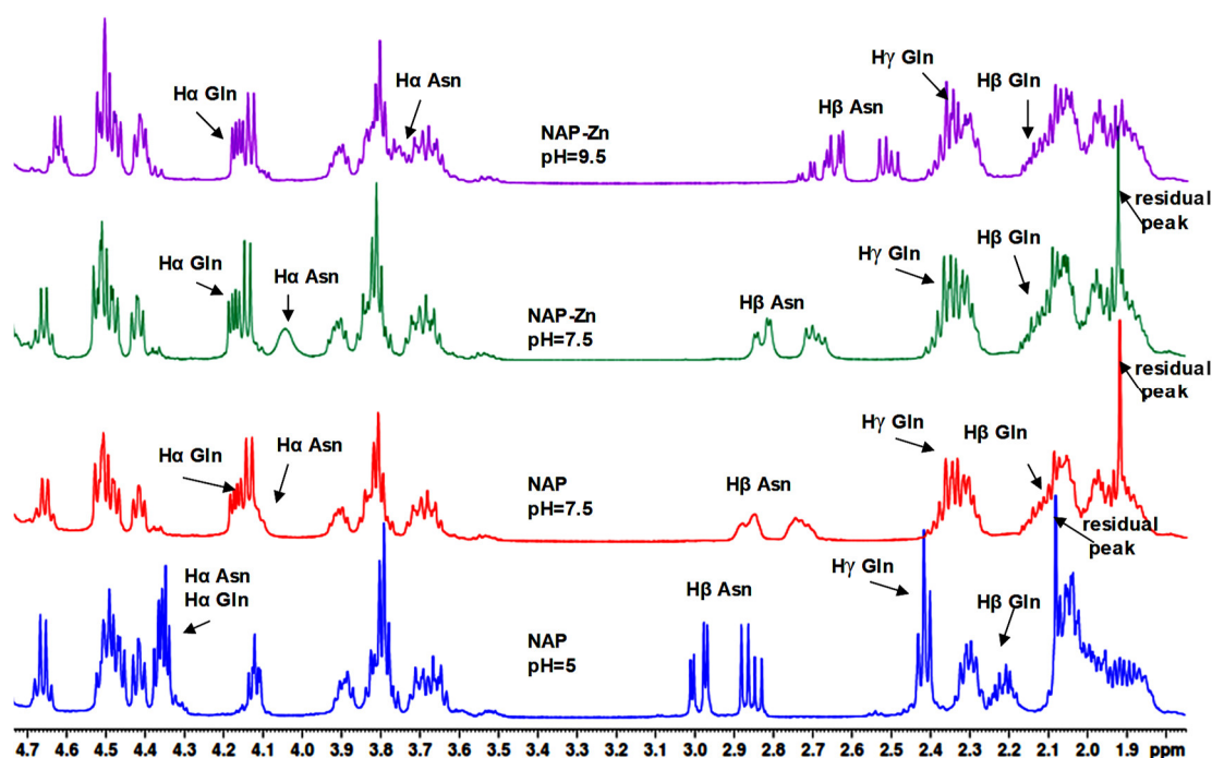
Figure 8. ^1\text{H} -NMR spectra of NAP peptide titrated with \text{Zn}^{2+} ions at pH 7.5 and pH 9.5, at a 1:10 molar ratio.
