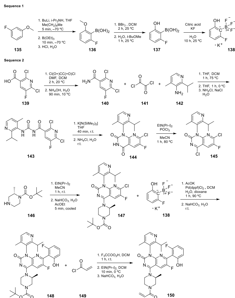
Scheme 15. 6-fluoro-7-(2-fluoro-6-hydroxyphenyl)-1-[4-methyl-2-(propan-2-yl)pyridin-3-yl]-4-[(2S)-2-methyl-4-(prop-2-enoyl)piperazin-1-yl]-1H,2H-pyrido[2,3-d]pyrimidin-2-one ( 150 ), AMG-510, [56].
