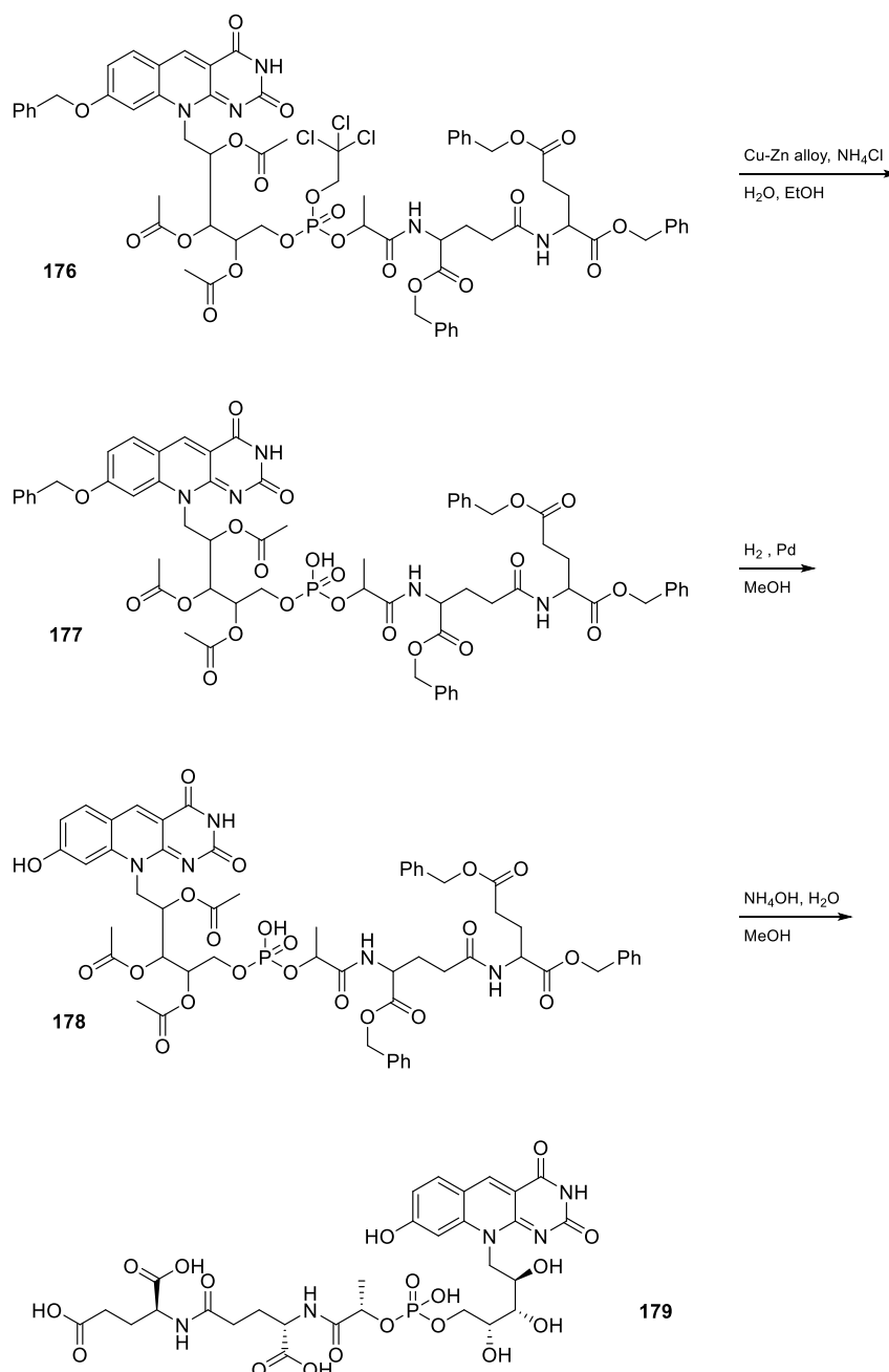
Scheme 18. (2S)-2-[(4S)-4-carboxy-4-[(2S)-2-[(hydroxy(((2R,3S,4S)-2,3,4-trihydroxy-5-(8-hydroxy-2,4-dioxo-2H,3H,4H,10H-pyrimido[4,5-b]quinolin-1-yl)pentyl]oxy))phosphoryl]oxy)propanamido]butanamido]pentanedioic acid ( 179 ) [59].
