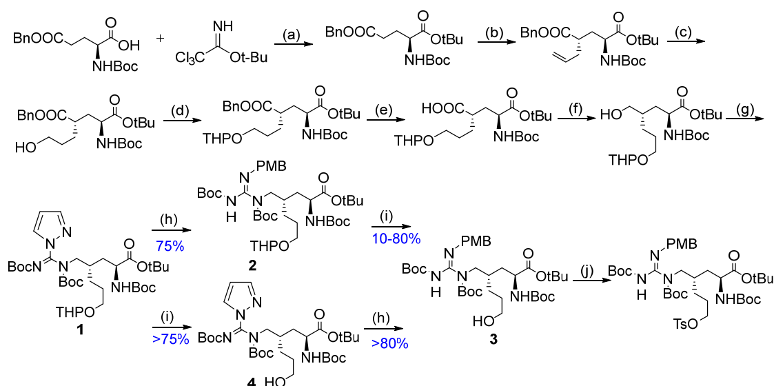
Scheme 1. Synthesis of precursor of (2S,4S)4-[ 18 F]FPArg. (a) tert-butyl 2,2,2-trichloroacetimidate (TBTCA), BF 3 ·Et 2 O, DCM, cyclohexane, rt, overnight; (b) LiHMDS, Allyl bromide, THF, -78 °C, 4 h; (c) 9-BBN, H 2 O 2 , NaOH, 0 °C–rt, 48 h; (d) DHP, PPTS, DCM, rt, 3 h; (e) Pd/C, H 2 , EtOH, rt, 2 h; (f) Ethyl chloroformate, NaBH 4 , THF, H 2 O, 0 °C–rt, 4 h; (g) N,N' -Di-Boc-1 H -pyrazole-1-carboxamide, triphenyl phosphine, diethyl azodicarboxylate, THF, 0 °C–rt, overnight; (h) 4-Methoxybenzylamine, N,N' -Diisopropylethylamine, ACN, 3 h; (i) PPTS, ethanol, 2 h; (j) p -toluenesulfonyl chloride, Et 3 N, DCM, rt, overnight.
