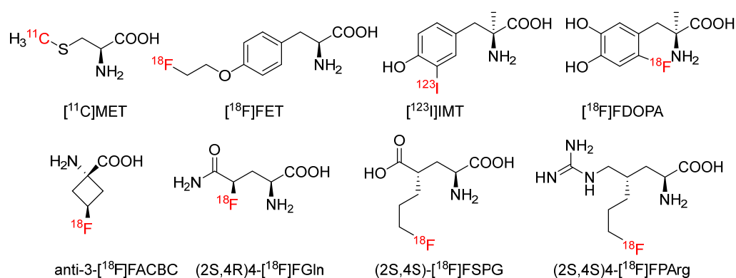
Figure 1. Chemical structures of [^{11}\text{C}]\text{MET} , [^{18}\text{F}]\text{FET} , [^{123}\text{I}]\text{IMT} , [^{18}\text{F}]\text{FDOPA} , anti-3- [^{18}\text{F}]\text{FACBC} , (2S,4R)4- [^{18}\text{F}]\text{FGln} , (2S,4S)- [^{18}\text{F}]\text{FSPG} and (2S,4S)4- [^{18}\text{F}]\text{FPArg} .
