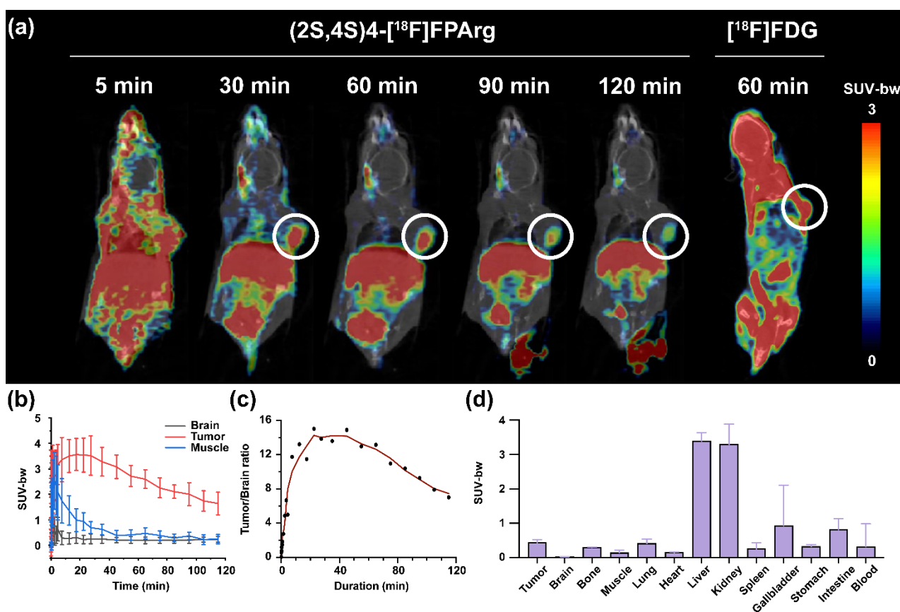
Figure 3. (a) The microPET-CT images of (2S,4S)4-[ 18 F]FPArg and [ 18 F]FDG in U87MG tumor-bearing nude mice, where the white circle indicates glioma area; (b) Time-activity curves of (2S,4S)4-[ 18 F]FPArg uptake in brain, muscle and tumor; (c) The tumor/brain SUV ratio of (2S,4S)4-[ 18 F]FPArg uptake in U87MG tumor-bearing nude mice; (d) Biodistribution of (2S,4S)4-[ 18 F]FPArg in U87MG tumor-bearing nude mice at 30 min point.
