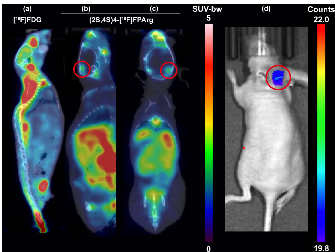
Figure 4. (a) The microPET–CT sagittal image of [ ^{18}\text{F} ]FDG in HS683–Luc tumor-bearing nude mice; The microPET–CT sagittal (b) and coronal (c) images of (2S,4S)4–[ ^{18}\text{F} ]FPArg in HS683–Luc tumor-bearing nude mice; (d) Bioluminescence imaging was collected for 1 min in a nude mouse bearing HS683–Luc glioma after injection of D–luciferin, where the red circle indicates glioma area.
