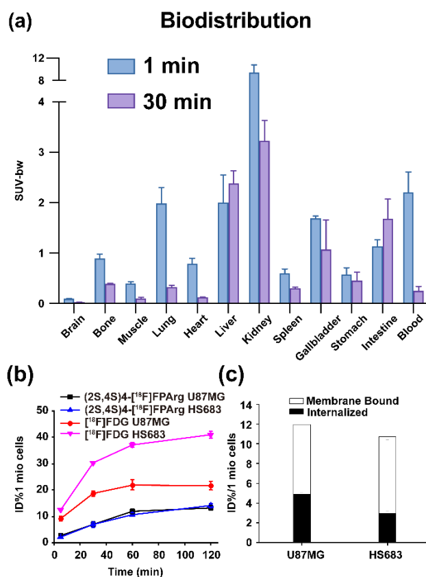
Figure 2. (a) In vivo biodistribution of (2S,4S)4-[ 18 F]FPArg in BALB/c mouse ( n = 4 ); Cell uptakes (b) and internalization (c) of (2S,4S)4-[ 18 F]FPArg in U87MG and HS683–Luc cells.
