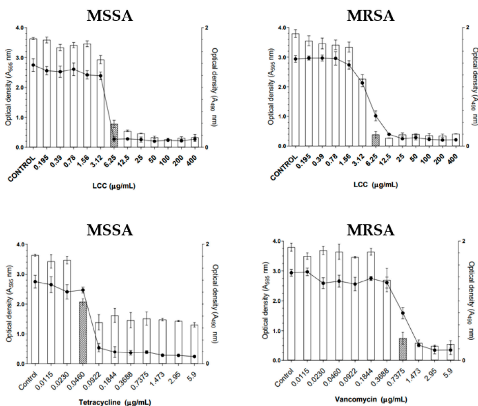
Figure 2. Effect of LCC (6.25 µg/mL) and the positive controls (tetracycline—0.046 µg/mL; vancomycin—0.737 µg/mL) on MSSA and MRSA biofilm formation, respectively. The hatched bars represent the minimum biofilm inhibitory concentration (MBIC 50 ) values. The lines represent the curve of the optical density (OD) values of biofilm metabolic activity in relation to the concentration of the tested sample.
