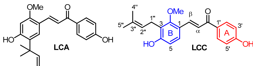
Figure 1. Structure of licochalcones A (LCA) and C (LCC).
