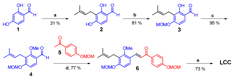
Scheme 1. Synthetic route for LCC. (a) Isoprenyl bromide, NaOH, MeOH, rt, 12 h; (b) MOMCl, K 2 CO 3 , acetone, rt, 24 h; (c) CH 3 I, K 2 CO 3 , acetone, rt, 12 h; (d) NaOH, EtOH, H 2 O, rt, 36 h; (e) HCl, EtOH, THF, 70 °C, 6 h. MOM = methoxymethyl.
