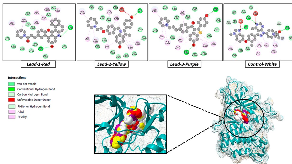
Figure 2. Depicts the two-dimensional (2D) ( Top ) and three-dimensional (3D) ( Bottom ) structures of HER2 with the ChEMBL193865 (Lead-1), ChEMBL46740 (Lead-2), ChEMBL151318 (Lead-3), and control. The bottom (3D) indicates the docking pose of the three compounds and references within the active site of the HER2: Lead-1 (Red), Lead-2 (Yellow), Lead-3 (Purple), and reference colors (White), respectively.
