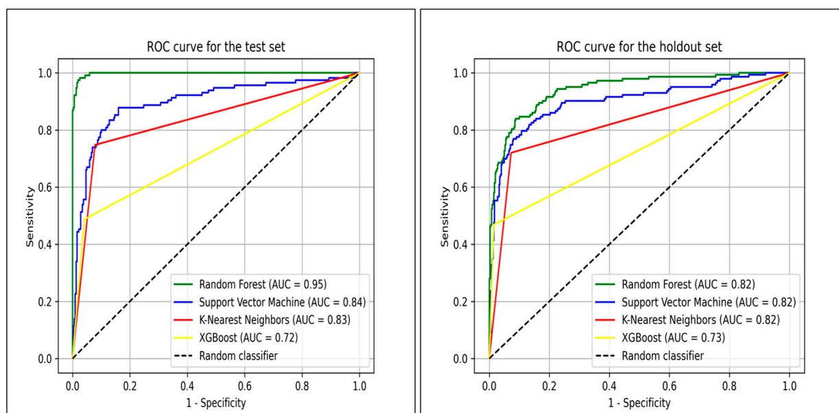
Figure 1. Receiver operating characteristic (ROC) curves of ML models to predict HER2 inhibitor prioritization. The test set is represented by the left panel, and the holdout set is represented by the right panel. Some of the models used are Random Forest, Support Vector Machine, K-nearest neighbors, and XGBoost.
