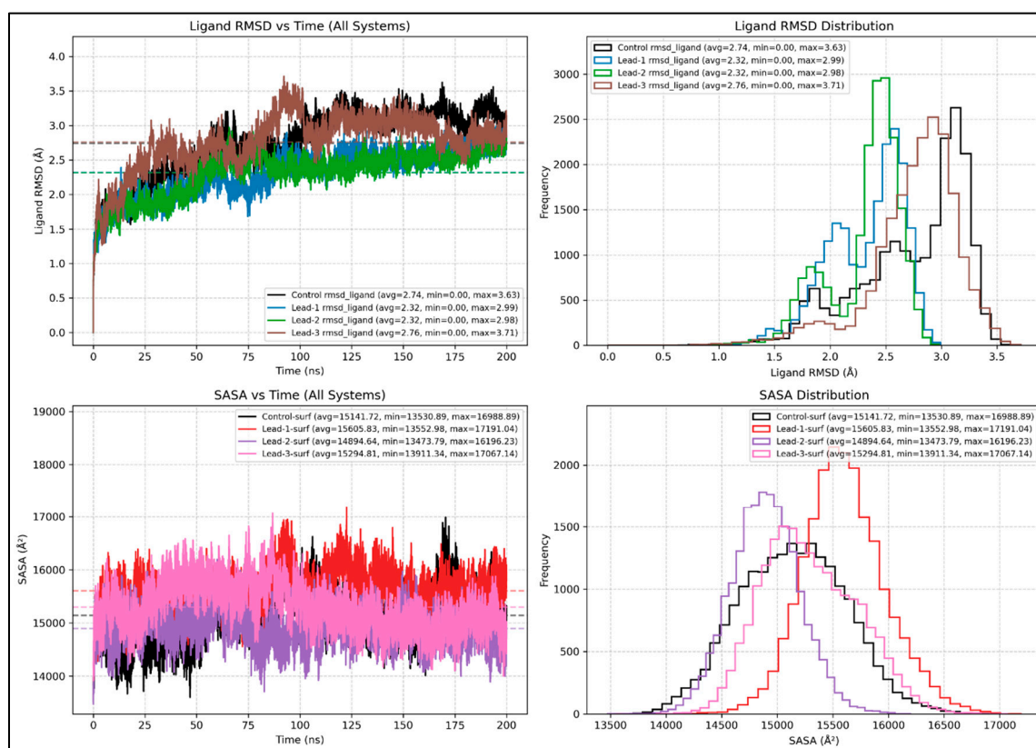
Figure 5. The Ligand-RMSD and SASA of HER2 in the presence of three compounds: CHEMBL193865 (Lead-1), CHEMBL46740 (Lead-2), CHEMBL151318 (Lead-3), and a control ligand after 200 ns of MD simulation. Left: The Ligand-RMSD (top), SASA (bottom) versus time curve, while the top right shows the Ligand-RMSD (top) and SASA (bottom) distribution.
