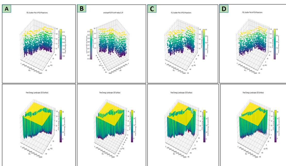
Figure 6. Depicts the PCA and FEL of the HER2–ligand complexes in the course of the MD simulations. The conformational sampling and dominant motions of three novel compounds,
