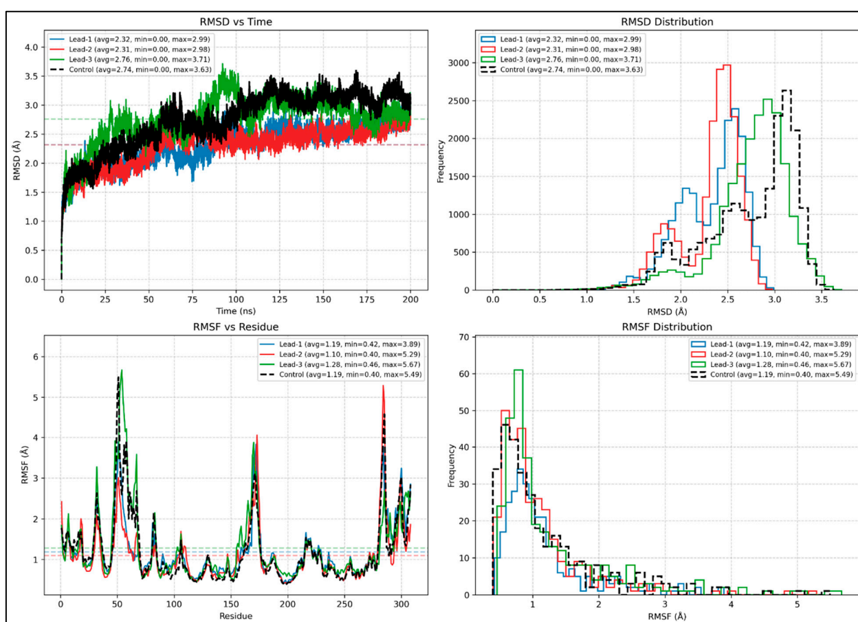
Figure 3. The RMSD and RMSF of HER2 in the presence of three novel ligands, CHEMBL193865 (Lead-1), CHEMBL46740 (Lead-2), CHEMBL151318 (Lead-3), and a control ligand after 200 ns of MD simulation. Left: The RMSD ( top ), RMSF ( bottom ) versus time curve, while the top right shows the RMSD ( top ) and RMSF ( bottom ) distribution.
