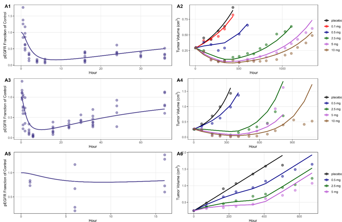
Figure 8. Model prediction and measured data for pEGFR (after 5 mg/kg dose) and tumor volume in PC9 (A1,A2), NCI-H1975 (A3,A4) and A431 (A5,A6).
