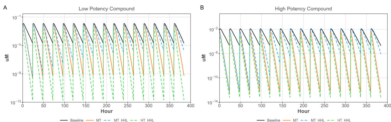
Figure 9. Effects of target protein pool and half-life on the exposure of covalent inhibitors. (A) Low-potency inhibitors ( K_i = 100 \mu\text{M} , k_{\text{inact}} = 3000 \text{ h}^{-1} , k_{\text{on}} = 10 \mu\text{M}^{-1}\text{h}^{-1} ) and (B) high-potency inhibitors ( K_i = 100 \mu\text{M} , k_{\text{inact}} = 30,000 \text{ h}^{-1} , k_{\text{on}} = 50 \mu\text{M}^{-1}\text{h}^{-1} ). Legends—MT: Target pool increased by 20,000-fold, MT_HHL: Target pool increased by 20,000-fold and half-life increased by 10-fold, HT_HHL: Target pool increased by 200,000-fold and half-life increased by 10-fold.
