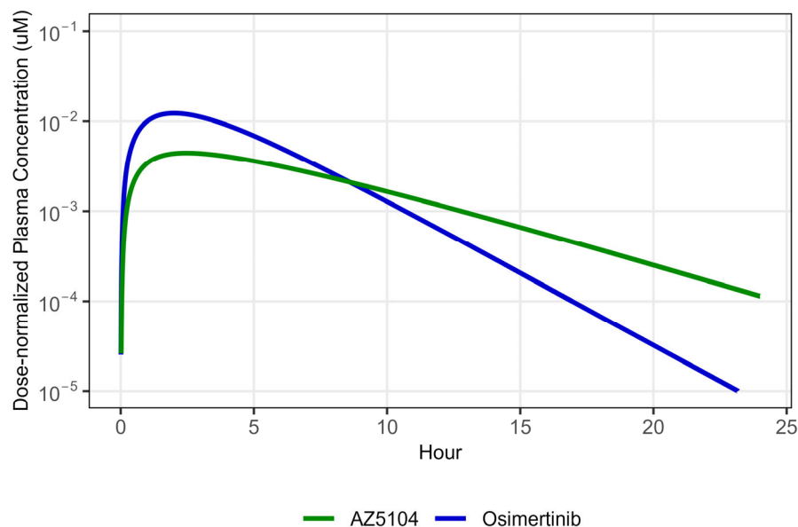
Figure 7. OSM PK model plasma concentration predictions in nude mice.
