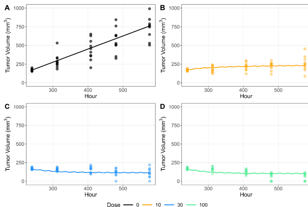
Figure 3. Efficacy of sotorasib following repeated daily oral dosing of 0 mg/kg (A), 10 mg/kg (B), 30 mg/kg (C), and 100 mg/kg (D) in Mia PaCa-2 xenograft-bearing mice. Solid lines are model predictions, and the solid circles are observations.
