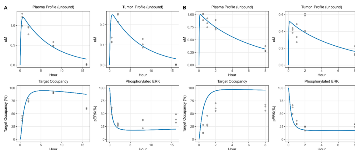
Figure 4. Pharmacodynamic model validation for two internal Amgen KRAS G12C inhibitors, Inhibitor-1 (A) and Inhibitor-2 (B). Plasma concentrations were fitted either with a one- or two-compartmental model, while tumor concentrations were predicted based on experimental tumor-plasma K_{p,uu} . The PD model was then used to independently predict target occupancy (%TO) and p-ERK inhibition (%p-ERK). Red lines are model predictions and black circles are observations.
