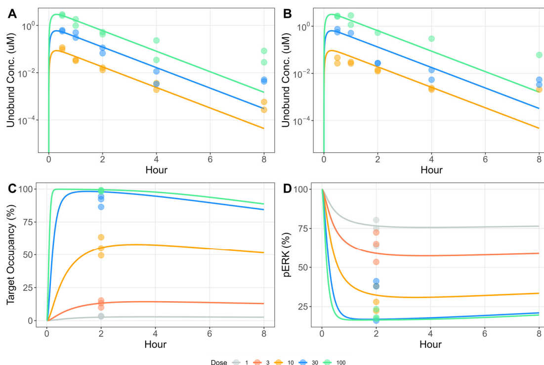
Figure 2. Unbound plasma concentrations (A), unbound tumor concentrations (B), target occupancy (C), and phospho-ERK inhibition (D) following administration of sotorasib in Mia PaCa-2 xenograft bearing mice. Solid lines are model predictions and the solid circles are observations.
