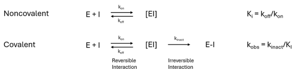
Figure 1. Binding mechanism for noncovalent and covalent drugs. E is enzyme, I is inhibitor, k_{\text{on}} is binding rate, k_{\text{off}} is dissociation rate, K_i is inhibition constant for reversible inhibitors, K_i is the inhibition constant for covalent inhibitors, and k_{\text{inact}} is rate of inactivation.
