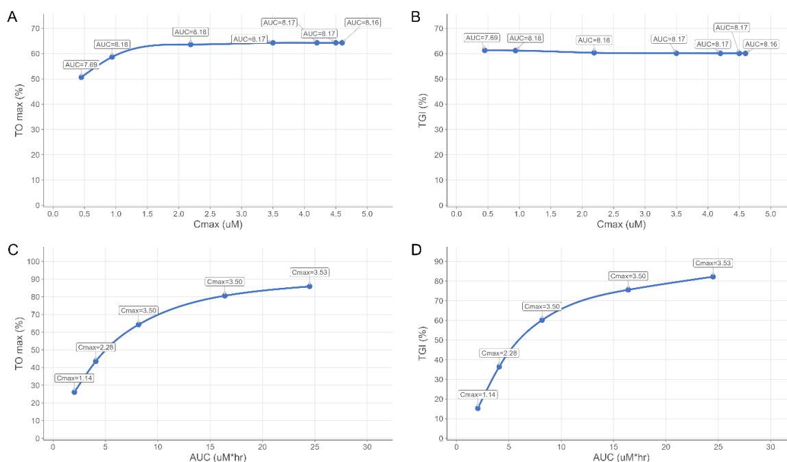
Figure 10. Sensitivity analysis showing the effects of C_{max} on target occupancy (%TO; (A)) and tumor growth inhibition (TGI; (B)), and the effects of AUC on %TO (C) and TGI (D) for KRAS G12C inhibitors.
