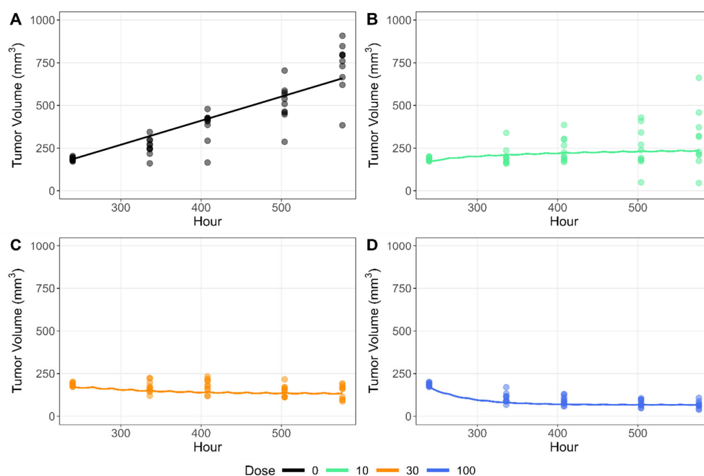
Figure 5. Validation of the efficacy model for an internal Amgen KRAS G12C inhibitor (inhibitor 1) following daily administration of 0 mg/kg (A), 10 mg/kg (B), 30 mg/kg (C), or 100 mg/kg (D) in mice.
