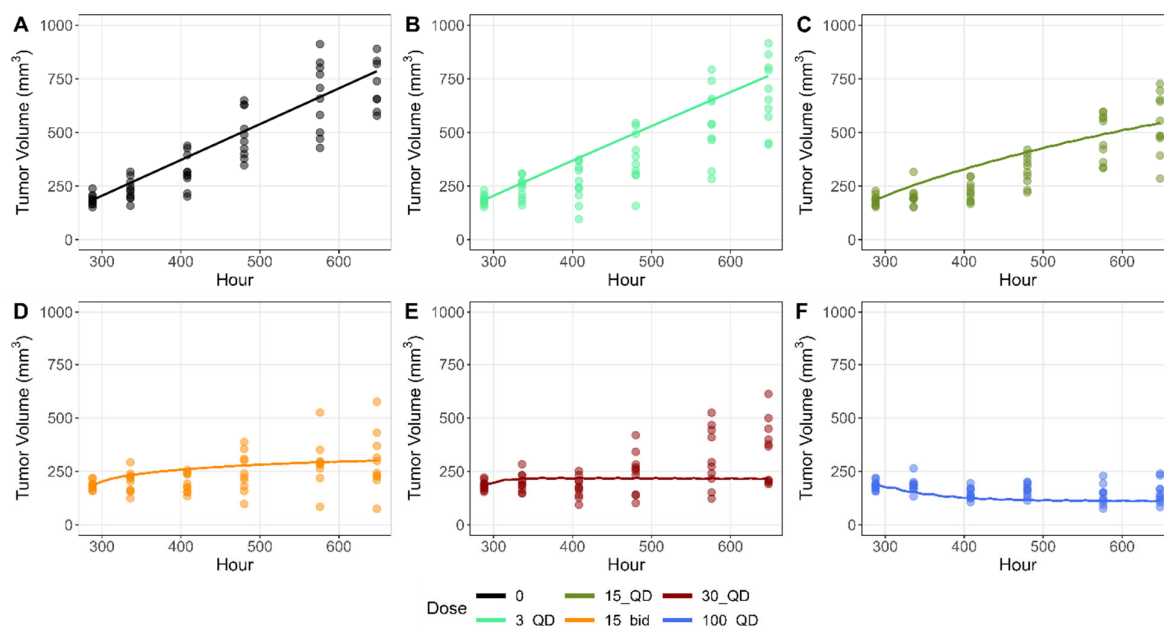
Figure 6. Validation of the efficacy model for an internal Amgen KRAS G12C inhibitor (inhibitor 2) following daily administration of 0 mg/kg (A), QD 3 mg/kg (B), QD 15 mg/kg (C), BID 15 mg/kg (D), QD 30 mg/kg (E), or QD 100 mg/kg (F) in mice bearing Mia PaCa-2 xenografts. Solid lines are model predictions, and solid circles are experimental observations. The zero-order tumor growth rate was estimated separately for each study given varying tumor growth kinetics across experiments.
