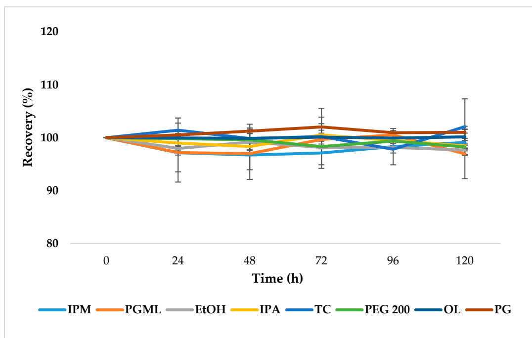
Figure S4. Recovery (%) of TBF-free base in a series of solvent systems after 24, 48, 72, 96 and 120 h at 32 \pm 1^\circ\text{C} ( n = 3 ; mean \pm SD).
