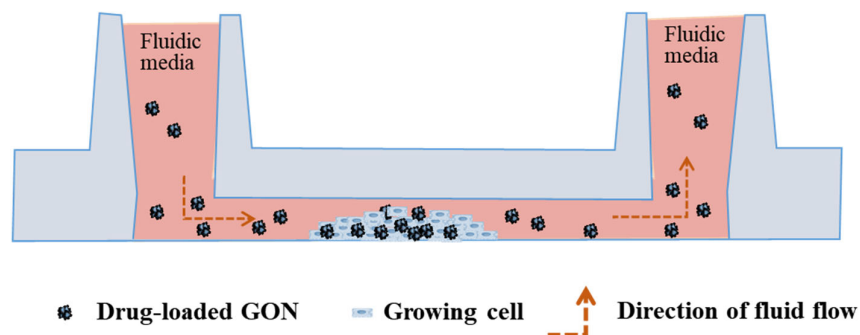
Figure 2. A cross-sectional view of a microfluidic cell chamber showing cellular behaviors of NPs under the biomimetic microfluidic system (BMS).
