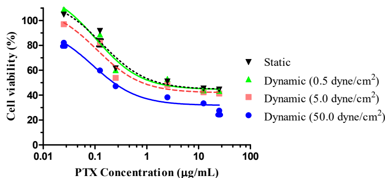
Figure 7. Cell viability of A549 cells treated with PTX-GONs under different cell culture conditions incubated for 24 h (data are expressed as mean \pm SD for triplicate experiments, n = 6 ).
