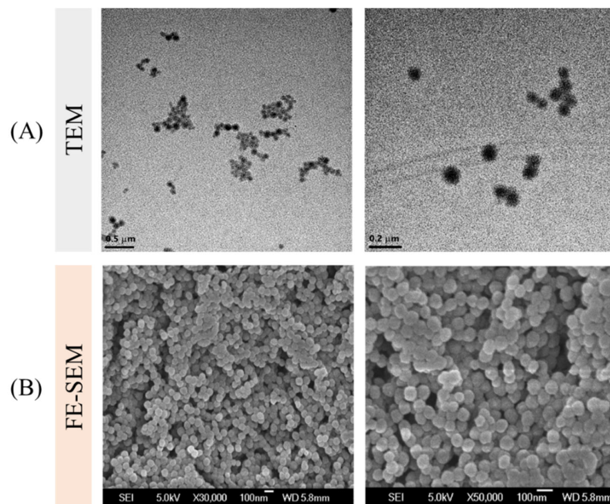
Figure 3. Electron microscopy images of GONs at two different magnifications ( \times 30K and \times 50K ): (A) TEM and (B) FE-SEM.
