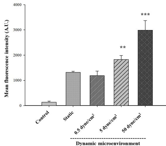
Figure 5. Cellular uptake of C-GONs by A549 cancer cells under a static or biomimetic dynamic microenvironment for 1 h (mean \pm SD; n = 3 , ** p < 0.01 ; *** p < 0.001 ).
