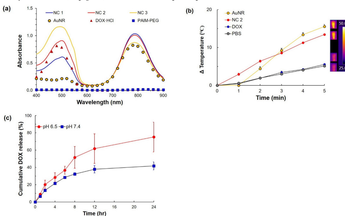
Figure 2. Photothermal effect: (a) absorption spectra, (b) heat generation by NIR laser (AuNR 1 µg/mL, 808 nm, 2.0 W/cm 2 ), and (c) DOX release at different pH conditions (pH 7.4 and 6.5).
