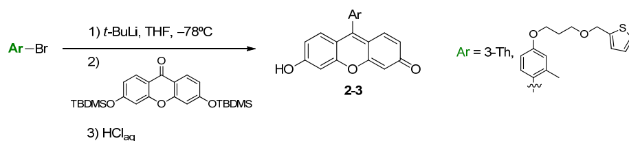
Scheme 2. Synthetic route of compounds 2–3.
