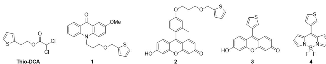
Chart 1. DCA-based drug Thio-DCA and thiophene-containing fluorescent dyes (acridone 1 , xanthene 2–3 , and BODIPY 4 ) synthesized in this work.
