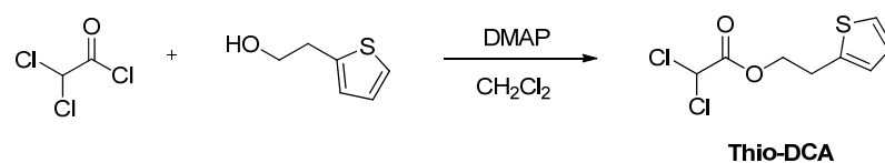
Scheme 3. Synthesis of Thio-DCA.
