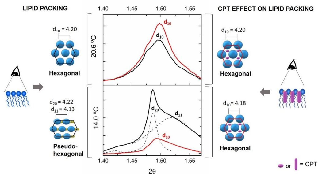
Figure 7. Wide angle X-ray diffraction (WAXS) patterns of DMPC (black) or DMPC containing CPT (red) measured in the L_{\beta'} ( 14.0 \text{ }^\circ\text{C} ) and P_\beta ( 20.6 \text{ }^\circ\text{C} ) phases of DMPC. Solid lines give the best fit of the Lorentzian's analysis model (dashed lines) to the scattered intensities. A model of drug-membrane interaction is proposed for each diffractogram together with the resultant d_s values.
