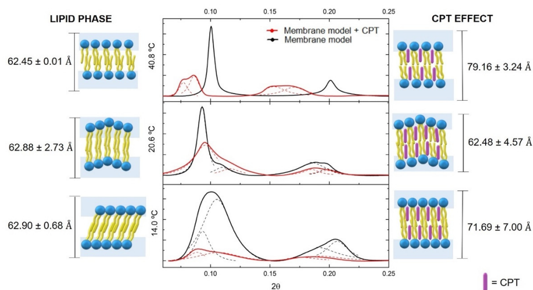
Figure 6. Small angle X-ray diffraction (SAXS) patterns of DMPC (black) or DMPC containing CPT (red) measured in the L_{\beta}' (14.0 °C), P_{\beta} (20.6 °C), and L_{\alpha} (40.8 °C) phases of DMPC. Solid lines give the best fit of the Lorentzian's analysis model (dashed lines) to the scattered intensities. A model of the drug–membrane interaction is proposed for each diffractogram, together with the resultant d_L values.
