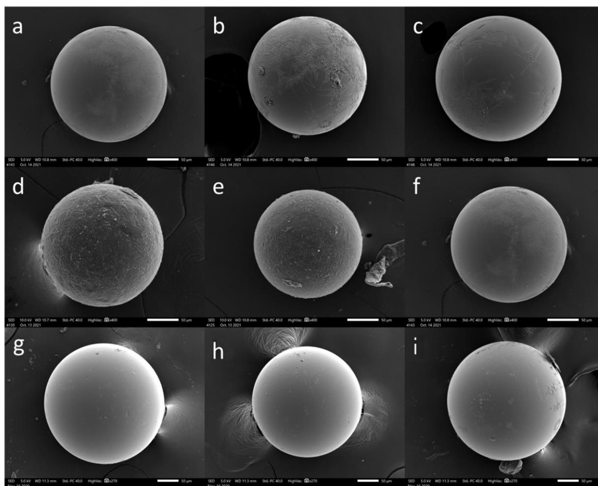
Figure 5. API particles printed on an aluminum surface. SEM images of (a–c) paracetamol, (d–f) carbamazepine, and (g–i) indomethacin microparticles. Scale bars: 50 \mu\text{m} .
