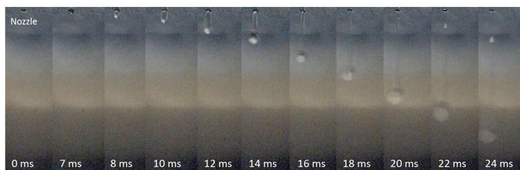
Figure 3. Melt-jet printing process paradigm: a sequence of images (from left to right) captured with a high-speed digital camera, showing the ejection of a molten paracetamol droplet from the nozzle (top) on an aluminum surface (bottom).
