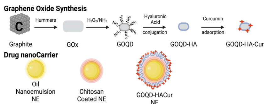
Scheme 1. Synthesis steps of multistage nanocarrier.
