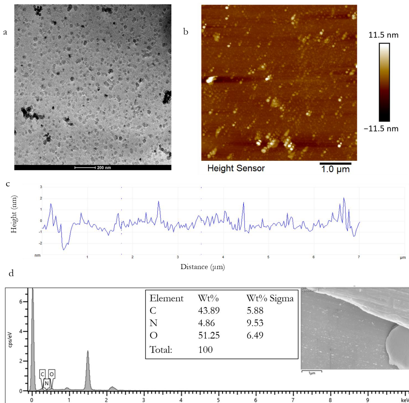
Figure 1. GOQDs-HA morphology and size evaluation, (a) cryo-TEM image, (b) AFM image, (c) height profile, and (d) EDX spectrum.
