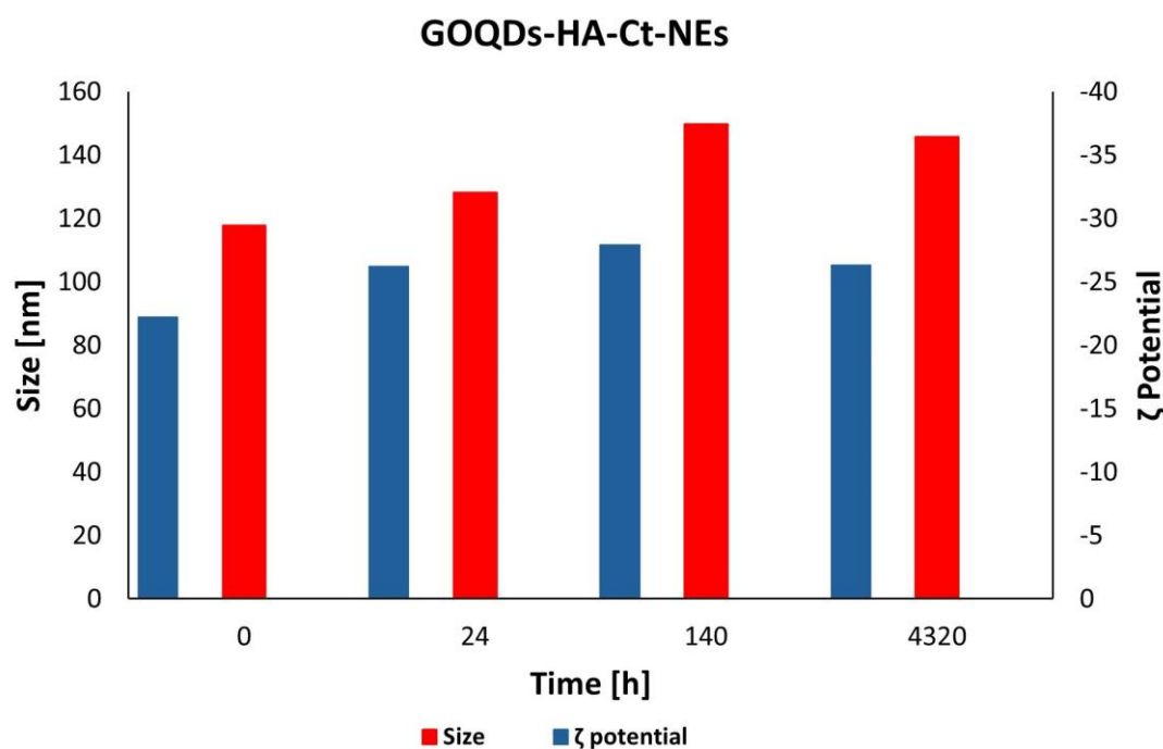
Figure 5. Size and \zeta potential time stability of GOQDs-HA-CT-NEs.
