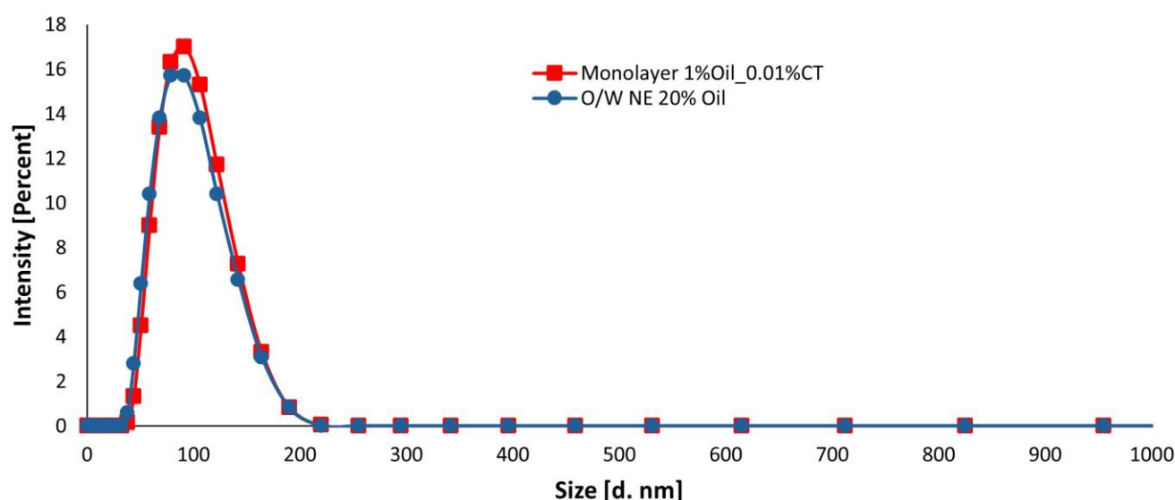
Figure 4. DLS size distribution of O/W NE 20% oil and monolayer 1%Oil_0.01%CT.
