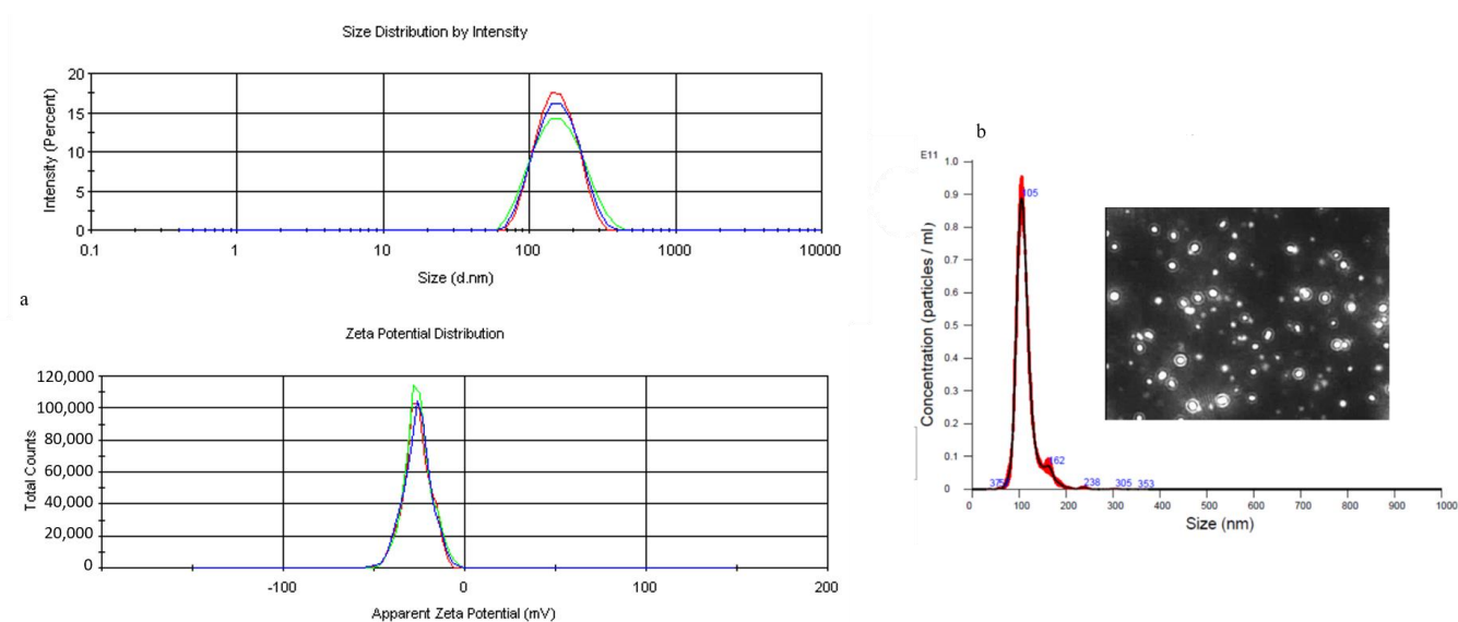
Figure 6. (a) DLS size distribution and \zeta potential bilayer CT-GOQDs-HA after 180 days; (b) NTA size distribution and frame of nanoparticles detected by NTA camera (insert).
