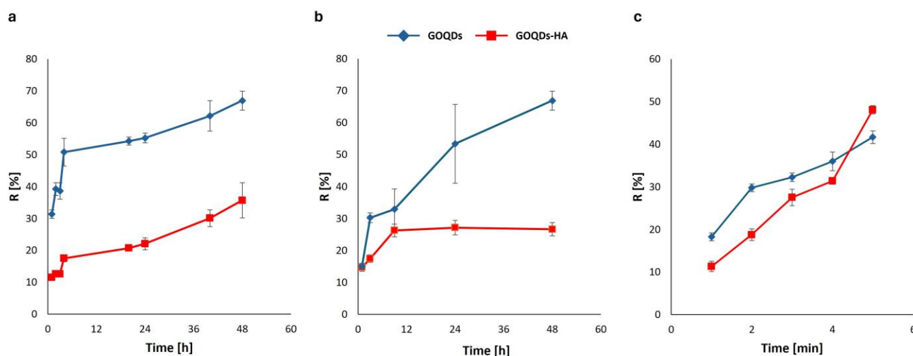
Figure 3. Cur release from GOQDs-NH 2 and GOQDs-HA at (a) 37 °C in PBS Buffer pH 7.4, (b) at 37 °C in PBS Buffer pH 5.5, and (c) at 60 °C in PBS buffer pH 7.4.
