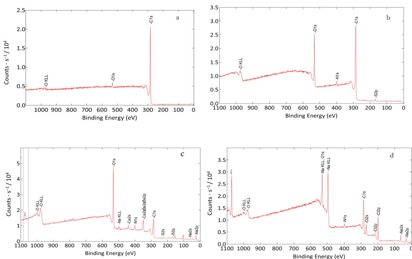
Figure 2. XPS survey spectra of (a) graphite; (b) GO Humder ; (c) GOQDs-NH 2 ; (d) GOQDs-HA.
