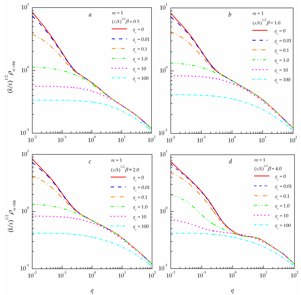
Figure 6. Integral coherence scale \rho_{m vbb} of partially coherent vortex Bessel beams ( m = 1 ) propagating in a turbulent atmosphere at the different source coherence q_c for four values of the Bessel beam parameter \tilde{\beta} : (a) \tilde{\beta} = 0.5 ; (b) \tilde{\beta} = 1.0 ; (c) \tilde{\beta} = 2.0 ; (d) \tilde{\beta} = 4.0 .
