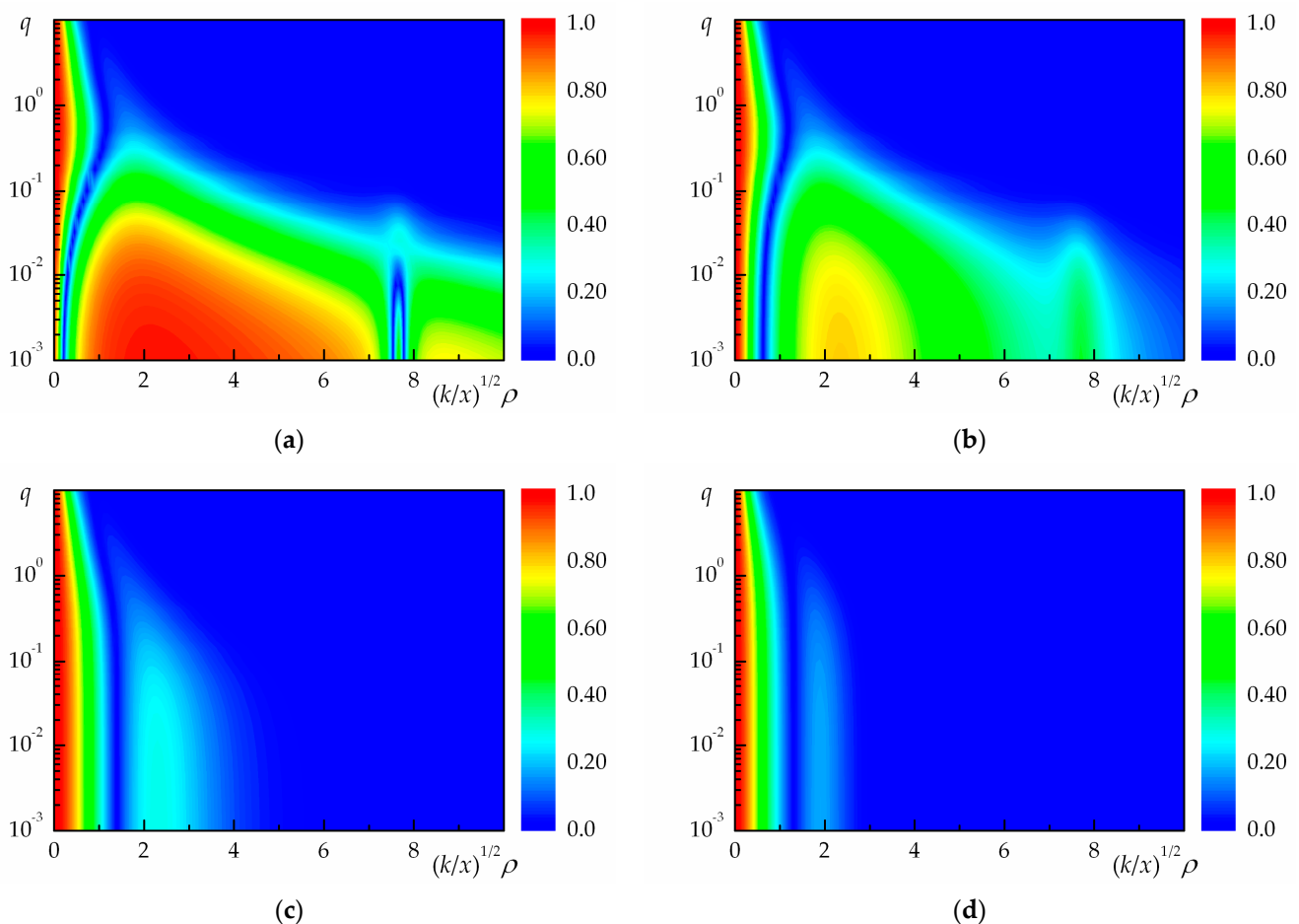
Figure 3. Coherence degree \mu_{vbb}(x, \rho) of partially coherent vortex Bessel beams propagating in a turbulent atmosphere at \tilde{\beta} = 1.0 and m = 1 for different values of the dimensionless parameter q_c : (a) q_c = 0.01 ; (b) q_c = 0.1 ; (c) q_c = 1.0 ; (d) q_c = 10.0 .
