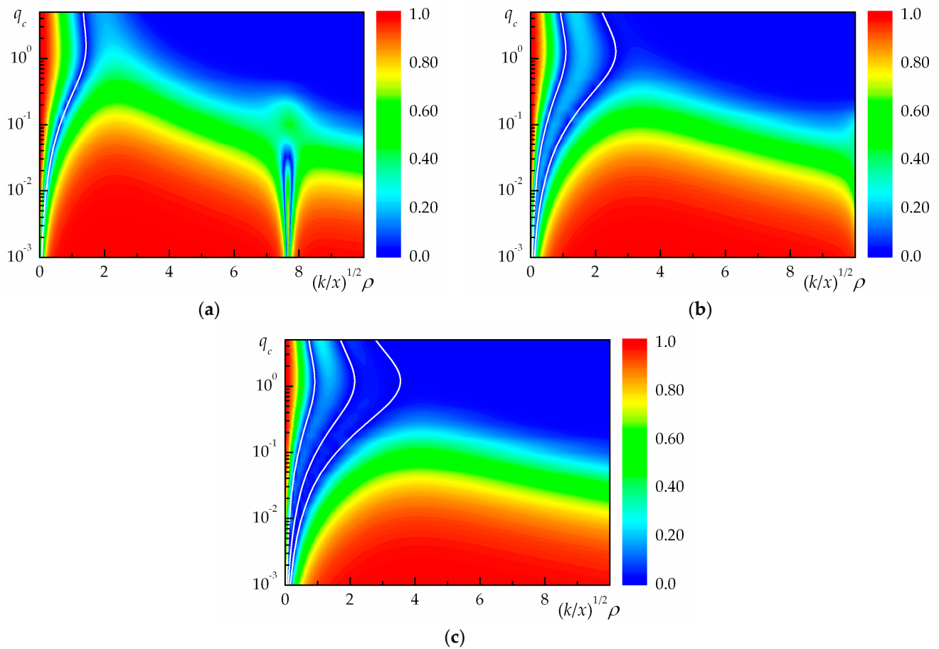
Figure 1. Coherence degree \mu_{vbb}(x, \rho) of partially coherent vortex Bessel beams propagating in a uniform medium at \tilde{\beta} = 1.0 for different values of the topological charge of the vortex beam m : (a) m = 1 ; (b) m = 2 ; (c) m = 3 . The white curves represent the coordinates of a ring dislocation.
