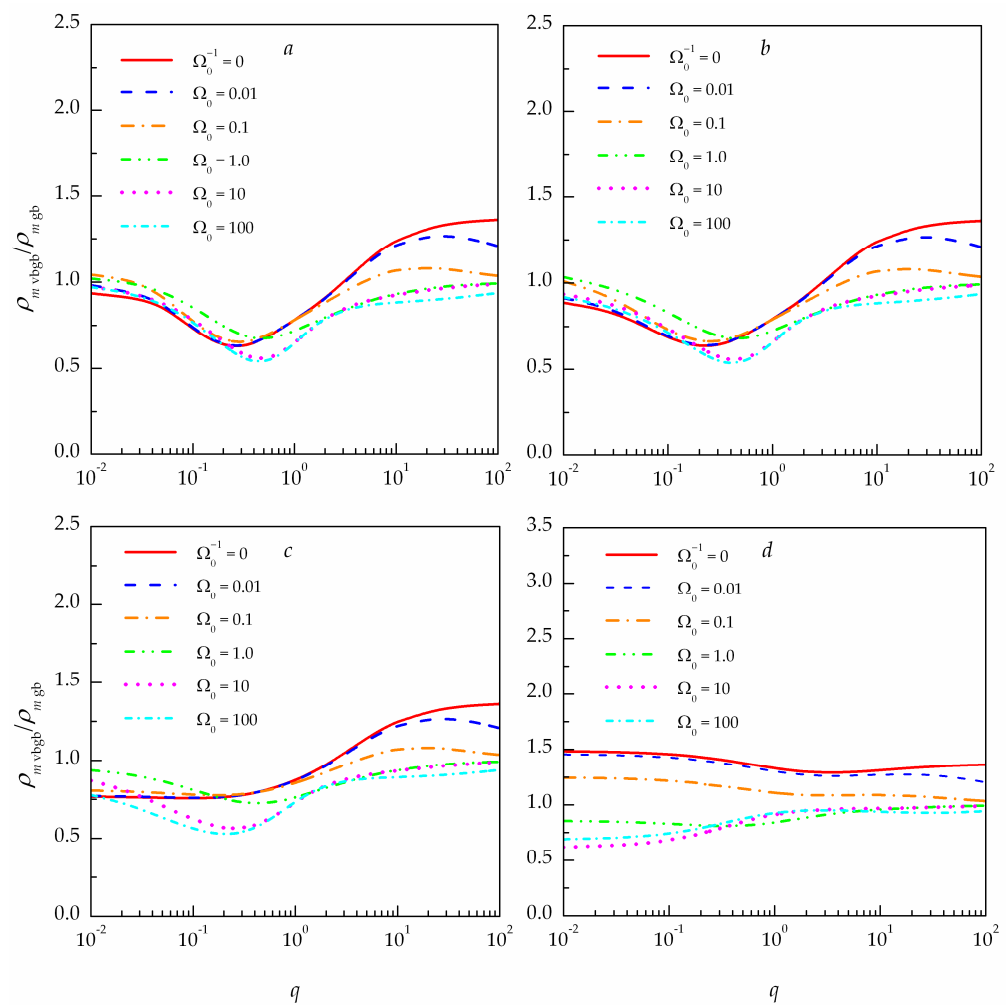
Figure 7. Ratio of the integral coherence scales of partially coherent vortex Bessel–Gaussian \rho_{m,vbgb} and Gaussian \rho_{m,gb} beams with \tilde{\beta} = 1.0 and m = 1 at different values of the Fresnel number of the transmitting aperture \Omega_0 for three source coherence levels q_c : (a) q_c = 0 ; (b) q_c = 0.1 ; (c) q_c = 1.0 ; (d) q_c = 10.0 .
