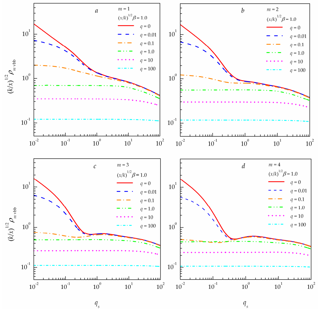
Figure 5. Integral coherence scale \rho_{m vbb} of partially coherent vortex Bessel beams propagating in a turbulent atmosphere at different turbulence level q in the propagation medium for four values of the topological charge of vortex beam m : (a) m = 1 ; (b) m = 2 ; (c) m = 3 ; (d) m = 4 .
