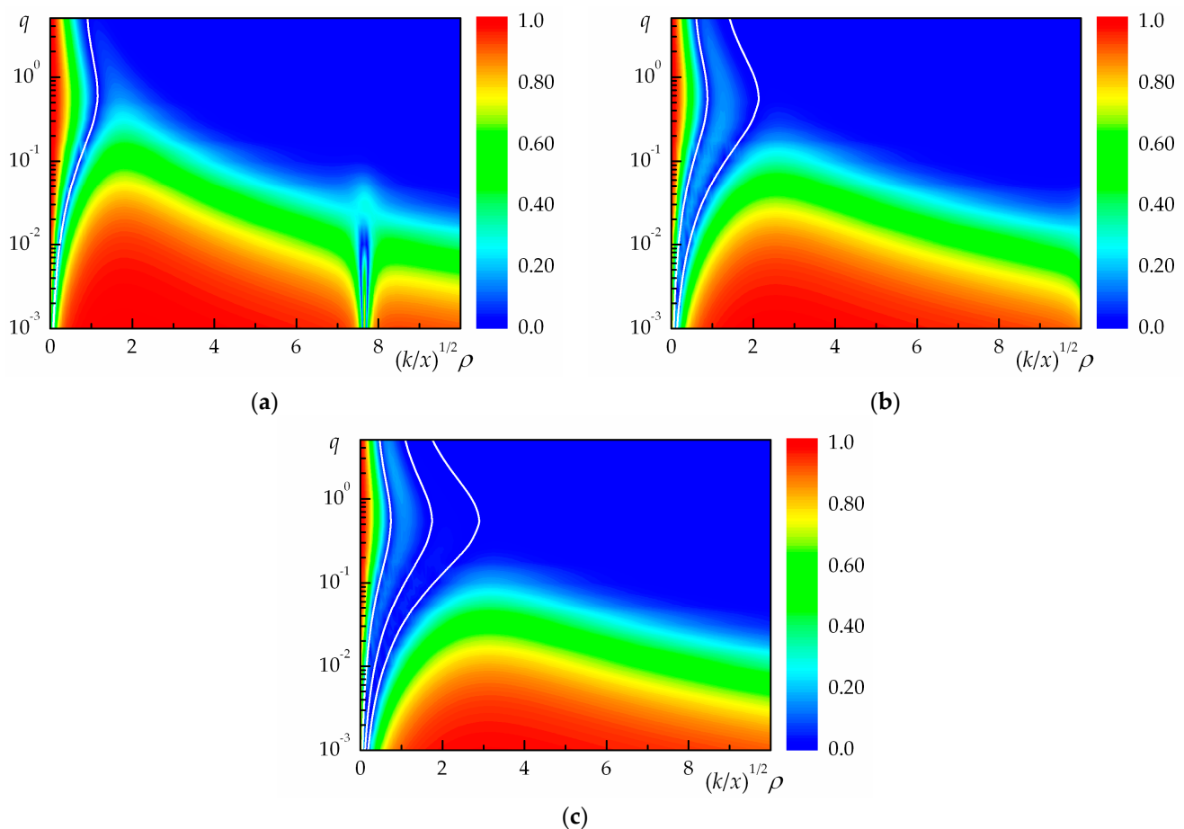
Figure 2. Coherence degree \mu_{vbb}(x, \rho) of coherent vortex Bessel beams propagating in a turbulent atmosphere at \beta = 1.0 for different values of the topological charge of the vortex beam m : (a) m = 1 ; (b) m = 2 ; (c) m = 3 . The white curves represent the coordinates of a ring dislocation.
