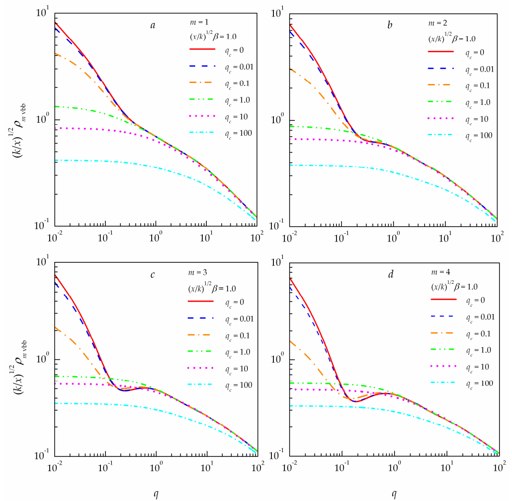
Figure 4. Integral coherence scale \rho_{m vbb} of partially coherent vortex Bessel beams propagating in a turbulent atmosphere at different source coherence levels q_c for four values of the topological charge of the vortex beam m : (a) m = 1 ; (b) m = 2 ; (c) m = 3 ; (d) m = 4 .
