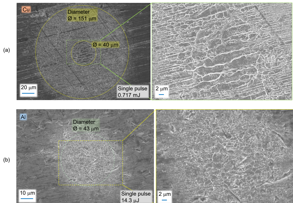
Figure 4. SEM images of single-pulse ablation sites (see Figure 3a) at high (a) and low (b) pulse energies on coupons of Cu (a) and Al (b), respectively. The focal spot size is \sim 60 \text{ μm} .
