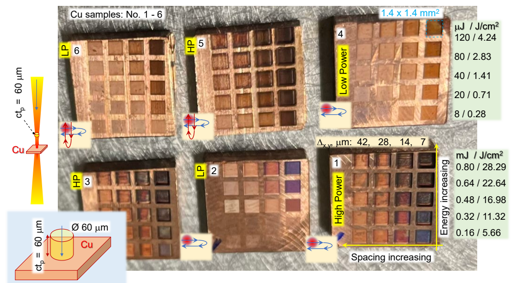
Figure 2. Typical 1 \times 1 \text{ cm}^2 Cu coupon samples used to determine ablation rates. Samples were not polished. High and low power ranges were used to explore the different surface roughness and material removal rates of the ablated surfaces (see pulse energy E_p and fluence F_p [\text{J/cm}^2] ). F-theta lens had focal diameter on the sample 2r = 60 \mu\text{m} , depth of focus \text{DoF} = 2.7 \text{ mm} , field of scan 50 \times 50 \text{ mm}^2 , and axial pulse extent of ct_p = 60 \mu\text{m} for pulse duration of t_p = 200 fs. The melting temperature of Cu is 1085^\circ\text{C} , evaporation/boiling point is 2595^\circ\text{C} . For samples Nos. 1 and 2, the focal spot was placed 6 mm deeper along the beam propagation direction from the top surface of the sample. Hatching passes in X-/Y-directions are shown schematically; the total number of passes was always 10.
