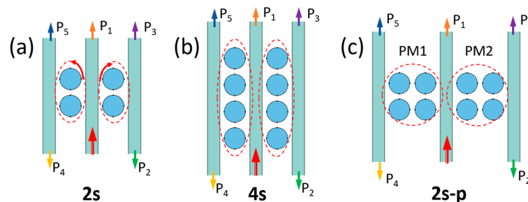
Figure 2. Structural types of PM-based optical splitters with (a,b) serial (2s and 4s) and (c) serial–parallel (2s-p) electromagnetic coupling of atoms in photonic molecules PM1 and PM2 (outlined
