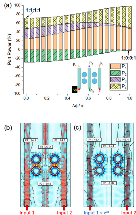
Figure 8. (a) Dependence of relative power in the optical ports of optical coupler on the left port dephasing \Delta\phi . (b,c) Poynting vector streamlines in the 2s PM coupler at (b) \Delta\phi = 0 and (c) \Delta\phi = \pi radians at 1339.4 nm bonded supermode resonance.
