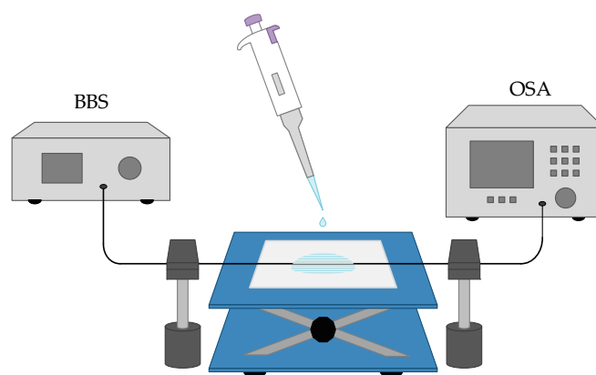
Figure 6. Schematic illustration of the experimental setup.
