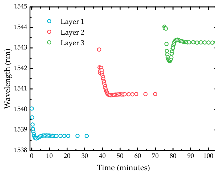
Figure 4. Wavelength evolution during the drying process of three layers of chitosan, measured for the filter dip at around 1540 nm.
