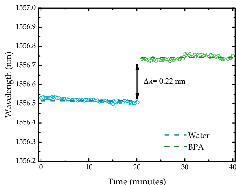
Figure 8. Wavelength stability, using distilled water and a 0.01 mg/mL BPA solution, determined for the coated sensor.
