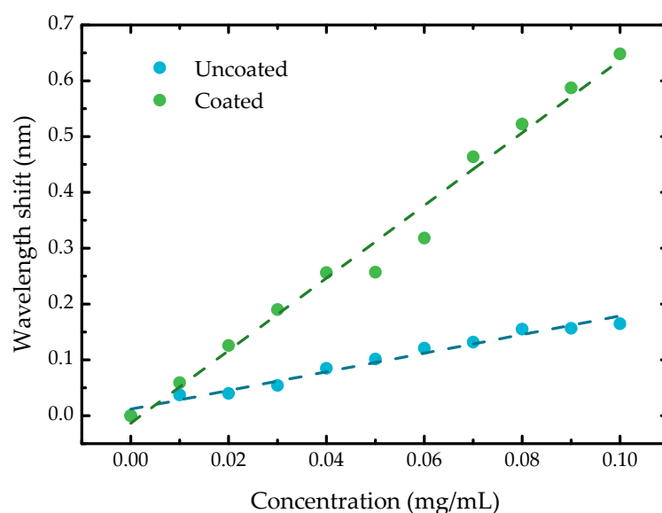
Figure 7. Wavelength shift with increasing concentrations of BPA, expressed in mg/mL, determined for the uncoated and coated sensor.
