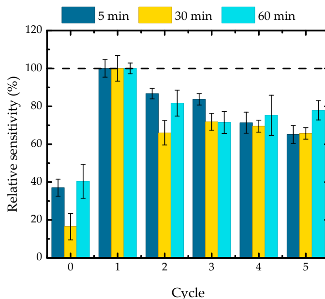
Figure 9. Relative sensitivity of 5 measurement cycles, obtained for the washing assays with a 70% (v/v) methanol solution, under different exposure times. Cycle 0 represents the relative sensitivity of the uncoated sensor.
