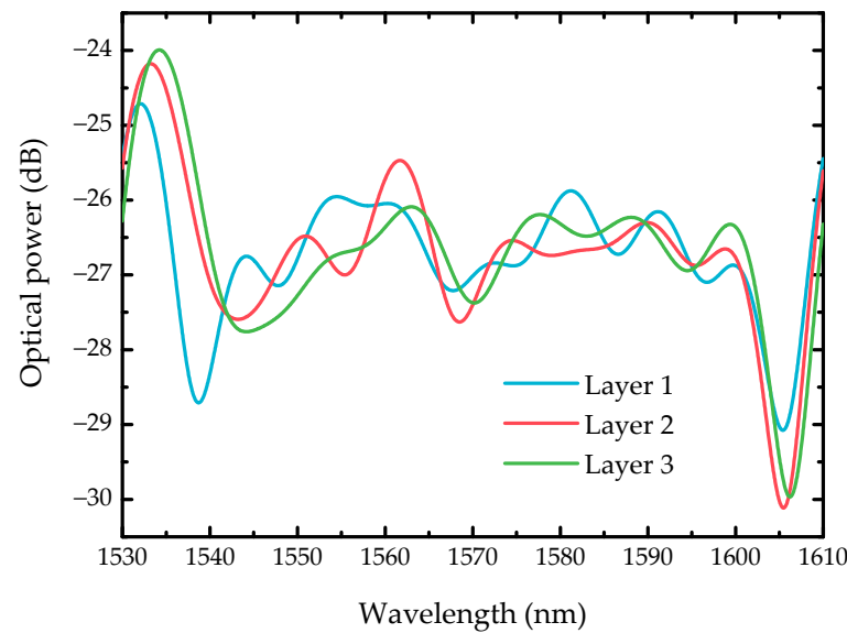
Figure 3. Band pass filter of the chitosan-coated sensor, in air, acquired immediately after each coating procedure.
