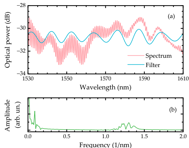
Figure 2. (a) Spectral response of the sensor submerged in water with the corresponding band pass filter between 0.07 and 0.12 nm −1 ; (b) FFT of the spectrum.
