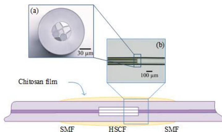
Figure 1. Schematic illustration of the sensing structure, consisting of a section of HSCF between two SMFs and subsequently coated with three layers of chitosan. Microscope photographs of the (a) microstructured fiber cross-section, and (b) sensor, in the splice region.
