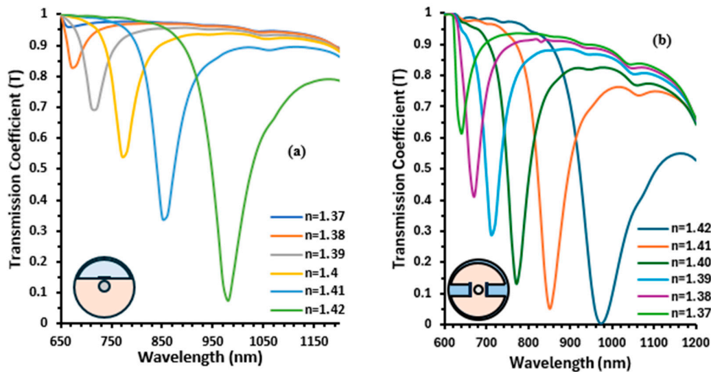
Figure 2. Transmission spectrum for (a) D-shaped SPR sensor; (b) \pi -shaped SPR sensor.
