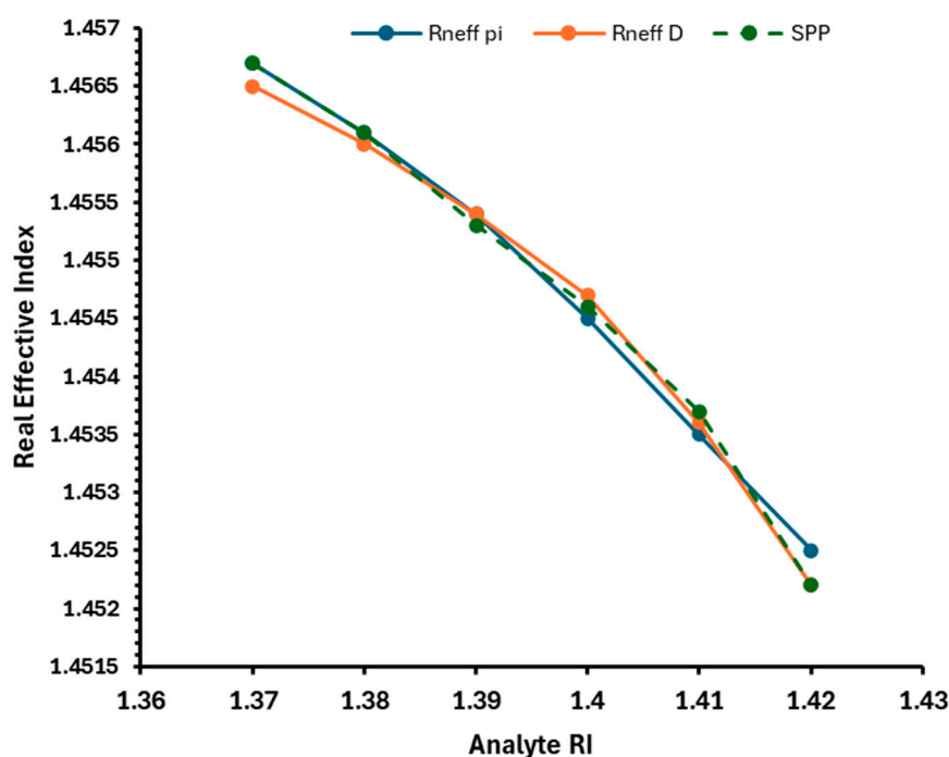
Figure 3. Phase matching plot showing Re(n_{SPP}) and Re(n_{eff}) for D-shaped and \pi -shaped SPR sensors.
