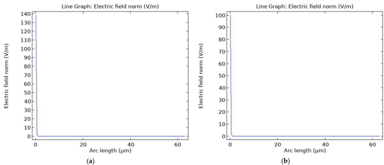
Figure 6. Graph of electric field norm vs. arc length for (a) \pi -configuration; (b) D-shaped sensor.
