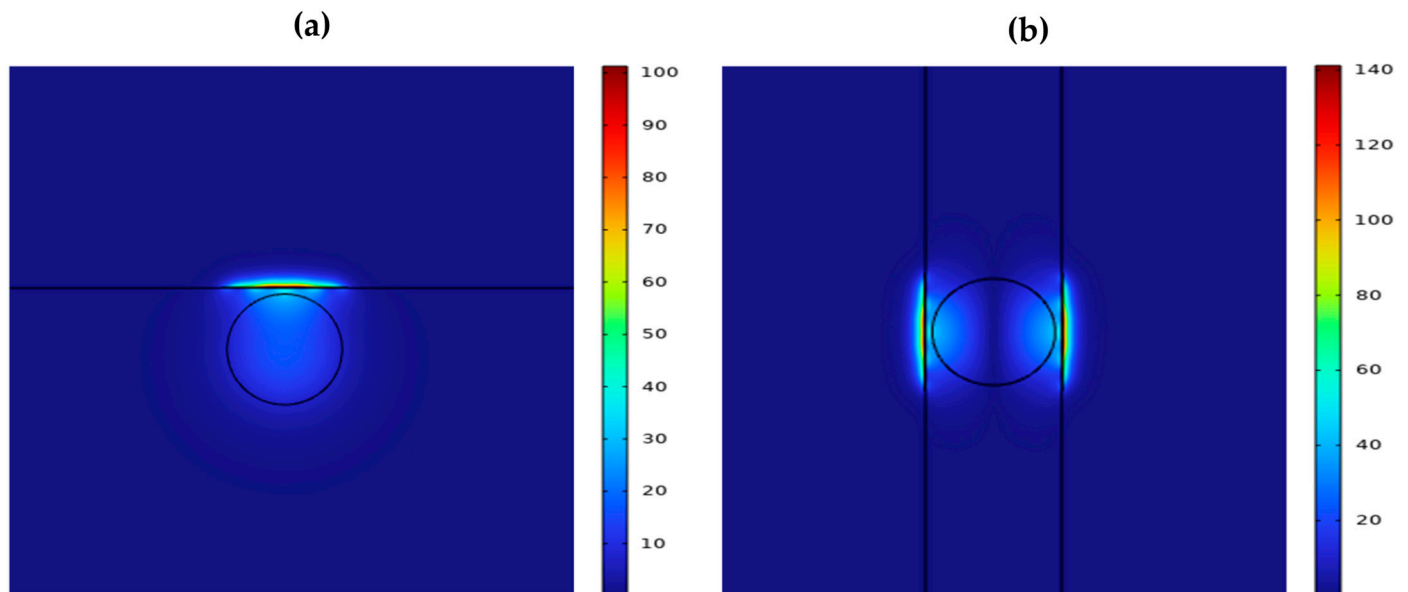
Figure 5. Electric field distribution for (a) D-shaped SPR mode; (b) \pi -config SPR mode.
