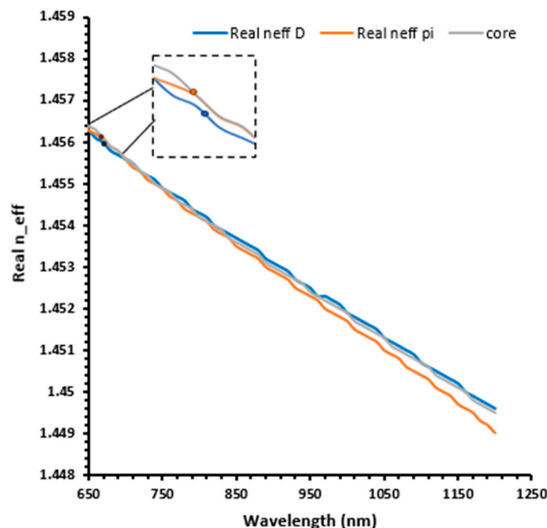
Figure 4. Dispersion relations for the core ( HE_{11} ) mode, D-shaped SPP mode, and \pi -hybridized SPP mode at RI = 1.38.
