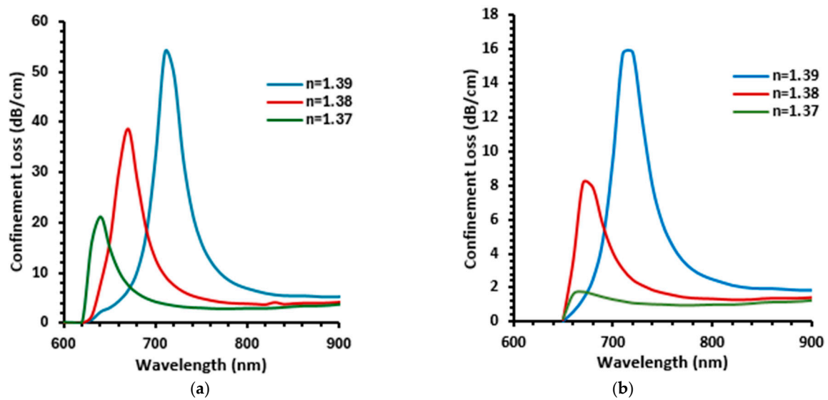
Figure 7. Confinement loss spectra for (a) \pi -configuration; (b) D-shaped sensor.
