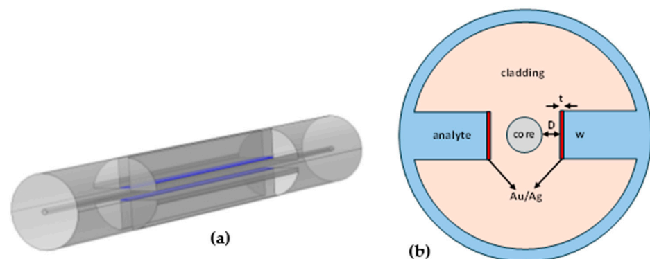
Figure 1. (a) The 3D schematic of \pi -config D-SPR sensor; (b) sensor design in 2D with core design parameters (residual cladding thickness D = 700 nm, the metal film width w = 10 \mu\text{m} , and the metal film thickness t = 45 nm).
