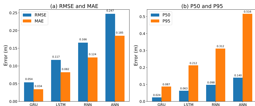
Figure 6. Training performance of recurrent models with PCA-based dimensionality reduction in the SCENE_VLP framework. Lower values indicate better accuracy (in meters).
