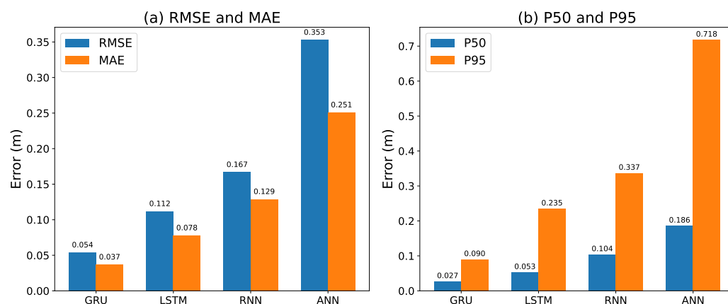
Figure 7. Training performance of recurrent models with DAE-based latent feature extraction in the SCENE_VLP framework. Lower values represent better accuracy (in meters).
