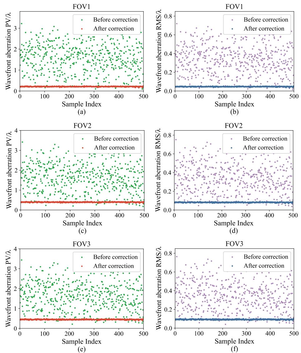
Figure 11. Scatter plots of wavefront aberrations before and after correction based on CNN-FCNN. (a,c,e) respectively represent the comparison of wavefront aberration PV of 500 groups of samples in three FOVs before and after correction. Green dots represent the distribution of wavefront aberration PV before correction, and red dots represent the distribution of wavefront aberration PV after correction. (b,d,f) respectively represent the comparison of wavefront aberration RMS of 500 groups of samples in three FOVs before and after correction. Purple dots represent the distribution of wavefront aberration RMS before correction, and blue dots represent the distribution of wavefront aberration RMS after correction. .
