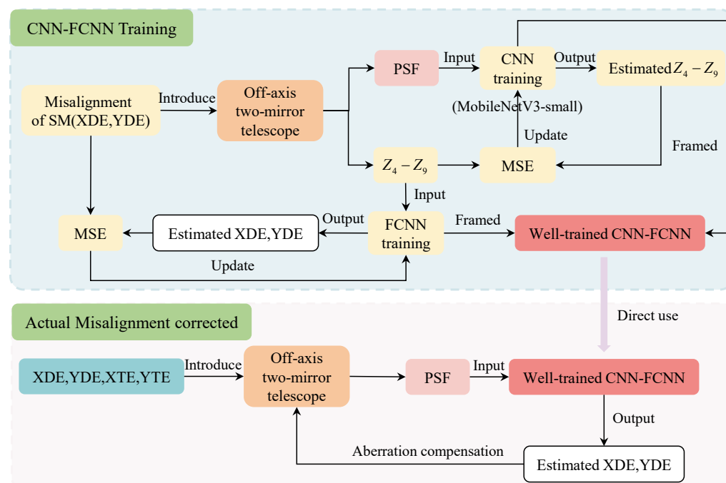
Figure 5. Flow chart of the misalignment-induced aberration compensation method based on fusion of focal spot images and Zernike polynomial coefficients.
