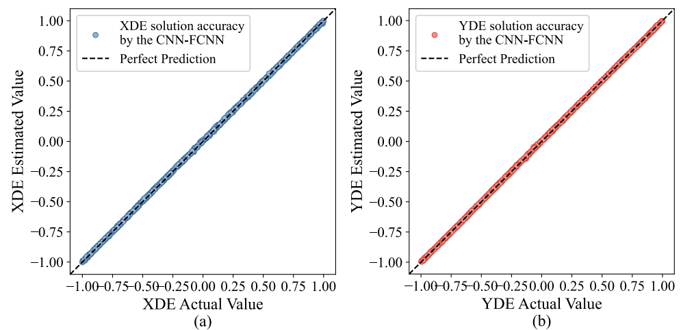
Figure 8. Comparison between estimated and actual misalignment value obtained by CNN-FCNN (abscissa: actual misalignment value, ordinate: estimated misalignment value, dashed line represents ideal fitting line y = x ). (a) Scatter plot of X-axis decenter error solution accuracy; (b) Scatter plot of Y-axis decenter error solution accuracy.
