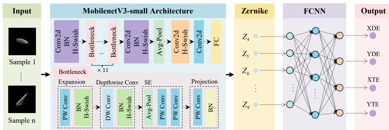
Figure 6. Schematic diagram of model training based on MobileNetV3-Small and FCNN.
