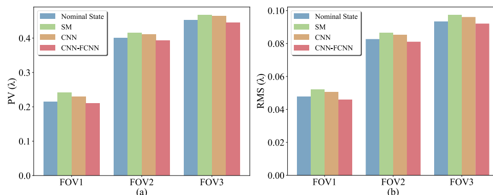
Figure 10. Comparison of wavefront correction effects by three methods. (a) Comparison of wavefront aberration PV values of three FOVs under SM, CNN, CNN-FCNN misalignment correction and nominal design states (b) Comparison of wavefront aberration RMS values of three FOVs under SM, CNN, CNN-FCNN misalignment correction and nominal design states.
