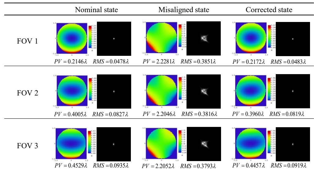
Figure 12. Misalignment correction effect.
