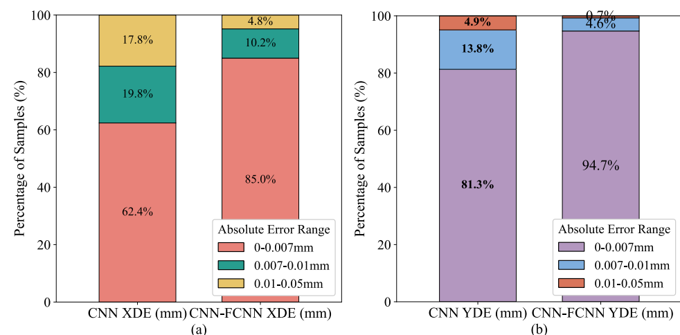
Figure 9. Comparison of absolute error ratio distributions of misalignment solutions by two methods. (a) Comparison of absolute error percentages of X-axis decenter error solution based on CNN and CNN-FCNN. (b) Comparison of absolute error percentages of Y-axis decenter error solution based on CNN and CNN-FCNN.
