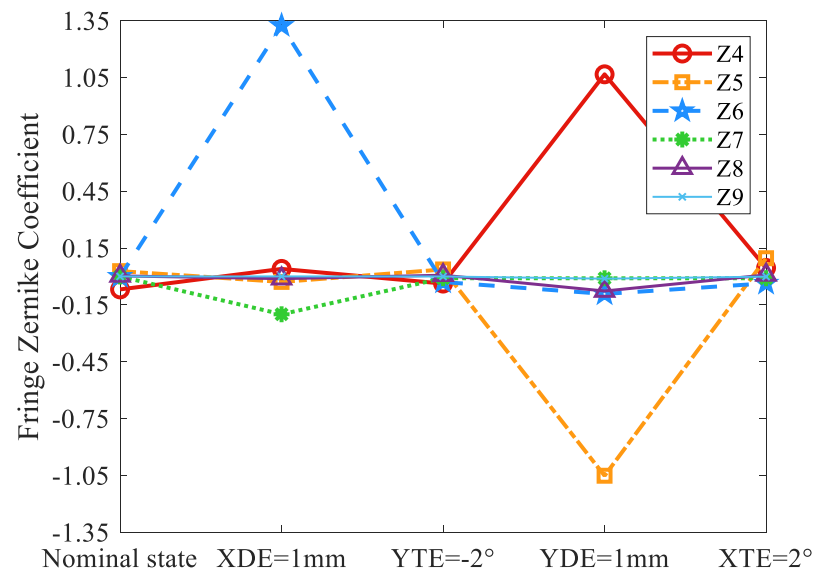
Figure 2. System aberration coupling caused by changes in misalignment values.
