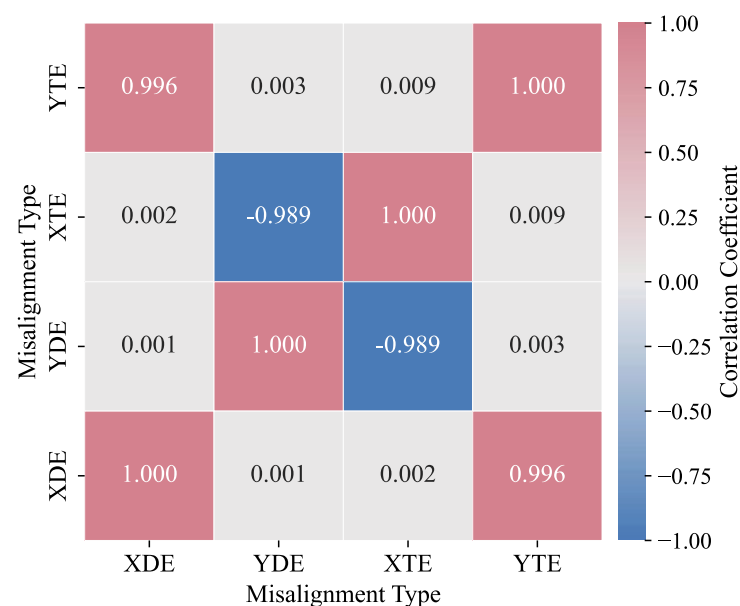
Figure 3. Correlation coefficient matrix of different misaligned DOFs.
