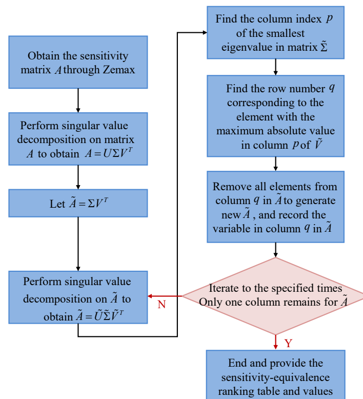
Figure 4. Sensitivity analysis flow using SVD-based mode truncation algorithm.
