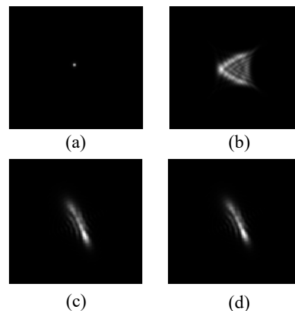
Figure 1. PSF morphology approximation due to misalignments coupling. (a) Spot image under nominal state; (b) Spot image under misaligned state; (c) Misaligned state: XDE = -0.251 mm, YDE = 0.704 mm, XTE = 0.486^\circ , YTE = -0.299^\circ ; (d) Misaligned state: XDE = -0.331 mm, YDE = 0.607 mm, XTE = 0.296^\circ , YTE = -0.154^\circ .
