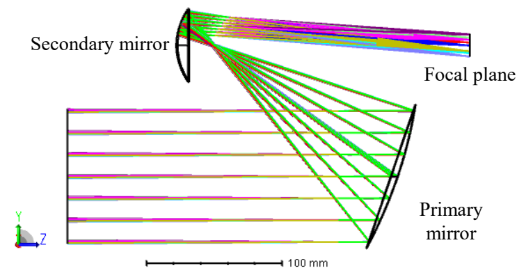
Figure 7. The optical layout of the off-axis two-mirror telescope system.
