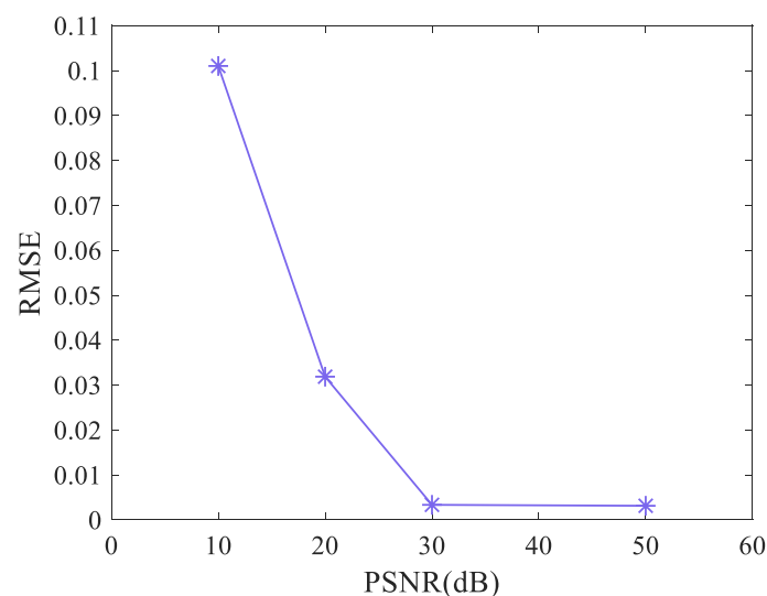
Figure 13. The relationship between the misalignment correction accuracy of the proposed CNN-FCNN method and the noise level.
