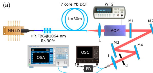
Figure 2. (a) Scheme of a Yb-doped multicore fiber pulsed laser: MM LD—multi-mode laser diode; HR FBG—fs-inscribed high-reflective FBG; L—collimating lens; M1—90% reflecting mirror, M2—M3—dichroic mirrors; OSA—optical spectrum analyzer; OSC—oscilloscope; PD—photodiode module; AOM—acousto-optic modulator; WFG—waveform generator; d—diaphragm. (b) Output pulse train at an LD pump power of 1.4 W and repetition rate of 1 kHz.
