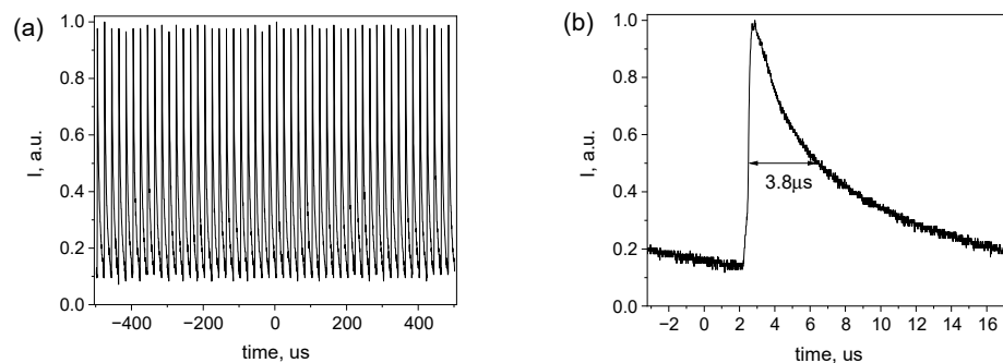
Figure 7. Train of pulses at a repetition frequency of 50 kHz (a) and corresponding optical pulse shape (b).
