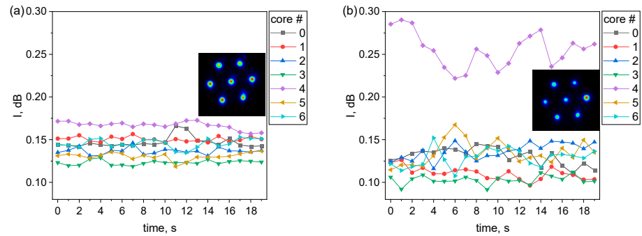
Figure 6. Dynamics of power distribution across the cores at 1.4 W (a) and 1.7 W (b) pumping.
