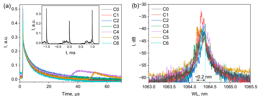
Figure 4. Output laser pulses (a) and optical spectra (b) at pump power of 1.7 W and rep. rate of 1 kHz.
