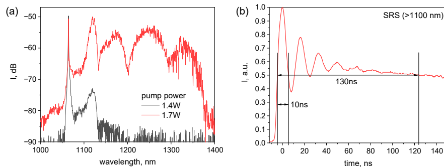
Figure 5. Output optical spectra at different powers (a) and the SRS pulse component at pump power of 1.7 W (b).
