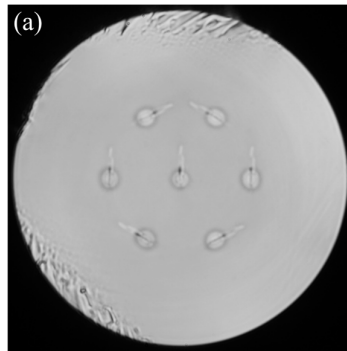
Figure 1. Fiber cross-section with fs-inscribed highly reflective (HR) FBGs (a) and individual FBG reflection spectra of the 7-core FBG array (C0-central, C1–C6 peripheral) (b).
