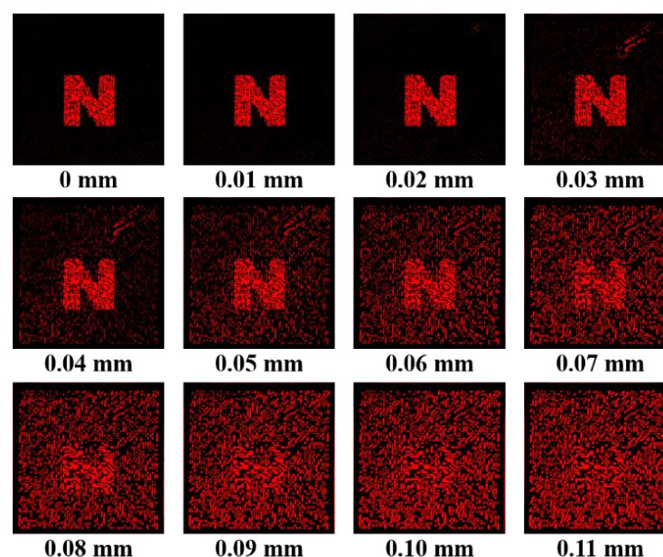
Figure 7. Decrypted images under different lateral translations.
