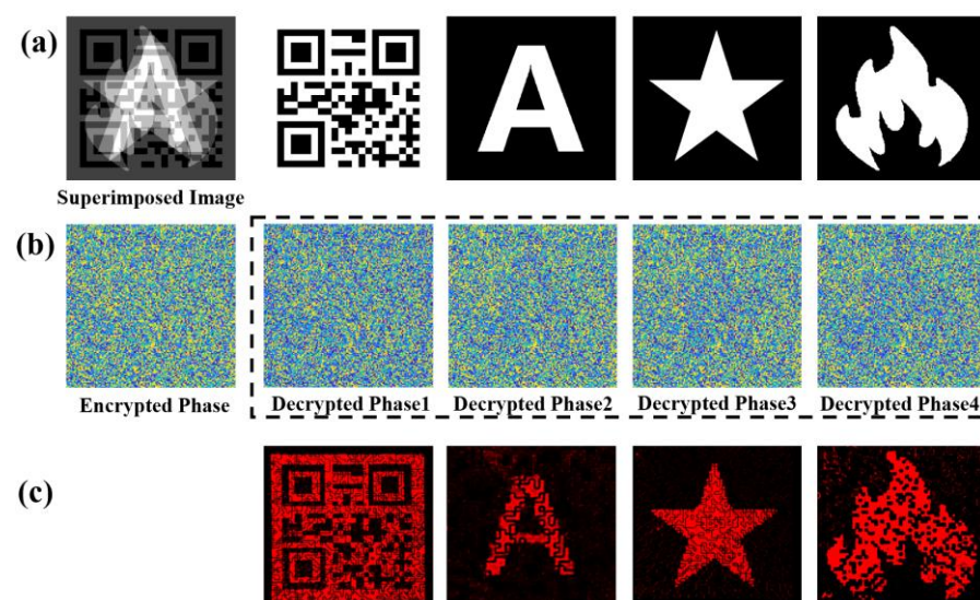
Figure 5. Schematic diagram of the multi-image integrated encryption principle: (a) integration of multiple two-gray-level images to form a mixed image; (b) generation of an encryption phase, and several decryption phases for target images; (c) experimental results of reconstructed images.
