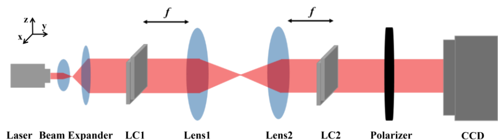
Figure 3. Schematic diagram of the optical path for the encryption with cascaded LC elements, where LC1 and LC2 are the encryption and decryption liquid crystal elements, respectively.
