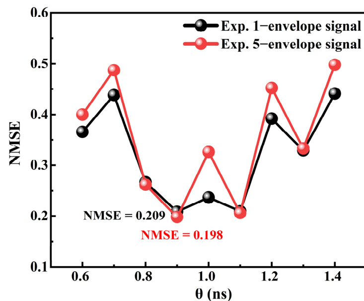
Figure 4. NMSE as a function of the virtual node interval \theta (ranging from 0.6 ns to 1.4 ns) using the two mask signals (Exp. 1-envelope signal and Exp. 5-envelope signal).
