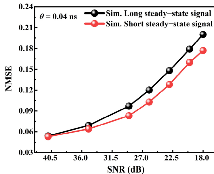
Figure 8. NMSE as a function of the SNR (ranging from 41 dB to 18 dB) for the Santa Fe time-series prediction task with \theta = 0.04 ns, where additive Gaussian white noise of varying amplitude is injected into the two mask signals. The black curves correspond to Sim. Long steady-state signal, while the red curves correspond to Sim. Short steady-state signal.
