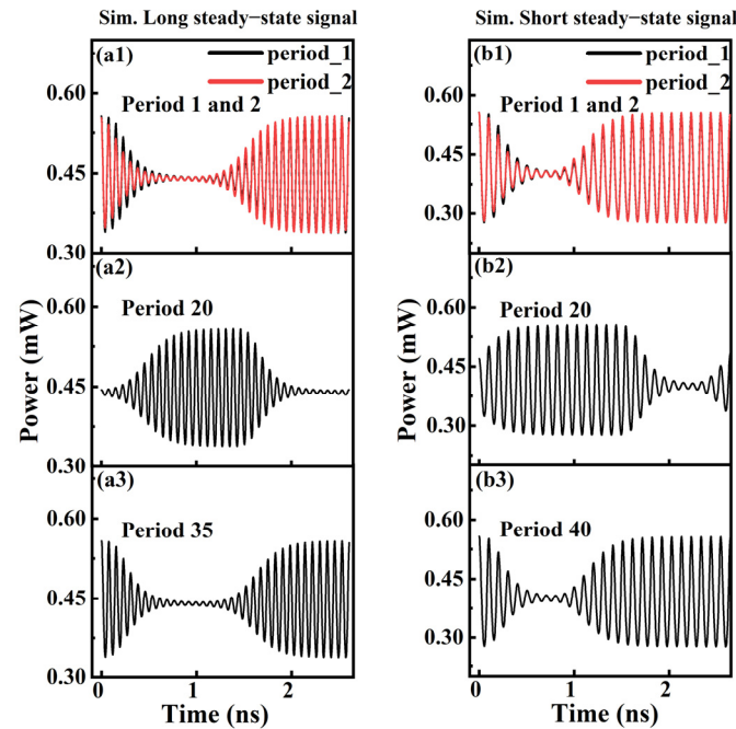
Figure 6. Time series of two noise-free simulated S-QPS signals for different periods: (a1) overlay of the first and second periods, (a2,a3) the 20th and 35th periods of Sim. Long steady-state signal; (b1) overlay of the first and second periods, (b2,b3) the 20th and 40th periods of Sim. Short steady-state signal.
