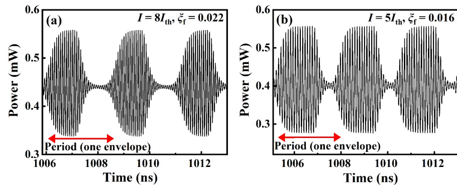
Figure 5. S-QPS states of an SL-OF under noise-free conditions with an external-cavity round-trip time of \tau_f = 2.5 ns: (a,b) simulated time series at I = 8I_{th} , \xi_f = 0.022 and I = 5I_{th} , \xi_f = 0.016 , respectively.
