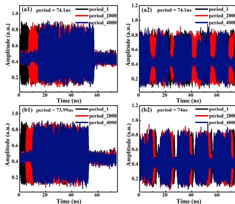
Figure 3. Overlay of representative periods extracted from the experimental time series for the Exp. 1-envelope signal and Exp. 5-envelope signal. The 1st, 2000th, and 4000th periods are shown to compare long-term period consistency. (a1,a2) Period overlays using a period of 74.1 ns; (b1,b2) Period overlays using period of 73.99 ns (for Exp. 1-envelope signal) and 74.0 ns (for Exp. 5-envelope signal).
