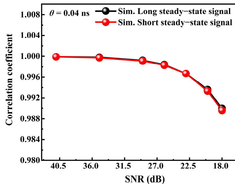
Figure 9. Correlation coefficient as a function of the SNR (ranging from 41 dB to 18 dB) for the Santa Fe time-series prediction task with \theta = 0.04 ns, where additive Gaussian white noise of varying amplitude is injected into the two mask signals. The black curves correspond to the Sim. Long steady-state signal, while the red curves correspond to the Sim. Short steady-state signal.
