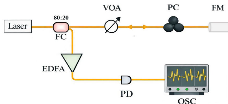
Figure 1. Experimental setup of the S-QPS signal generation. FC: fiber coupler; VOA: variable optical attenuator; PC: polarization controller; FM: fiber mirror; EDFA: erbium-doped fiber amplifier; PD: photodetector; OSC: oscilloscope.
