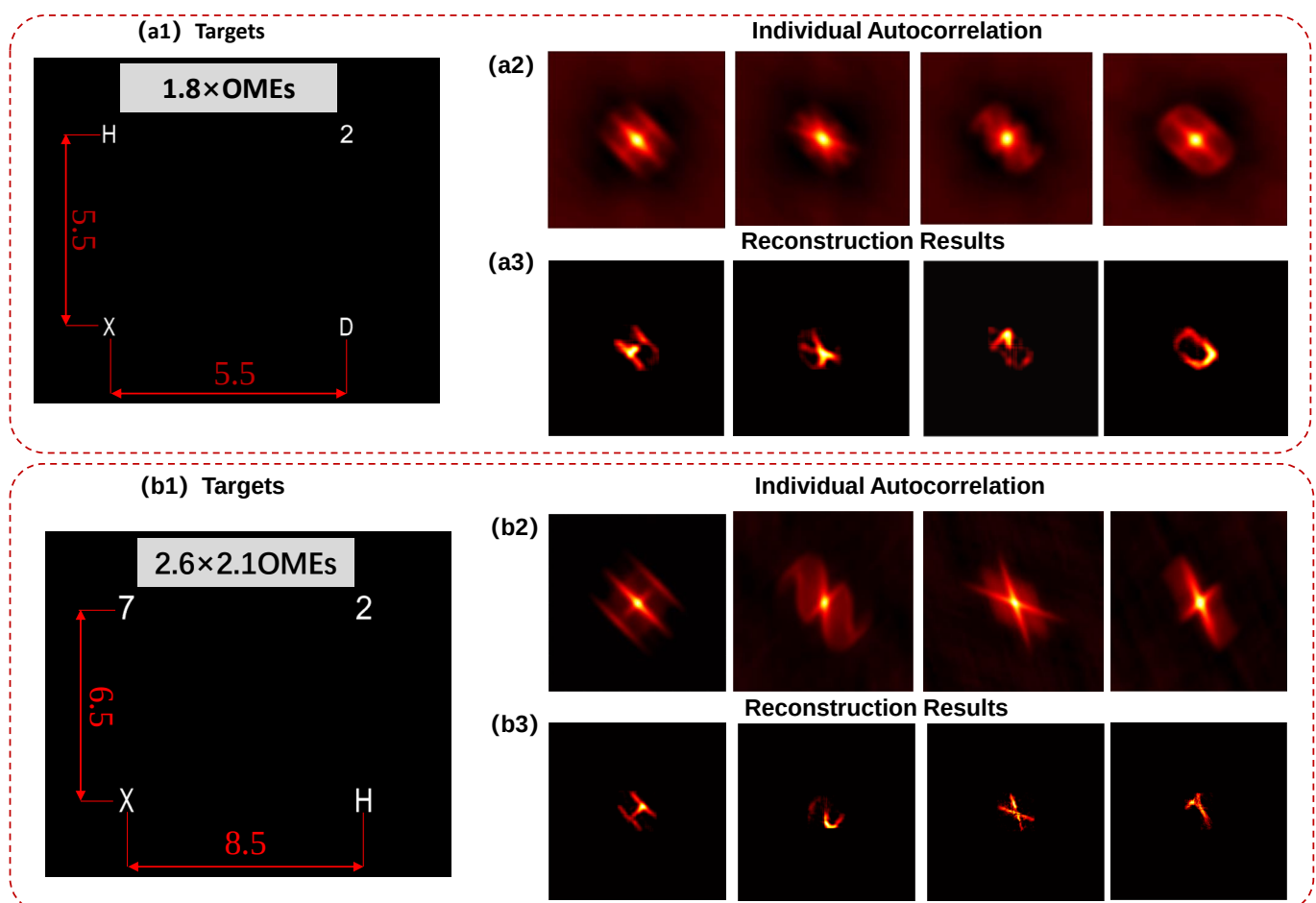
Figure 4. Comparative imaging results under different OME conditions. (a1–a3) Target configuration at 1.8 times the OME range, the corresponding individual target auto-correlations, and reconstructed target images. (b1–b3) Target configuration with increased separations, the corresponding autocorrelations and reconstructed target images.
