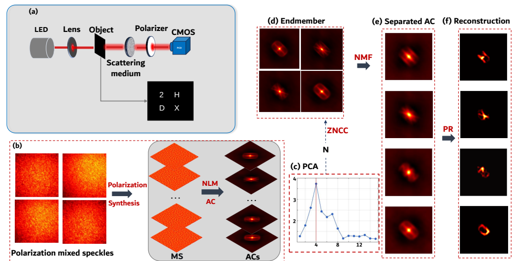
Figure 1. Schematic illustration of the process of the proposed method for realizing noninvasive scattering imaging of multiple targets beyond the OME. (a) Transmissive imaging configuration. (b–f) The data processing of the polarization demixing method. MS denotes the multi-angle synthesized speckles; ACs denotes the corresponding autocorrelations of the synthesized speckles.
