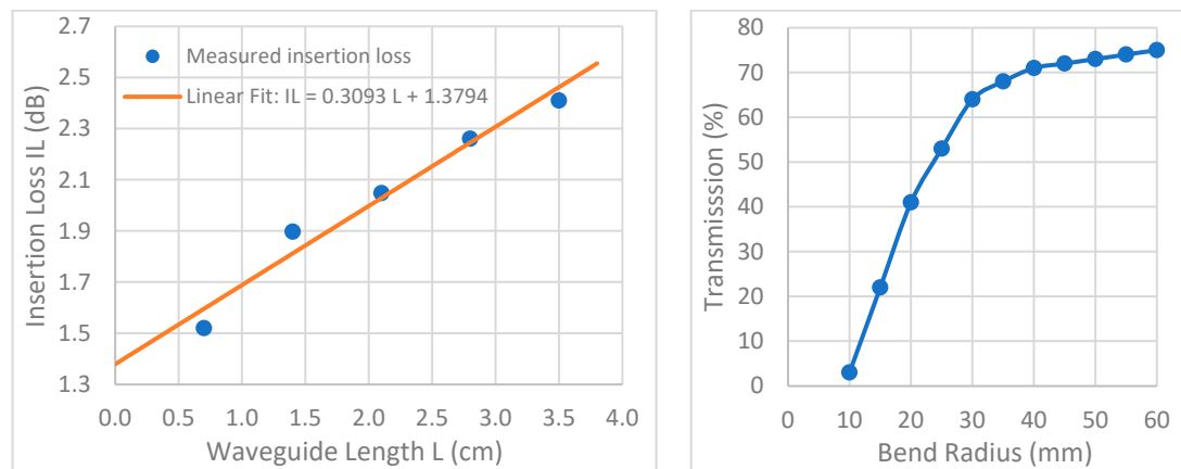
Figure 8. Optical loss characterization of stress-assisted waveguides in BF33 borosilicate glass. (Left) insertion loss as a function of waveguide length measured using the cut-back method at 808 nm. The solid line represents a linear fit; its slope was used to estimate the propagation loss. The fit intercept contains length-independent loss contributions, including input/output coupling losses, Fresnel reflections, facet quality, mode mismatch, and alignment uncertainty, and should therefore not be interpreted as a pure coupling loss. (Right) measured transmission as a function of bend radius for waveguides fabricated with the selected BF33 writing parameters.
