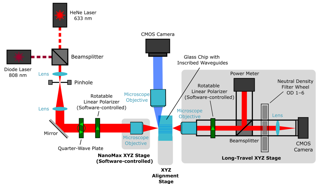
Figure 5. Schematic of the optical and thermo-optic characterization setup. The setup enables end-fire coupling, polarization control, near-field mode imaging, transmission measurements, and characterization of thermo-optic phase shifters integrated into Mach–Zehnder interferometers.
