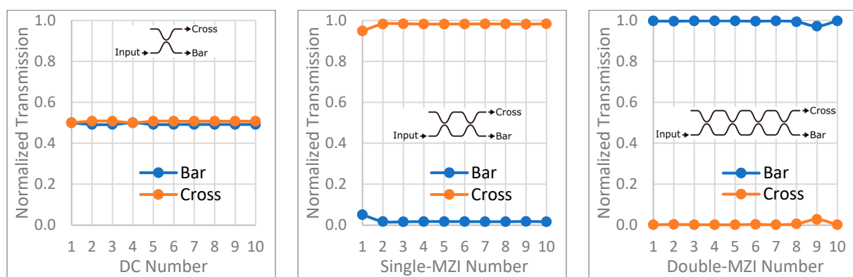
Figure 10. Device-to-device consistency of interferometric building blocks fabricated in BF33. Results are shown for ten nominally identical directional couplers, Mach–Zehnder interferometers, and cascaded double-MZI structures fabricated on the same test chip.
