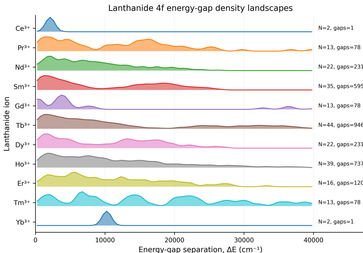
Figure 2. Ridgeline visualization of the normalized energy-gap distributions for the \text{Ln}^{3+} ions considered in this work. Each profile was constructed from non-zero internal gaps generated from the corresponding energy-only manifold. The values to the right indicate the number of multiplet-centre energies, N , and the number of non-zero pairwise gaps used for each ion. Continuous profiles are used exclusively as visual guides for the underlying binned distributions; all numerical descriptors were calculated from unsmoothed normalized histograms.
