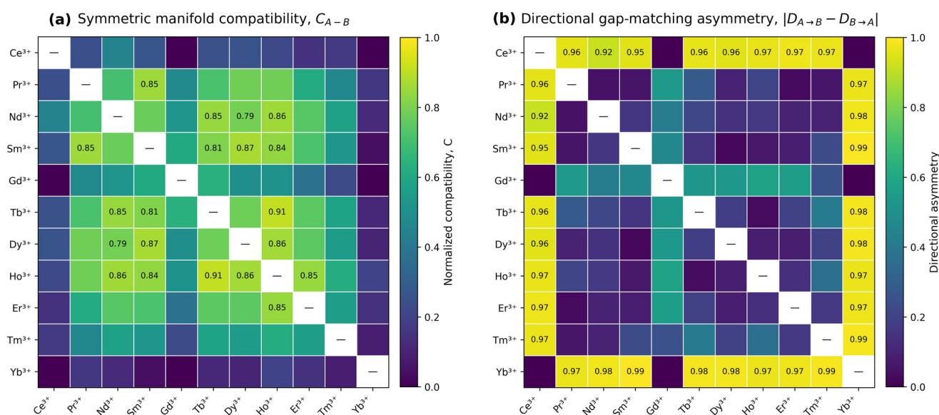
Figure 3. Pairwise \text{Ln}^{3+} – \text{Ln}^{3+} descriptor matrices. (a) Symmetric manifold-compatibility matrix C_{A-B} , measuring global overlap between normalized gap distributions. (b) Directional gap-matching asymmetry matrix |D_{A \rightarrow B} - D_{B \rightarrow A}| , highlighting pairs for which gap inclusion is strongly directional.
