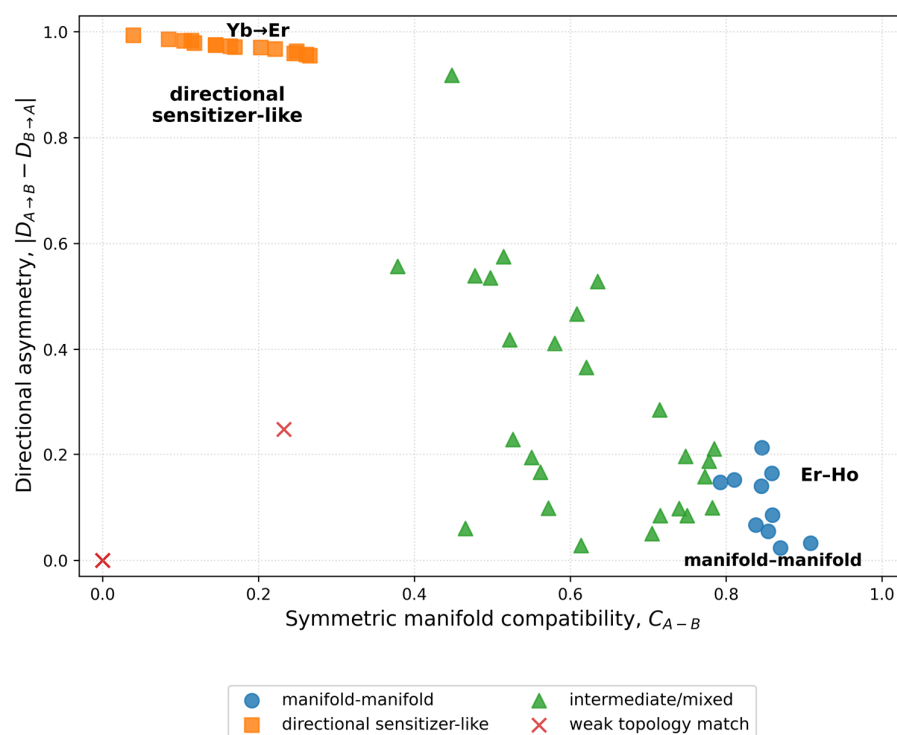
Figure 4. Coupling-architecture map obtained by combining symmetric manifold compatibility with directional gap-matching asymmetry. High- C_{A-B} , low-asymmetry pairs define the manifold–manifold region, whereas low- C_{A-B} , high-asymmetry pairs define directional sensitizer-like architectures. Pairs located between these limiting regions are shown as intermediate/mixed, whereas low-compatibility pairs without strong directional inclusion are shown as weak topology matches. \text{Er}^{3+} – \text{Ho}^{3+} and \text{Yb}^{3+} \rightarrow \text{Er}^{3+} are shown as representative examples of the two limiting regimes. The labelled regions are interpretive guides within the present \text{LaF}_3 -based dataset and do not represent universal decision boundaries or direct assignments of experimental transfer mechanisms.
