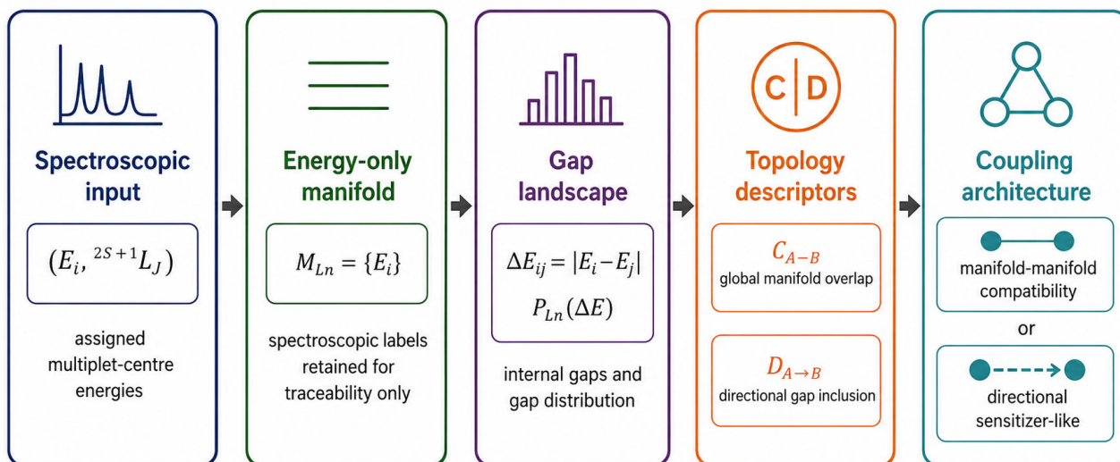
Figure 1. Energy-gap topology workflow for mapping \text{Ln}^{3+}\text{--Ln}^{3+} coupling architectures. Assigned multiplet-centre energies are reduced to energy-only manifolds, from which internal gaps and gap distributions are constructed. The complementary descriptors C_{A\rightarrow B} and D_{A\rightarrow B} are then used to distinguish broad manifold–manifold compatibility from directional sensitizer-like coupling.
