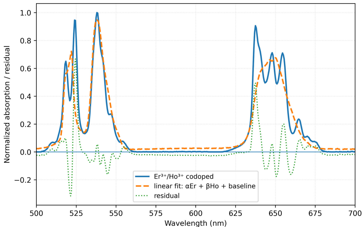
Figure 5. Linear-combination test of the \text{Er}^{3+}/\text{Ho}^{3+} co-doped absorption spectrum in the shared visible window. The baseline-corrected and normalized \text{Er}^{3+}/\text{Ho}^{3+} absorption spectrum between 500 and 700 nm is compared with the best linear combination of the Er-only and Ho-only reference spectra, A_{\text{ErHo}}(\lambda) \approx \alpha A_{\text{Er}}(\lambda) + \beta A_{\text{Ho}}(\lambda) + B(\lambda) . The fit gives R^2 = 0.841 , with \alpha = 0.705 and \beta = 0.902 , indicating that the co-doped absorption response in this region is better described by the combined contribution of both \text{Er}^{3+} and \text{Ho}^{3+} manifolds than by either single-ion contribution alone. The residual highlights the remaining spectral mismatch. This analysis is included as an illustrative multicomponent absorption example and is not used to validate the topology descriptors or to measure \text{Er}^{3+} \leftrightarrow \text{Ho}^{3+} energy-transfer efficiency.
