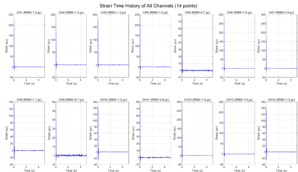
Figure 17. Time-history strain responses of the 14 measurement points.
