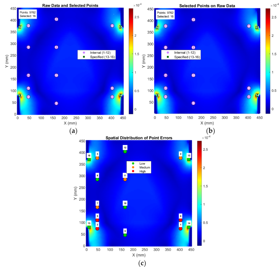
Figure 12. Optimal sensor placement of the CFRP plate under dynamic loading: (a) original dynamic response data; (b) optimized sensor placement scheme; (c) error analysis of the optimized sensor placement scheme.
