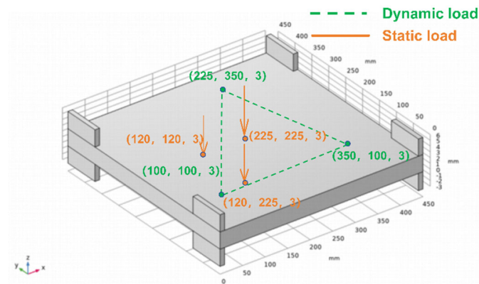
Figure 1. CFRP plate model constructed in COMSOL.
