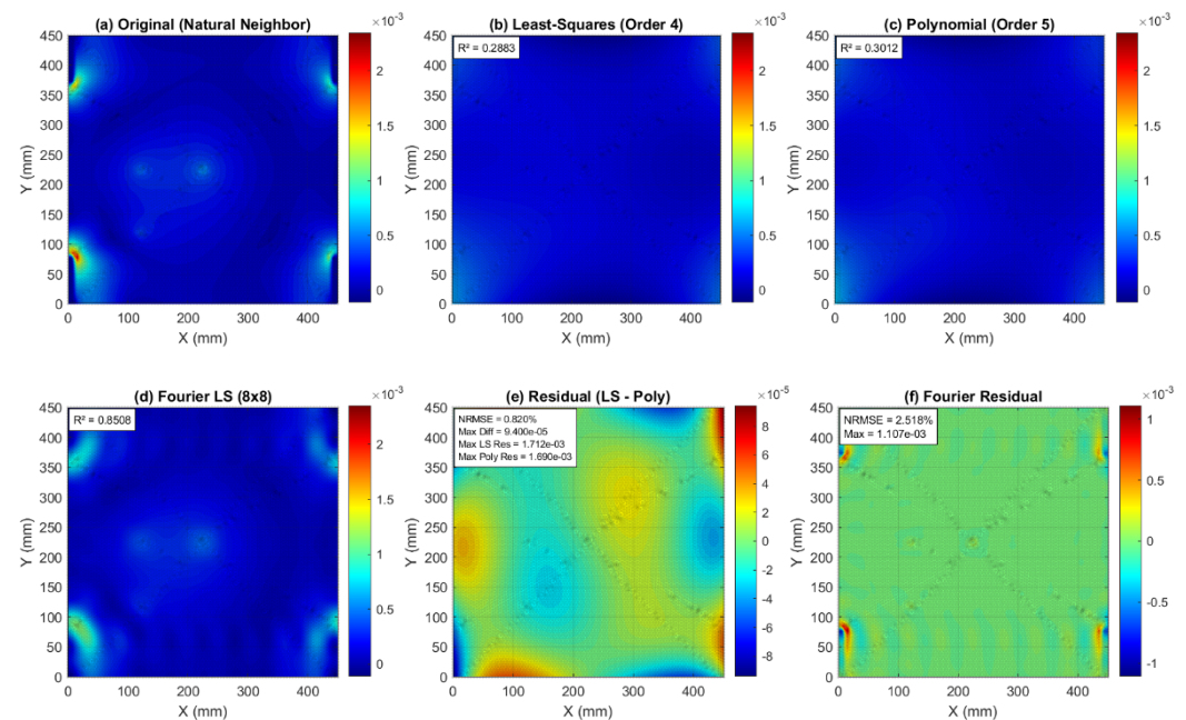
Figure 4. Case under static loading: (a) original strain field; (b) strain field reconstructed using least-squares fitting; (c) strain field obtained by polynomial fitting; (d) strain field reconstructed using Fourier least-squares fitting; (e) residual comparison between least-squares fitting and polynomial fitting; (f) residual distribution of Fourier series fitting.
