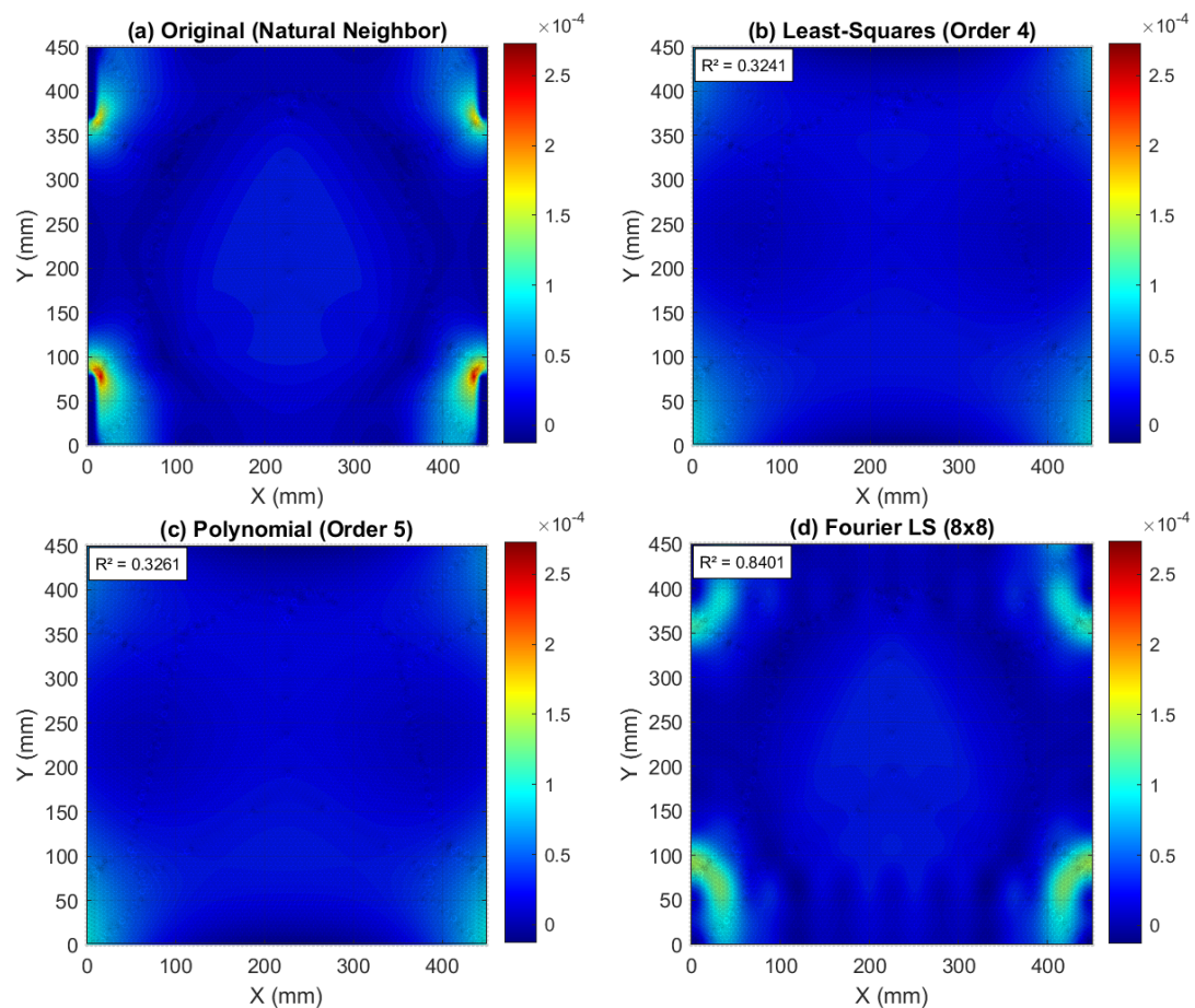
Figure 7. Strain distributions under dynamic loading: (a) original strain contour map; (b) least-squares fitted strain contour map; (c) polynomial-fitted strain contour map; and (d) Fourier least-squares fitted strain contour map.
