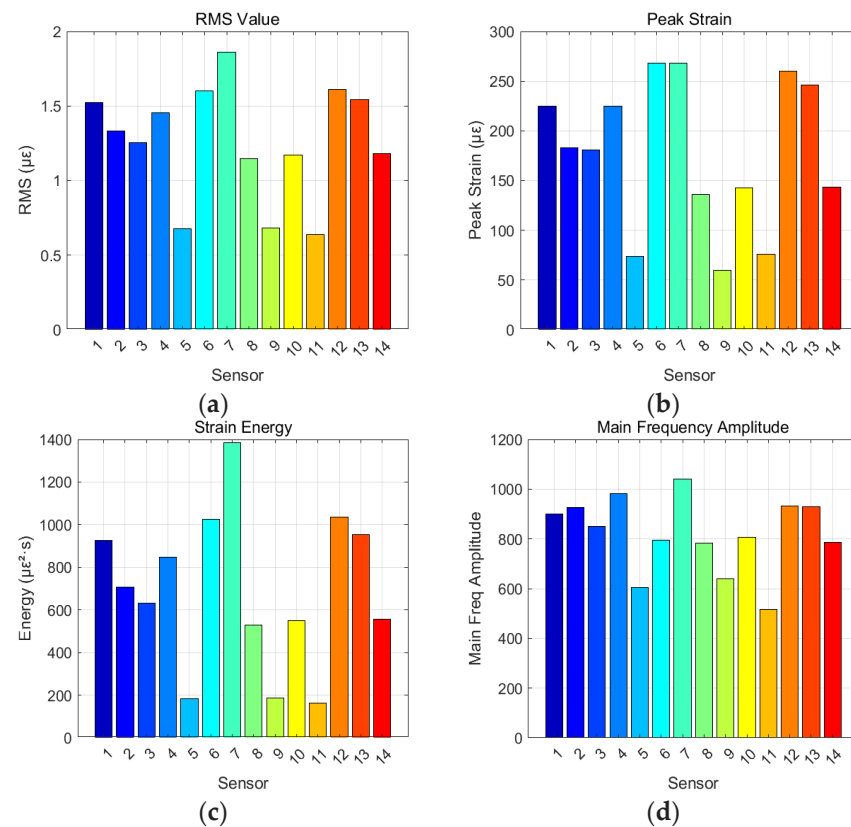
Figure 19. Dynamic-response characteristics of the measurement points: (a) RMS values, (b) peak strain values, (c) strain energy values, and (d) dominant frequency amplitudes.
