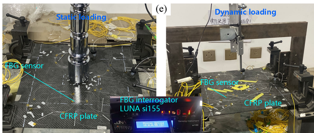
Figure 14. Experimental device of CFRP laminates: sensor layout on (a) top surface and (b) bottom surface under static loading; sensor layout on (c) top surface and (d) bottom surface; (e) practical testing models.
