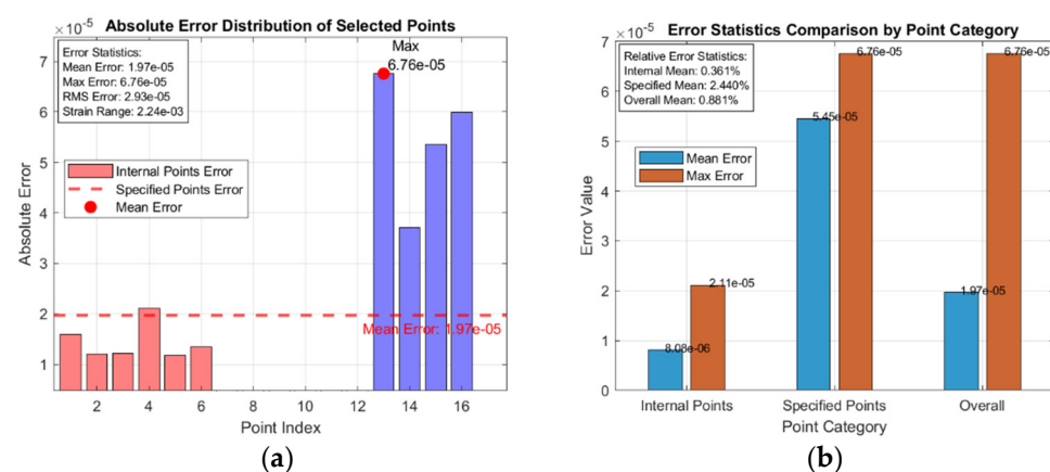
Figure 11. (a) Absolute error distribution of the optimal sensor placement scheme for the CFRP plate under static loading; (b) statistical comparison of strain reconstruction errors for the optimal sensor placement scheme under static loading.
