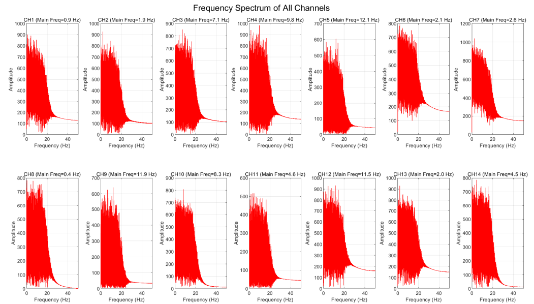
Figure 18. Frequency spectra of the strain responses at the 14 measurement points.
