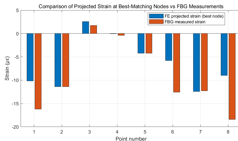
Figure 22. Comparison between measured and reconstructed strain data at the measurement.
