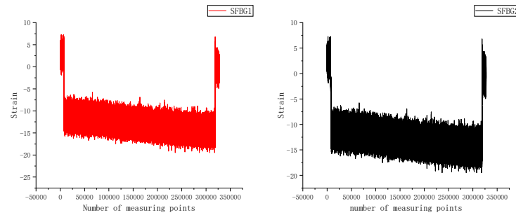
Figure 15. The strain time–history responses of two local measurement points.
