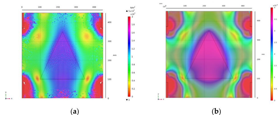
Figure 5. (a) Stress contour and (b) strain contour under dynamic loading.
