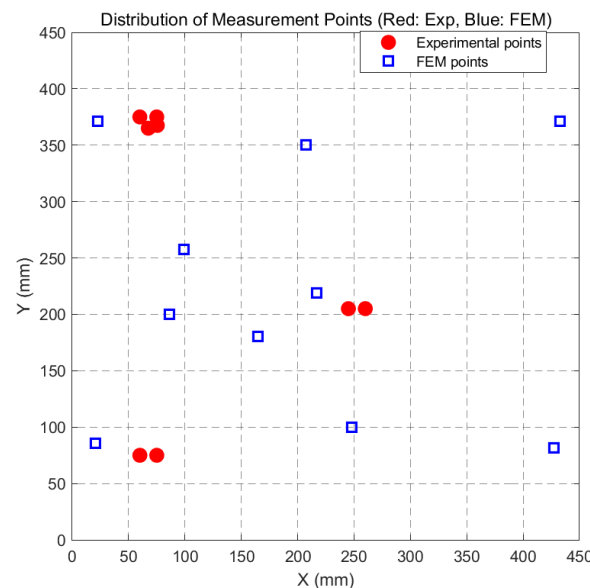
Figure 21. Comparison between the Finite Element and Experimental Measurement Point Layouts.
