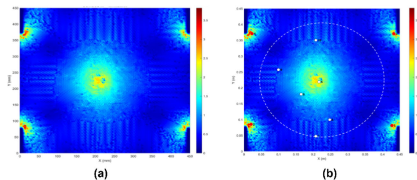
Figure 20. Static loading condition: (a) simulated strain contour; (b) optimal sensor placement scheme obtained from the finite element model.
