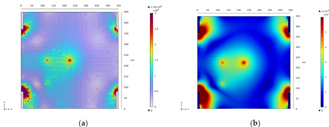
Figure 2. Finite element simulation results: (a) stress contour and (b) strain contour.
