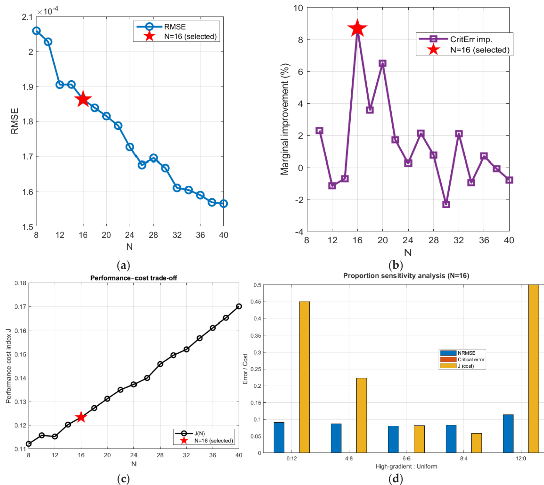
Figure 9. (a) Variation in global reconstruction root-mean-square error (RMSE) with the total number of sensors N (from 8 to 40, step size 2). (b) Marginal improvement rate of the critical-region error versus the total number of sensors N (improvement defined as the percentage reduction in critical-region MAE when adding two sensors). (c) Performance–cost index J(N) = \text{NRMSE}(N) + \lambda \cdot (N/N_{\max}) as a function of the number of sensors N , with \lambda = 0.1 and N_{\max} = 40 . (d) Reconstruction performance for different ratios of high-gradient to uniformly distributed interior points at a fixed total sensor number ( N = 16 ).
