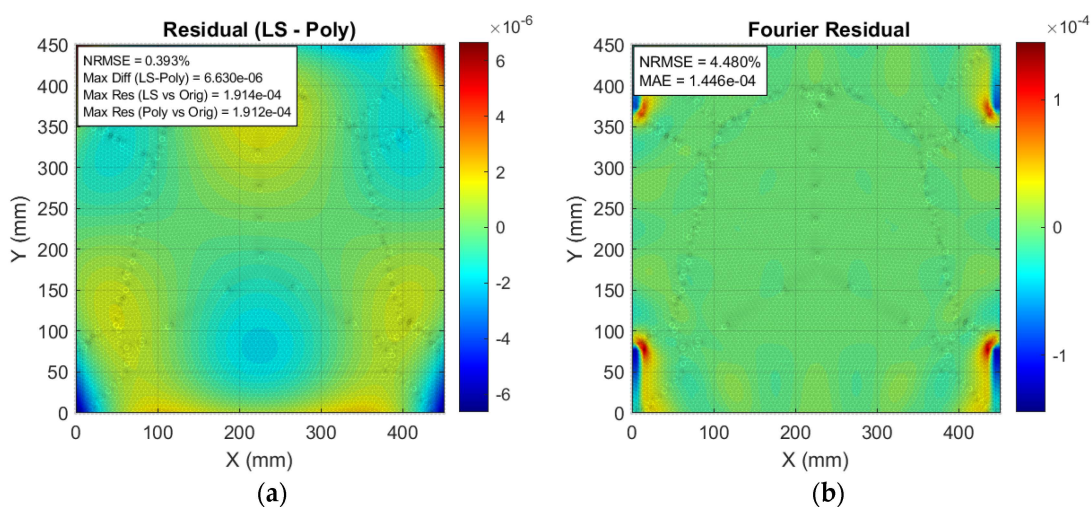
Figure 8. Residual strain maps under dynamic loading: (a) residual strain map of the polynomial and least-squares fitting methods relative to the original data; and (b) residual strain map of the Fourier series fitting method relative to the original data.
