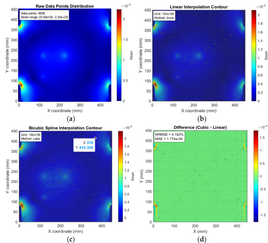
Figure 3. Strain field reconstruction under static loading based on 9696 data points: (a) original data points, (b) linear interpolation, (c) bicubic spline interpolation, and (d) difference between the two interpolation schemes.
