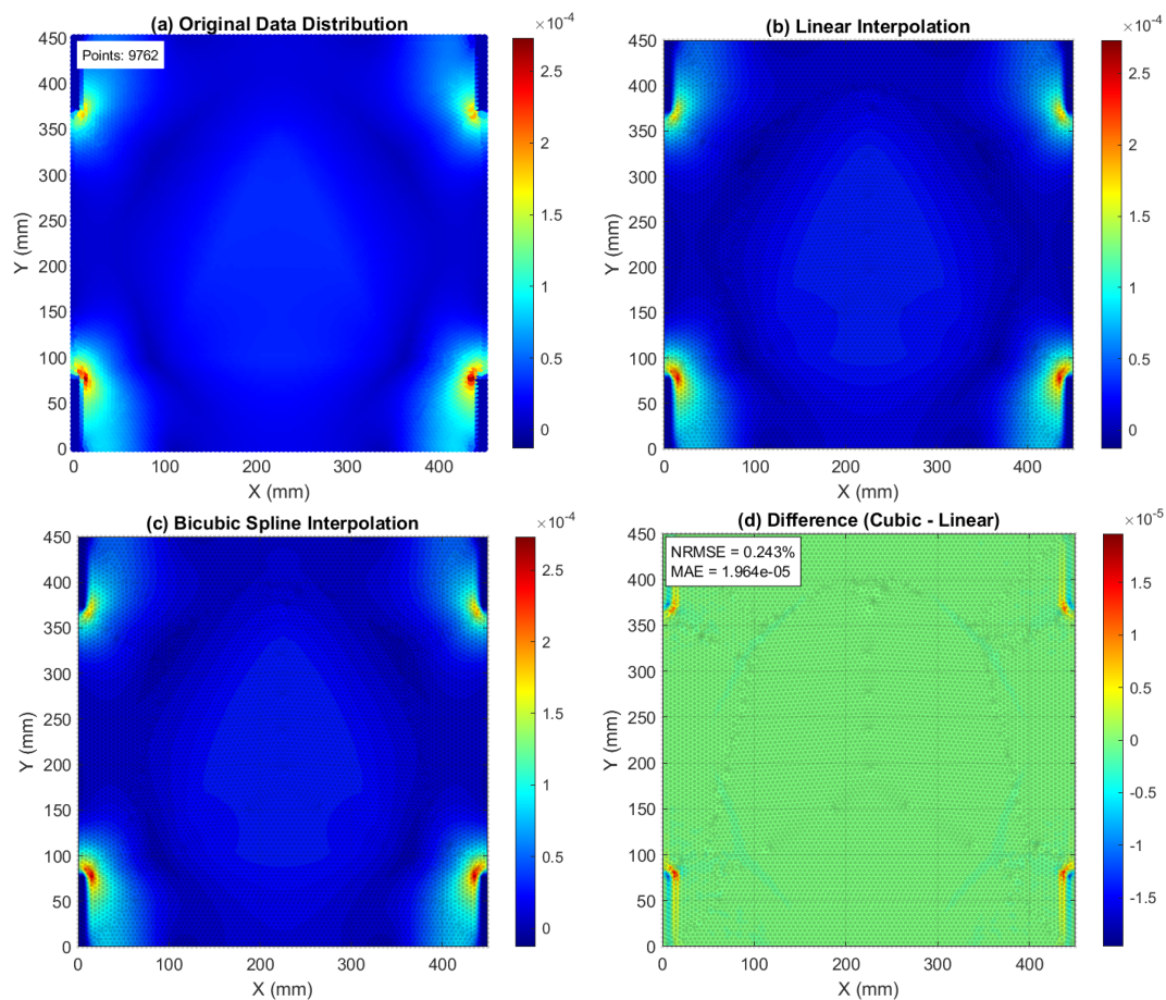
Figure 6. Results under dynamic loading: (a) original data distribution; (b) contour map obtained by linear interpolation; (c) contour map obtained by bicubic spline interpolation; and (d) difference between the two interpolation methods.
