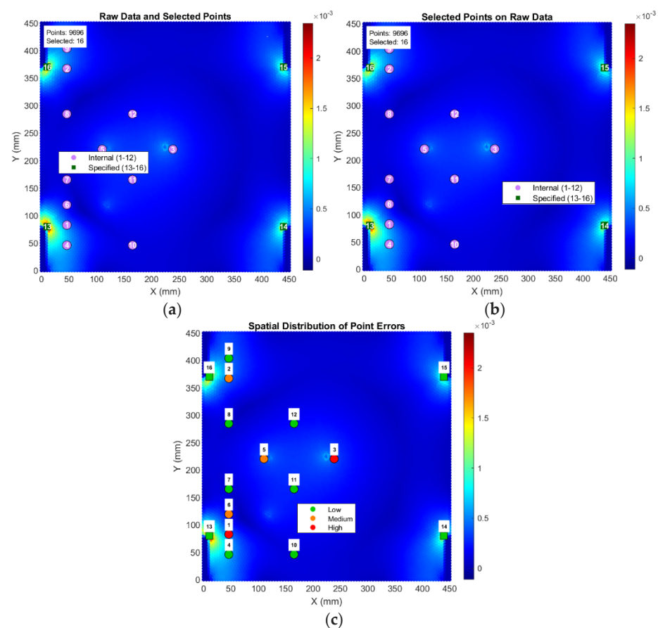
Figure 10. (a) Original data of the optimal CFRP plate layout under static load; (b) optimal CFRP plate layout scheme; (c) error analysis of the optimal CFRP plate layout scheme.
