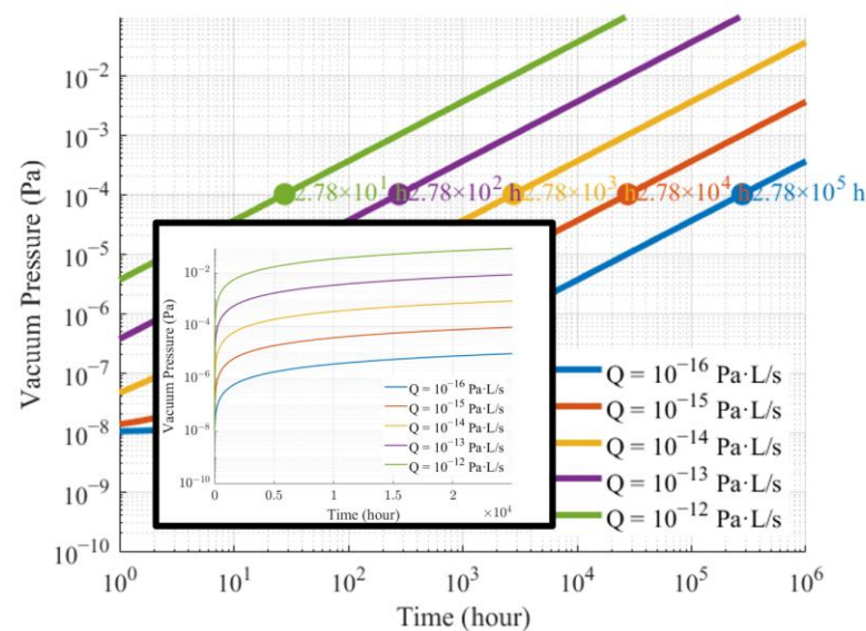
Figure 7. Vacuum level decay under different gas leak rates (log–log plot, initial vacuum level is 1 \times 10^{-8} Pa), the insert is a semi-log plot.
