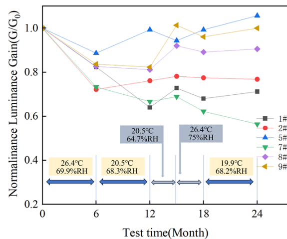
Figure 2. Normalized luminance gain of image intensifiers versus exposure time under humid and hot environments, together with the average temperature and humidity values corresponding to each storage stage (monitored every day by hygrothermograph).
