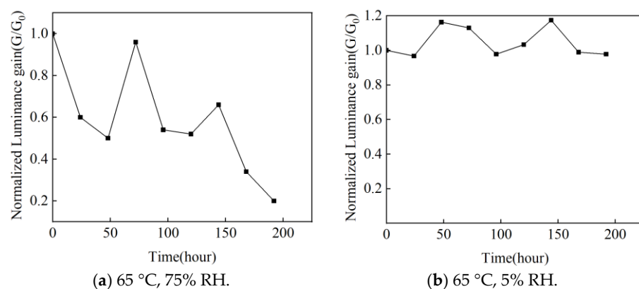
Figure 3. Decay curve of normalized luminance gain over time during high-temperature high-humidity/low-humidity aging test (data from a single sample, No. 220406).
