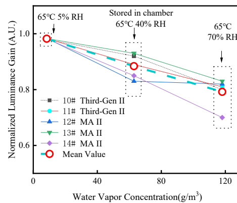
Figure 8. Relationship between the luminance degradation value of the image intensifiers screen and water vapor concentration.
