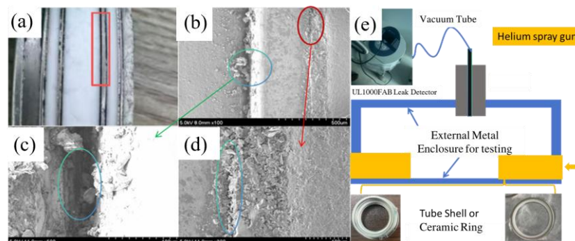
Figure 6. Physical and micro-morphology of the tube shell for sample 4# and gas leak rate detection. (a) Photograph of the tube shell; (b) low-magnification overall morphology of the sealing interface (scale bar: 500 μm); (c) local magnification of the interface edge (scale bar: 100 μm); (d) local magnification of the central region of the interface (scale bar: 100 μm); (e) schematic diagram of gas leak rate detection.
