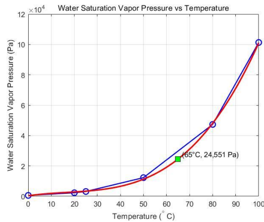
Figure 1. Fitted curve of water saturation vapor pressure as a function of temperature.
