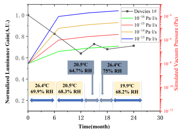
Figure 9. Luminance degradation of the image intensifier as a function of exposure time under natural humid and hot environments; the inset illustrates the variation trend of vacuum degree inside the image intensifiers after 12 months under different gas leak rates.
