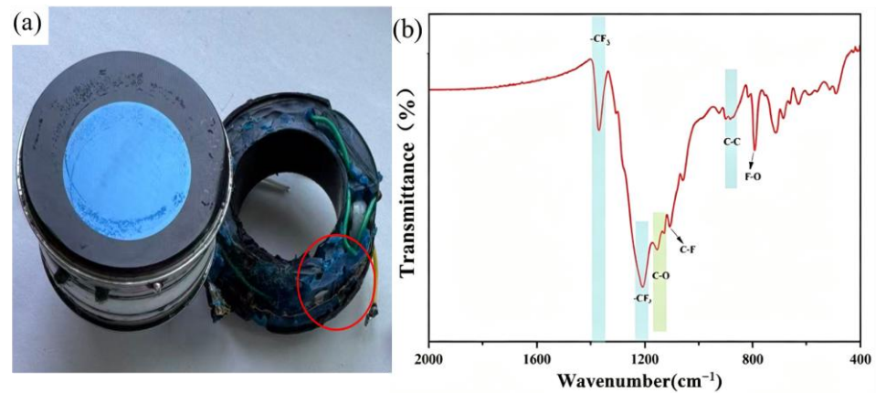
Figure 5. Attenuated total reflection (ATR) infrared spectroscopy test results of the circuit part and the green soft elastomer. (a) Morphology of the circuit part; (b) infrared spectroscopy result of the green elastomer.
