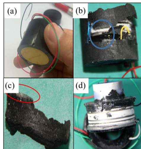
Figure 4. Photograph of image intensifier sample. (a) Intact sample with rigid outer housing; (b) device after removal of the rigid housing; (c) aging condition (red circle); (d) the power supply surface after removal of the sealing compound.
