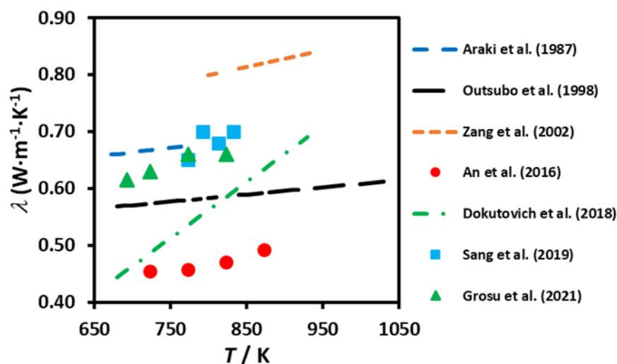
Figure 5. Thermal conductivity of the ternary eutectic (\text{LiNaK})_2\text{CO}_3 . Araki et al. (1987) [13]; Otsubo et al. (1998) [24]; Zhang et al. (2002) [25]; An et al. (2016) [12]; Dokutovich et al. (2018) [26]; Sang et al. (2019) [17]. The points from Grosu et al. (2021) [23] were estimated from the available plot. The lines are equations reported by the authors.
