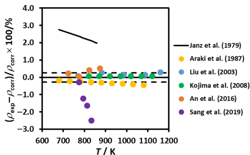
Figure 2. Deviation of different sets of data relative to the proposed correlation, Equation (1). Janz et al. (1979) [11]; Araki et al. (1987) [13]; Liu et al. (2003) [14]; Kojima et al. (2008) [15,16]; An et al. (2016) [12]; Sang et al. 2019 [17]. The dashed lines represent the estimated standard uncertainty of the correlation, 0.3%.
