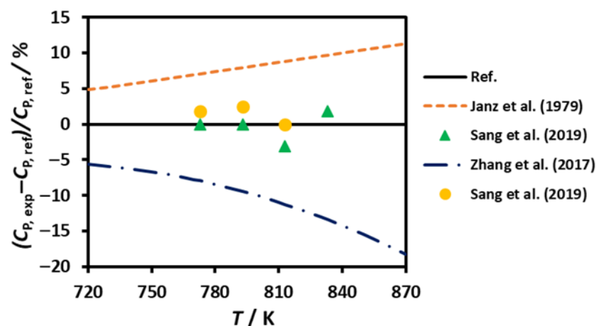
Figure 4. Deviation of different sets of data relative to the proposed reference value [12], Ref. Janz et al. (1979) [11]; Zhang et al. (2017) [22]; Sang et al. (2019) [17,18]. The lines are equations reported by the authors.
