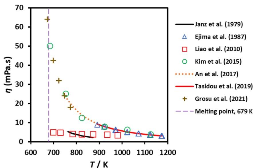
Figure 6. Viscosity of the ternary eutectic (\text{LiNaK})_2\text{CO}_3 . Janz et al. (1979) [11]; Ejima et al. (1987) [30,31]; Kim et al. (2015) [32]; An et al. (2017) [33]. The points from Liao et al. (2010) [21] and Grosu et al. (2021) [23] were estimated from the available plot. The lines are equations reported by the authors.
