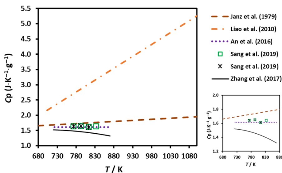
Figure 3. Heat capacity of the ternary eutectic (\text{LiNaK})_2\text{CO}_3 . Janz et al. (1979) [11]; An et al. (2016) [12]; Liao et al. (2010) [21]; Zhang et al. (2017) [22]; Sang et al. (2019) [17,18]. The lines are equations reported by the authors. The inset represents the data within a limited temperature range to enhance visibility.
