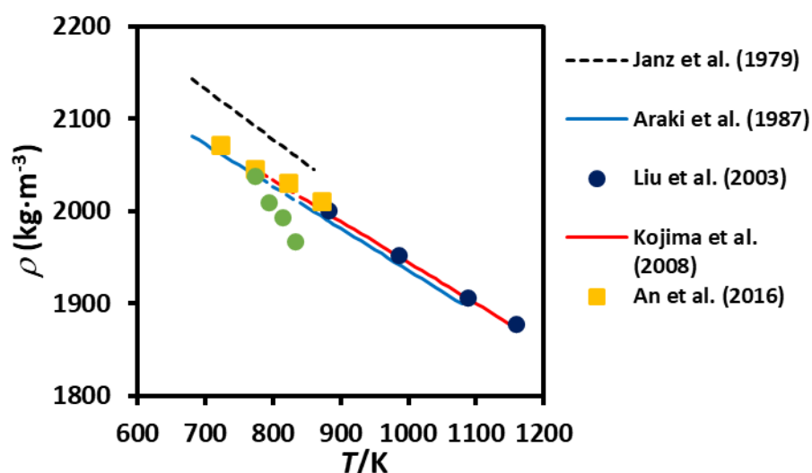
Figure 1. Density of the ternary eutectic (\text{LiNaK})_2\text{CO}_3 as a function of temperature. Janz et al. (1979) [11]; Araki et al. (1987) [13]; Liu et al. (2003) [14]; Kojima et al. (2008) [15,16]; An et al. (2016) [12]; Sang et al. 2019 [17]. The lines represent equations reported by the authors.
