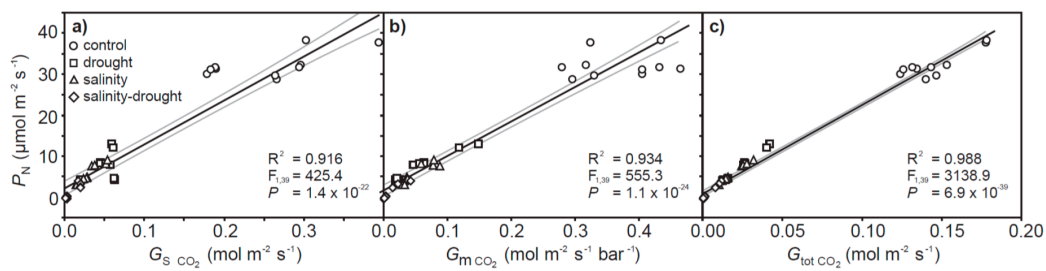
Figure 3. The relationship between photosynthesis with stomatal (a), mesophyll (b) and total (c) conductance to \text{CO}_2 . The black line indicates the line of best fit and the two grey lines either side indicate the 95% confidence intervals of the mean. Linear regression was used to assess the significance of any relationship.
