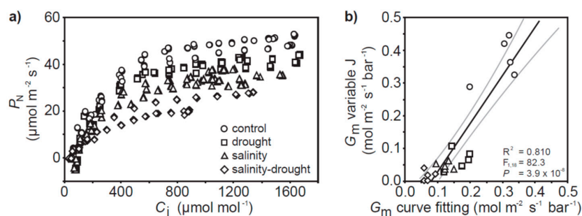
Figure 4. (a) P_{\text{N}}-C_i response curves of quinoa subject to the control, drought, salinity and salinity–drought treatments; (b) comparison of G_m values calculated using the variable J [32] and P_{\text{N}}-C_i curve fitting [31] methods. The black line indicates the line of best fit and the two grey lines either side indicate the 95% confidence intervals of the mean. Linear regression was used to assess the significance of any relationship.
