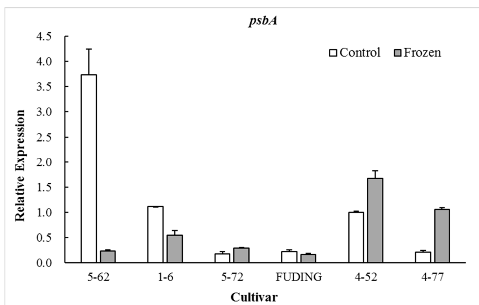
Figure 1. Effect of freezing on the expression of gene psbA .
