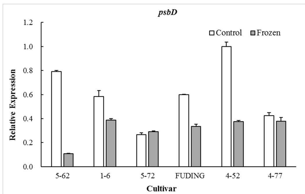
Figure 2. Effect of freezing on the expression of gene psbD .
