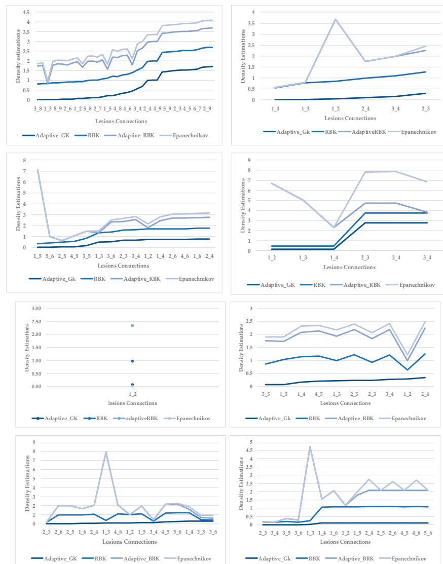
Figure 21. Probability density estimation according to the proposed adaptive Gaussian kernel, radial basis function kernel, adaptive radial bias function kernel, and Epanechnikov kernel methods.
