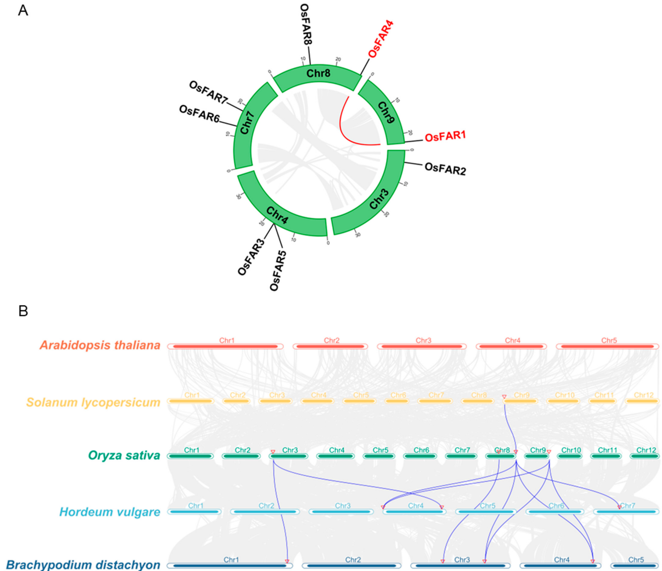
Figure 5. Chromosomal location, collinearity, and evolutionary analysis of OsFARs. (A) Distribution and collinearity of OsFARs in the rice genome. The collinearity of gene pairs is represented by gray and red lines. Scale bars marked on the chromosomes indicate chromosome lengths (Mb). (B) Interspecific collinearity analysis of FARs in rice, Arabidopsis thaliana , tomato, barley, and Brachypodium distachyon . The purple curves show the homology between FAR genes in rice and other species. The red triangles show gene locations.
