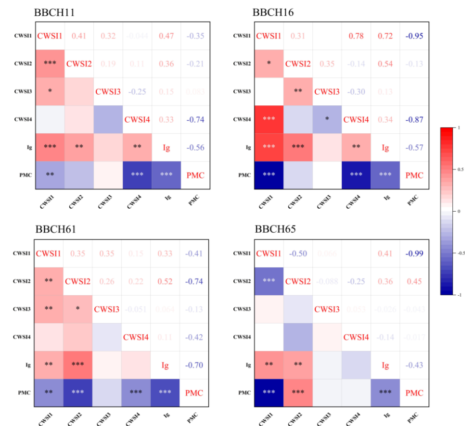
Figure 4. Relationships between PMC and temperature-related features in silage maize. Note: *, **, and *** denote significance at p < 0.05 , p < 0.01 , and p < 0.001 , respectively.
