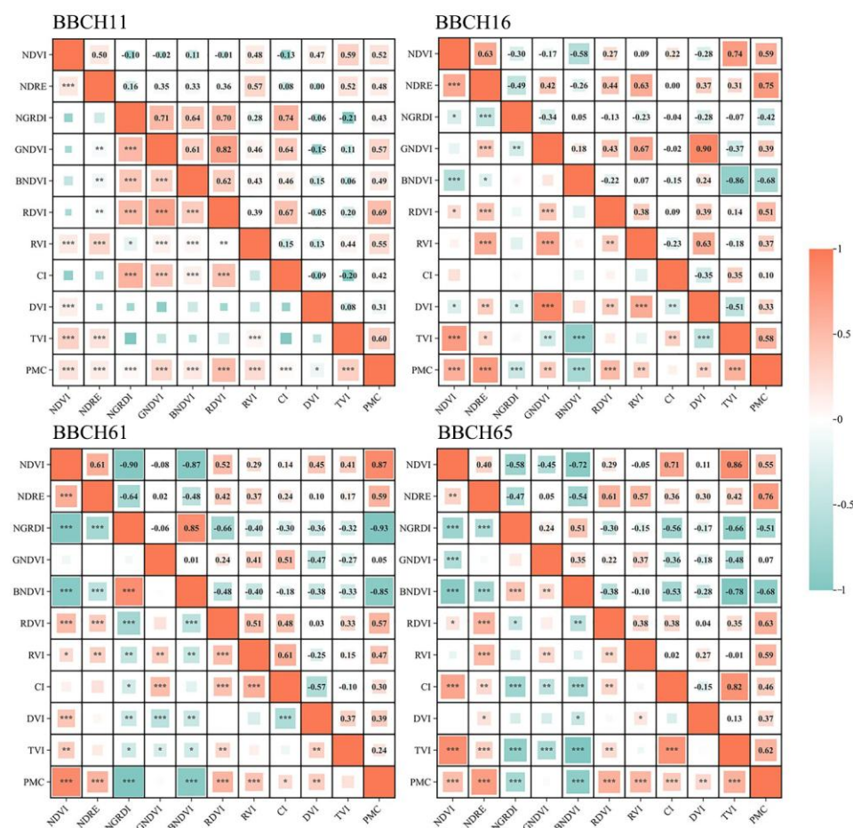
Figure 2. Relationships between PMC and vegetation indices in silage maize. Significance levels: *** p < 0.001 , ** p < 0.01 , * p < 0.05 .
