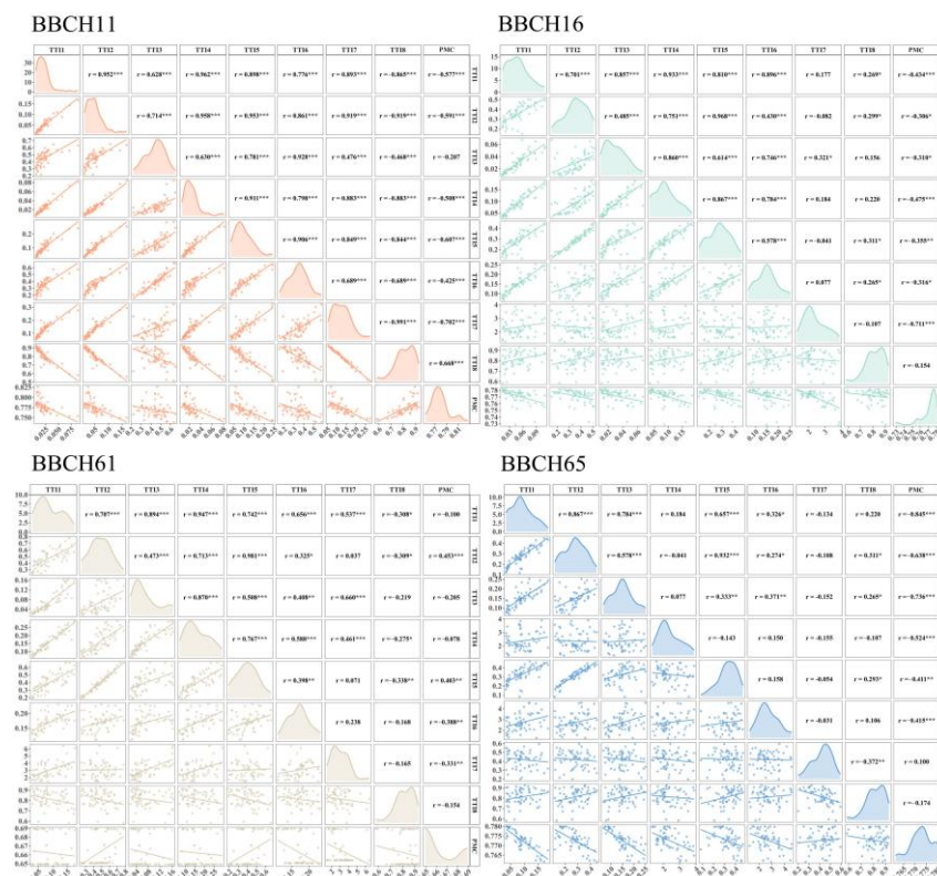
Figure 3. Relationships between PMC and texture features in silage maize. Significance levels: *** p < 0.001 , ** p < 0.01 , * p < 0.05 .
