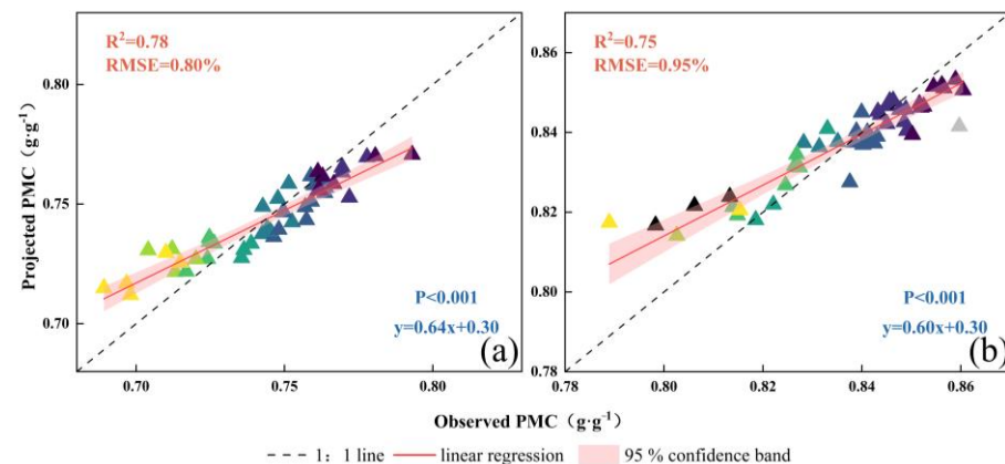
Figure 7. Validation of estimated plant moisture content against measured values in regions B (a) and C (b).
