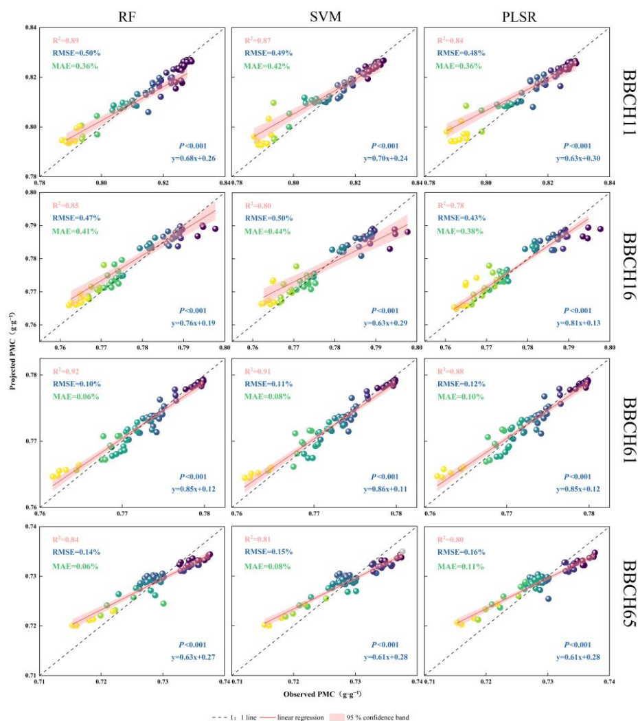
Figure 5. Performance of PMC models across different growth stages.
