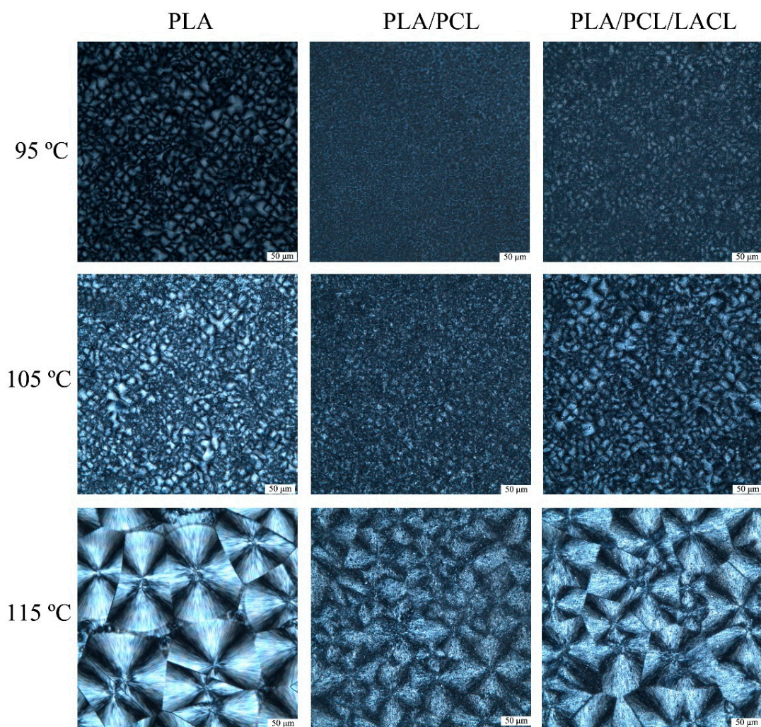
Figure 6. Polarized optical micrographs of PLA, PLA/PCL, and PLA/PCL/LACL spherulites isothermally melt crystallized at 95, 105, and 115 °C.
