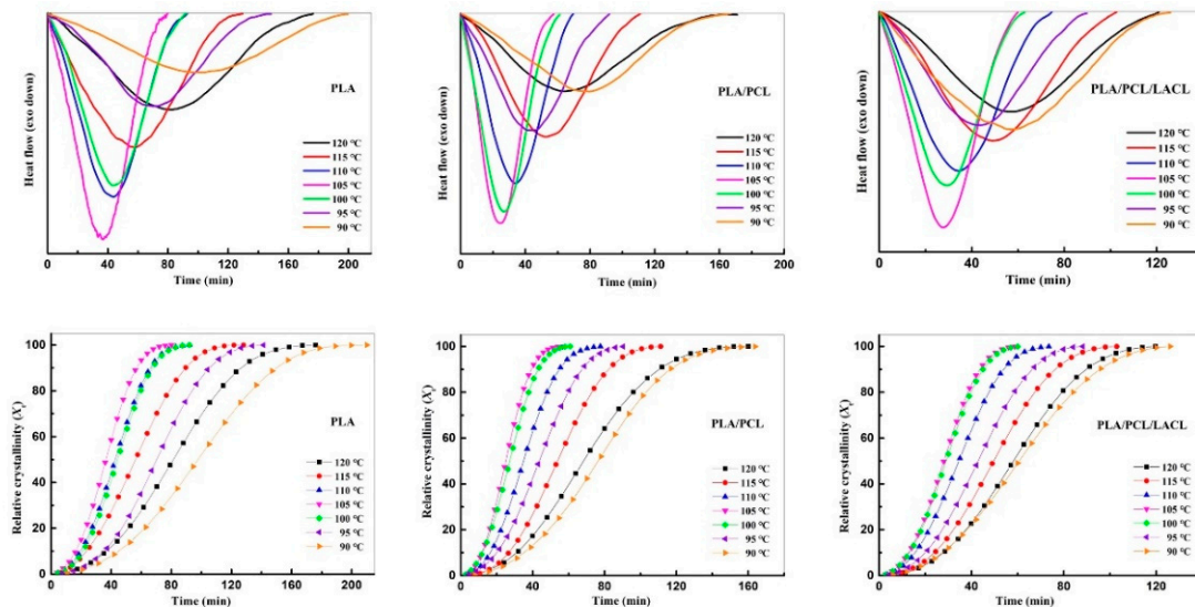
Figure 1. Heat flows and relative crystallinity as a function of time for PLA, PLA/PCL, and PLA/PCL/LACL isothermally melt crystallized at various temperatures characterized by differential scanning calorimeter (DSC).
