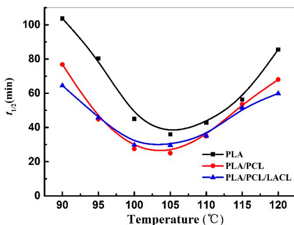
Figure 3. Crystallization half-time ( t_{1/2} ) of PLA, PLA/PCL, and PLA/PCL/LACL isothermally melt crystallized at various temperatures.
