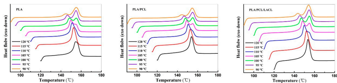
Figure 4. DSC heating scans of PLA, PLA/PCL, and PLA/PCL/LACL after isothermal crystallization at various temperatures.
