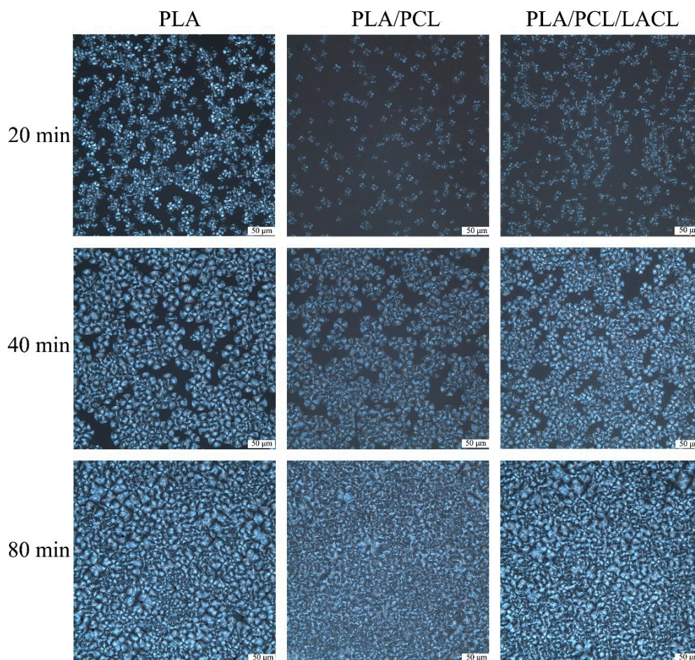
Figure 5. Polarized optical micrographs of PLA, PLA/PCL, and PLA/PCL/LACL spherulites isothermally melt crystallized at 105 °C for 20, 40, and 80 min.
