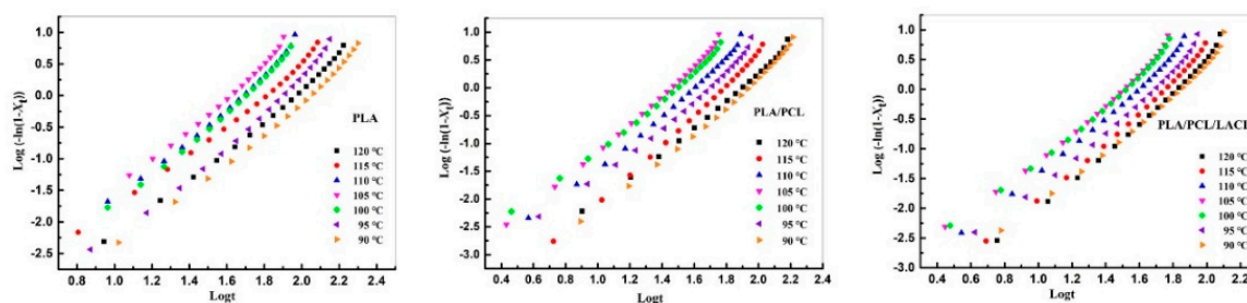
Figure 2. Avrami plots of PLA, PLA/PCL, and PLA/PCL/LACL isothermally melt crystallized at various temperatures.
